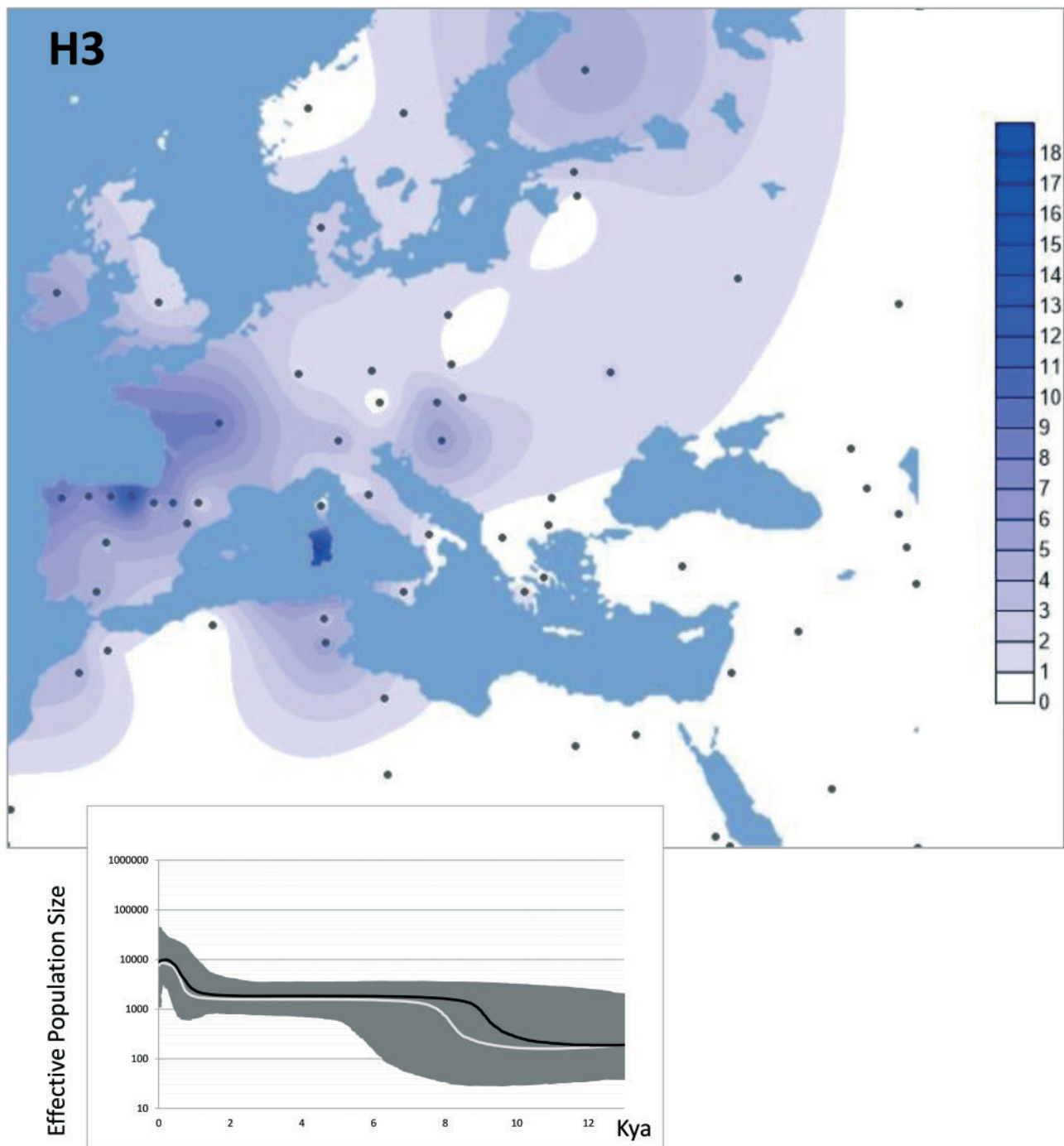
Fig. 4. Spatial frequency distribution map of haplogroup H3. Dots indicate the geographic locations of the surveyed populations. Population frequencies (%) are provided in supplementary table S9, Supplementary Material online. We constructed spatial frequency distribution plots with the program Surfer 9 (Golden Software, http://www.goldensoftware.com/products/surfer ). The inset shows the Bayesian skyline plot (BSP) showing effective population size trends of Sardinian H3 mtDNAs. The black and white lines are the median estimates obtained by employing the mutation rates proposed by Soares et al. (2009) and Posth et al. (2016) , respectively; the grey shading shows the highest posterior density limits.
