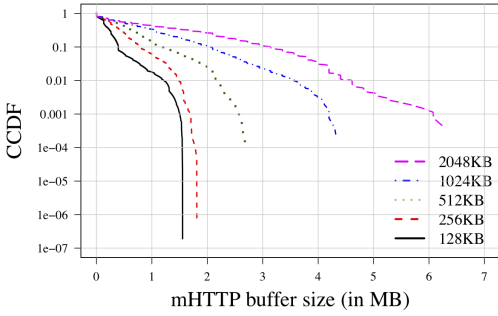
(a) mHTTP buffer size with scheduling.
