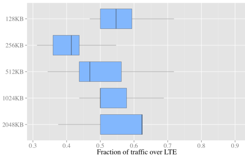
Figure 12: Scenario 1 (outdoor testbed): fraction of traffic carried over a LTE connection for file size of 16MB.
