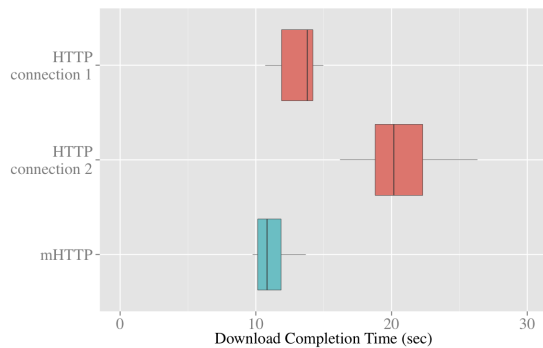
(b) Download completion time
