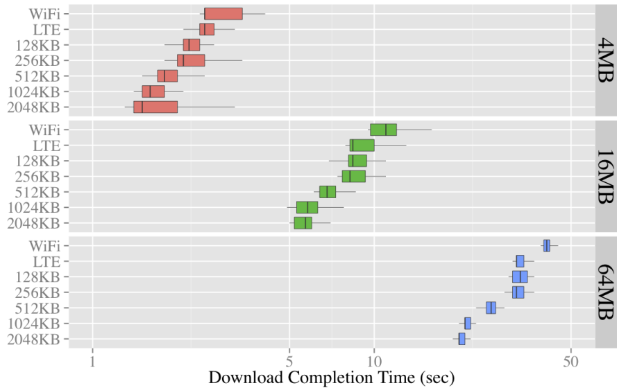
Figure 10: Scenario 1 (outdoor testbed): download completion time of regular HTTP vs. mHTTP for different file and chunk sizes. mHTTP can efficiently take advantage of the diversity exists in the network. We observe that mHTTP shows a relatively low performance when using small chunk sizes compared to the measurements with large chunk sizes which is due to the fact that our server configuration is not optimized for mHTTP.
