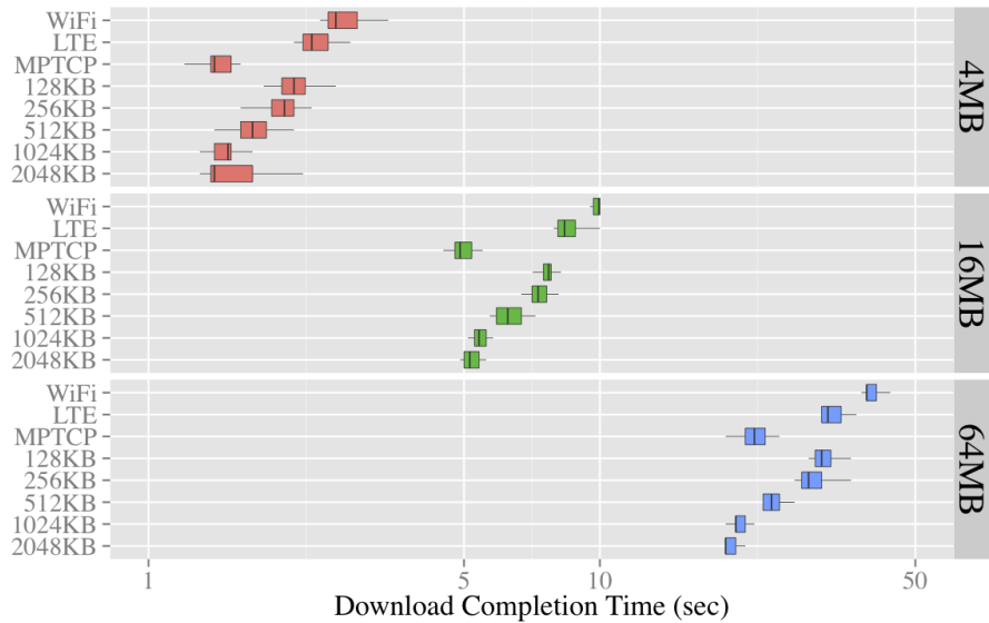
Figure 15: Scenario 2 (outdoor testbed): download completion time of mHTTP vs. MPTCP and regular HTTP. We observe that MPTCP is able to fully use the available bandwidth and mHTTP performs close to MPTCP.
