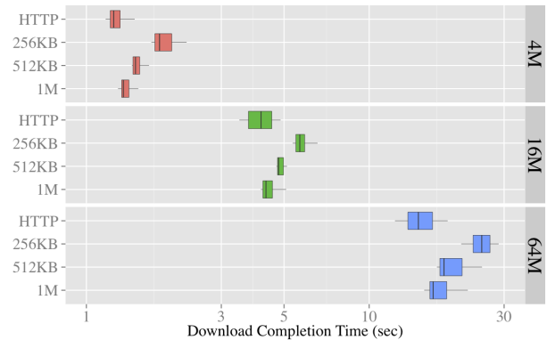
Figure 7: Overhead analysis: HTTP vs. mHTTP over a single connection.
