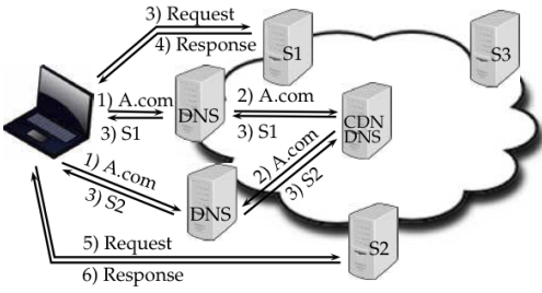
Figure 2: An mHTTP, with two connections over two available interfaces, operation in a CDN. Servers S1, S2, and S3 host replicas of content of A.com.
