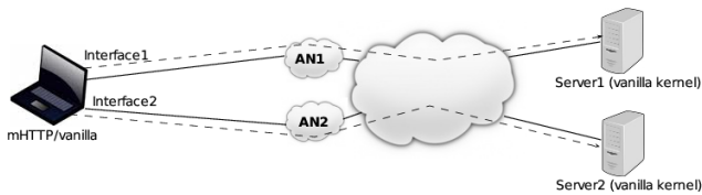
Figure 6: Scenario 1: 2 interfaces at the client; 2 servers; 2 paths (dashed lines). In our indoor testbed, AN1 and AN2 are Ethernet routers with a nominal rate of 100Mbps. In our outdoor testbed, the client is a mobile device (laptop) with one WiFi and one LTE interface.
