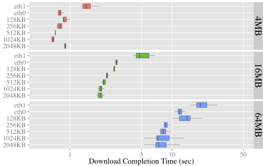
Figure 9: Scenario 1 (indoor testbed): download completion time of regular HTTP vs. mHTTP for different file and chunk sizes. mHTTP can efficiently use the bandwidth available to the client and outperforms the best performing connection among regular HTTP connections. 1024KB of the chunk shows the optimal performance in all file sizes.
