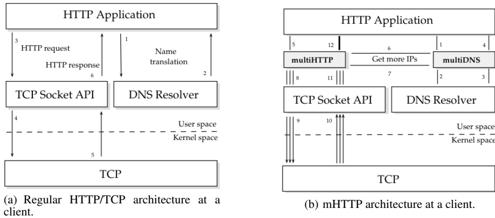
Figure 1: Structural differences between HTTP/TCP and mHTTP
