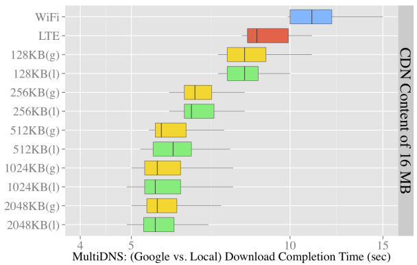
Figure 17: Measurement on a CDN infrastructure. The results are shown for two cases: the first case uses IP addresses obtained from DNS queries sent to Google DNS (shown with (g) in the y-axis); and the second case that uses IP addresses obtained from the local DNS of each of the interfaces networks (shown with (l) in the y-axis).
