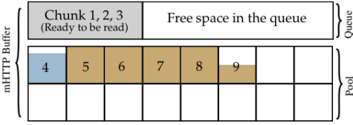
Figure 5: A bottleneck in mHTTP buffer. Chunk 4 is downloaded over a slow connection. Chunks 5, 6, 7, 8 are downloaded over a fast connection. These chunks cannot proceed to the queue before chunk 4 is completely received. A scheduler is needed to better allocate chunks across different connections.
