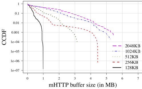
(b) mHTTP buffer size without scheduling.
