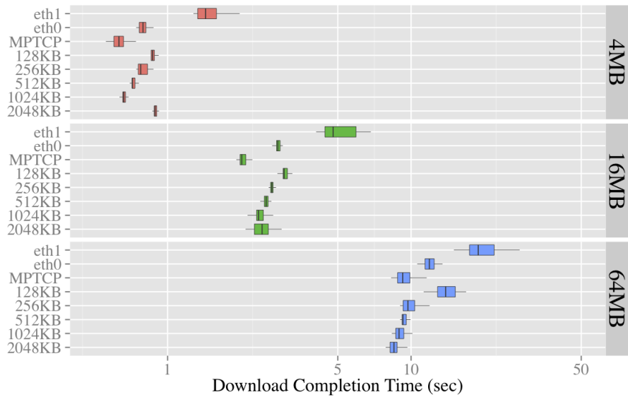
Figure 14: Scenario 2 (indoor testbed): download completion time of mHTTP vs. MPTCP and regular HTTP. Our testbed configuration is optimized for MPTCP. Hence, MPTCP is able to fully utilize the available capacity and provide a good performance. We observe that mHTTP perform very close to MPTCP and always outperforms regular HTTP over the best path.
