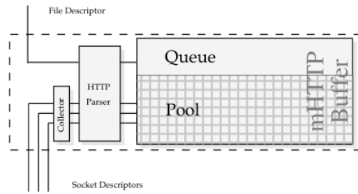
Figure 4: multiHTTP design: a) mHTTP buffer stores out-of-order received data b) HTTP parser examines and modifies HTTP headers c) collector gathers data from individual TCP connection buffers.
