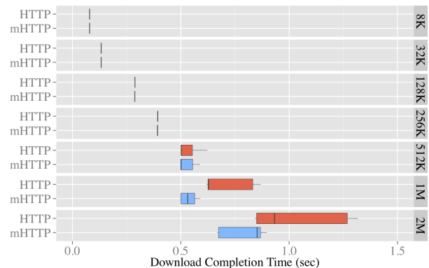
Figure 8: The performance of downloading small objects in Scenario 1 (mHTTP chunk size: 512KB).
