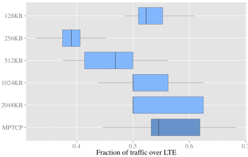
Figure 16: Scenario 2 (outdoor testbed): fraction of traffic carried over a LTE connection for 16MB file using mHTTP as well as MPTCP. We show the results for 16MB file.
