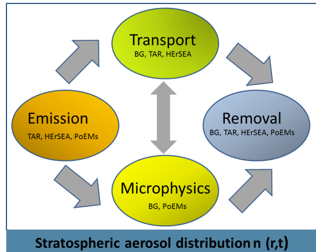
Figure 2. Schematic overview over the processes that influence the stratospheric aerosol size distribution. The related SSiRC experiments are listed below. BG stands for Background, TAR for Transient Aerosol Record, HErSEA for Historical Eruption SO 2 Emission Assessment, and PoEMs for Pinatubo Emulation in Multiple models.
