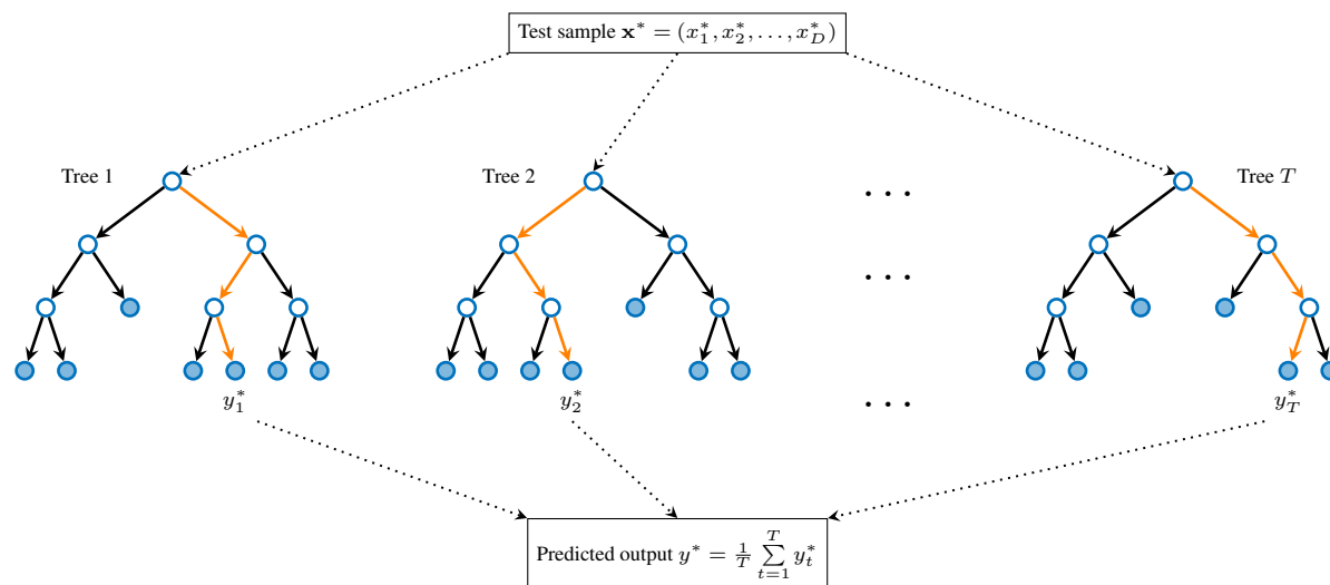
Figure 2. Predicting the output y^* of a sample \mathbf{x}^* with a randomized decision forest is carried out by averaging the individual predictions obtained from the T decision trees in the ensemble.
