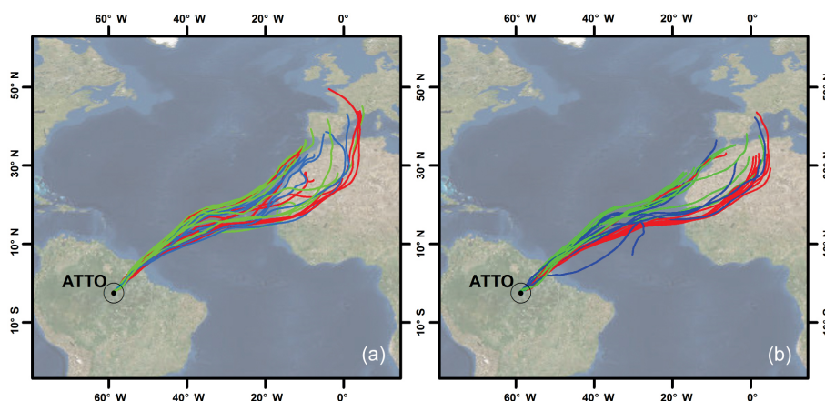
Figure 1. Backward trajectories of air parcels above the Amazon for 240 h during the sampling periods for (a) 5 April 2015 and (b) 6 April 2015, when the greatest concentrations of dust from the Sahara arrived at ATTO.
