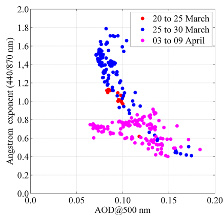
Figure 3. Ångström exponent (AE) calculated using aerosol optical depth (AOD) from 440 and 870 nm as a function of AOD at 500 nm (AOD at 500 nm) using data from AERONET sun photometers installed in Ilorin ( 08^{\circ}19'12'' N, 04^{\circ}20'24'' E – left plot) and upwind of Manaus in central Amazonia ( 02^{\circ}53'12'' S, 59^{\circ}58'12'' W – right plot) during distinct phases of the sampling period (20 March to 17 April).
