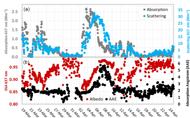
Figure 4. (a) Particle absorption and scattering coefficients at 637 nm observed in situ at the ATTO site. (b) Particle single scattering albedo (SSA) at 637 nm, and absorption Ångström exponent (AAE), retrieved from in situ observations of aerosol optical properties at ATTO.
