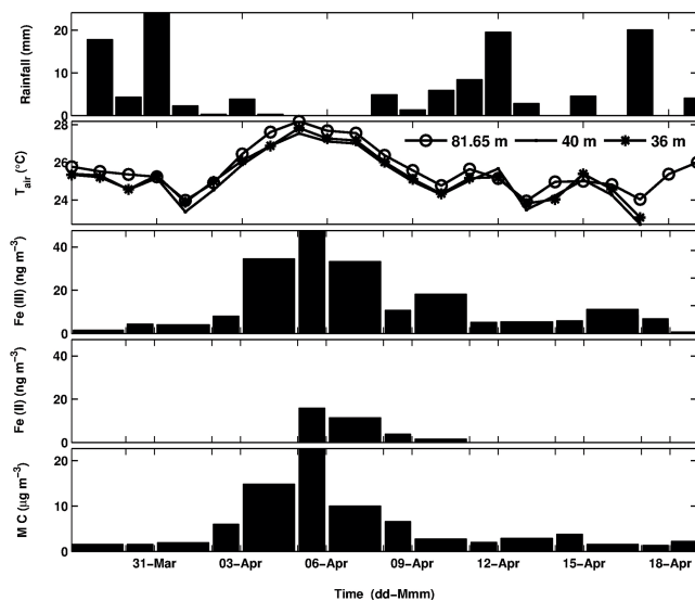
Figure 6. Daily comparison of micrometeorological variables: average air temperature and accumulated precipitation ( T_{\text{air}} , rainfall) with measurements of soluble Fe(III) and Fe(II) and mass concentration (MC) above the canopy.
