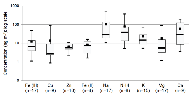
Figure 7. Box plot for the soluble ion and other species concentrations in the total particulate matter samples at 60 m height from 30 March to 25 April 2015. Upper and lower whiskers represent 1.5 interquartile ranges for the period; upper and lower boundaries are for the third and first quartile. The horizontal bar is the median value and the black square is the average value for each element. In the horizontal axis, the number of samples with valid results is shown.
