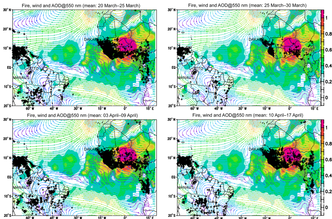
Figure 5. Mean aerosol optical depth at 550 nm (AOD, shaded color) and wind at 850 hPa (stream lines) and total fire spots (black plus symbol) for four distinct periods within the campaign at ATTO site, during the dominance of (a) the first Saharan dust outbreak; (b) a less active dust outbreak period; (c) the second Saharan dust outbreak; (d) the third Saharan dust outbreak.
