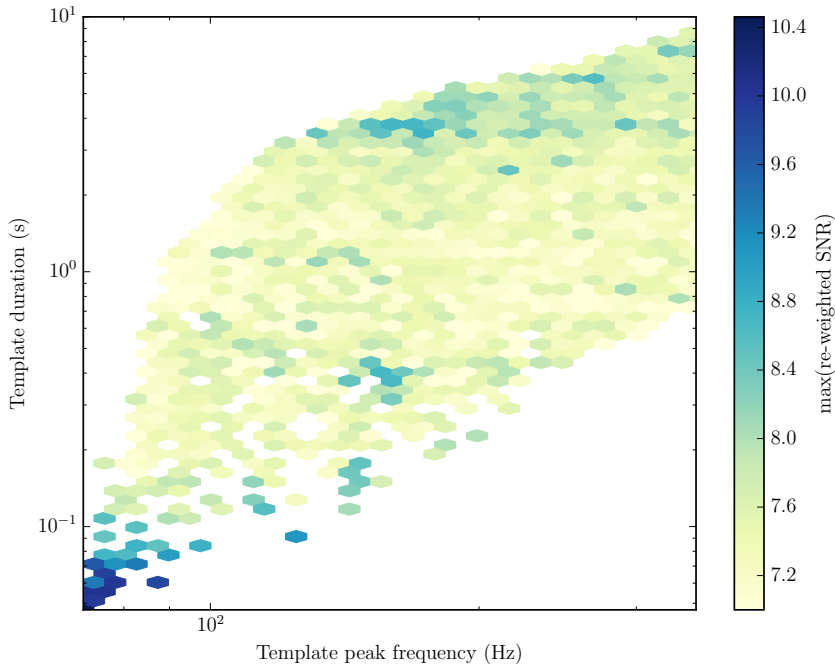
Figure 15: A plot of single detector triggers from the Livingston detector binned by template duration and waveform template peak frequency. The loudest triggers in re-weighted SNR are constrained to the area of the parameter space with template durations < 0.1 s, which is the timescale of typical instrumental transients, most notably blip transients. The small cluster of loud triggers with a template duration of roughly 4.4 s corresponds to the 60-200 Hz noise discussed in Section 8.3.
