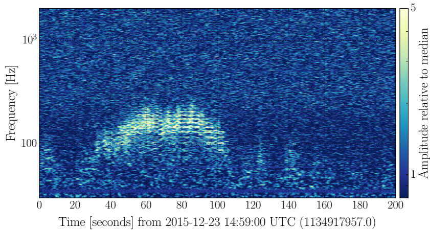
Figure 17: A zoomed in time-frequency spectrogram of the 60-200 Hz noise. This period of noise caused a loud trigger in the PyCBC background. The arc-like shape of the noise is reminiscent of noise due to scattered light, but the frequency of the noise is higher than expected.
