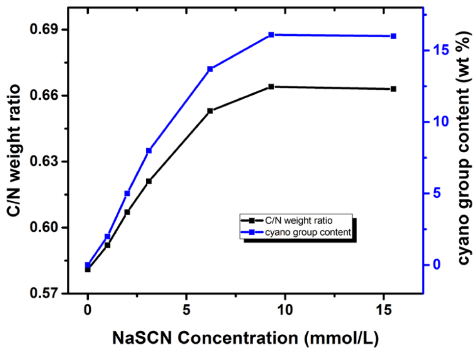
Figure S4 element analysis of the g\text{-C}_3\text{N}_4\text{-xCN} samples.
