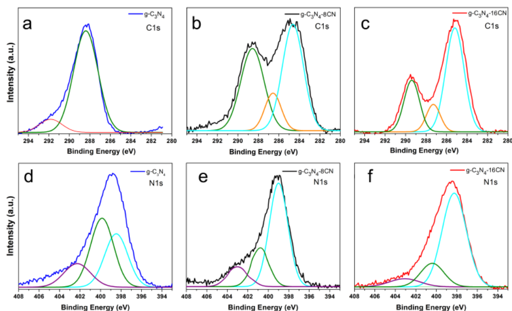
Figure 2. C 1s (a, b, c), N 1s (d, e, f) X-ray photoelectron spectroscopy (XPS) curves of g\text{-C}_3\text{N}_4 (blue), g\text{-C}_3\text{N}_4\text{-8CN} (black), g\text{-C}_3\text{N}_4\text{-16CN} (red).
