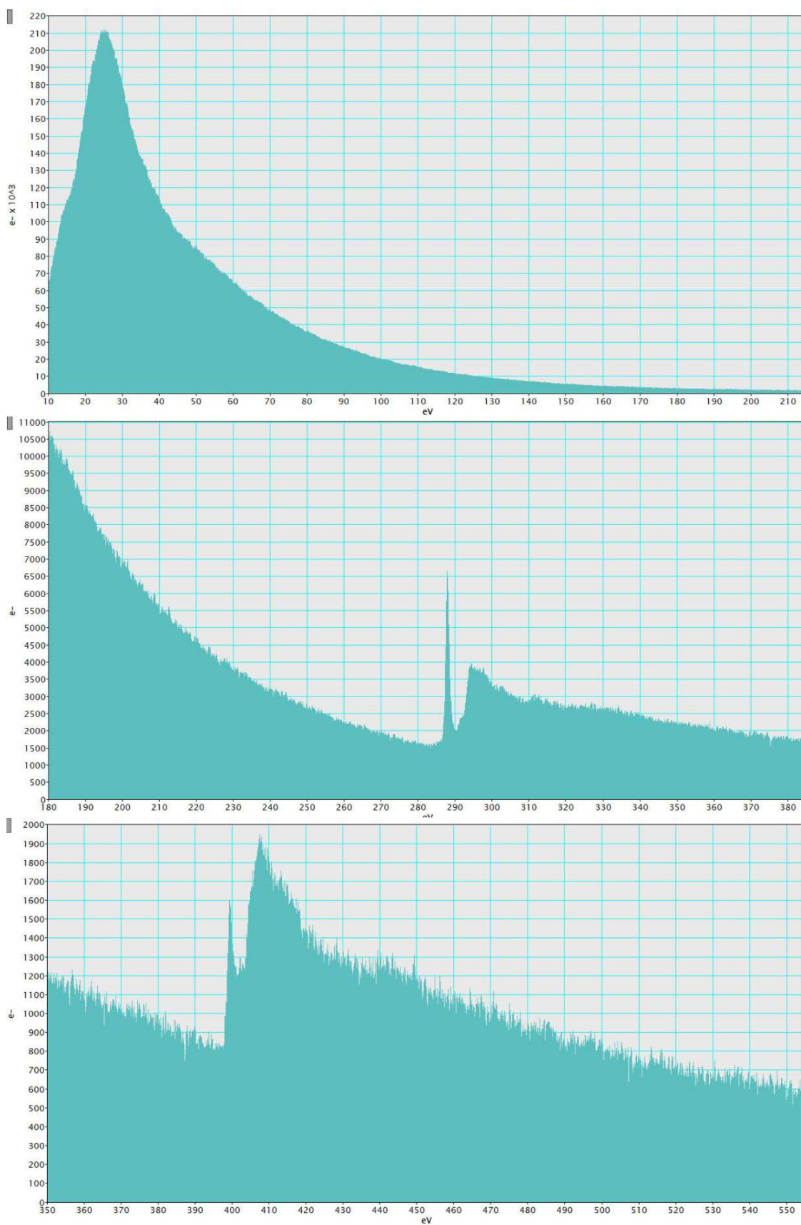
Figure S2. Electron Energy Loss Spectroscopy analysis of g-C 3 N 4 -16CN. Only the signals of C (284eV) and N (401eV) could be found.
