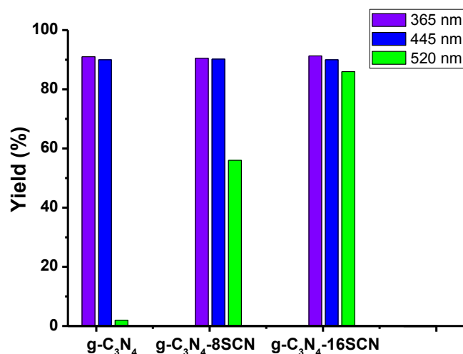
Figure 4. Photocatalytic performance of the pristine g-C 3 N 4 and g-C 3 N 4 -16SCN in the coupling reaction between styrene and sodium benzenesulfinate under UV (365 nm), blue (445 nm), green (520 nm), light and irradiation. Reaction conditions: 0.17 mmol of styrene 0.5 mmol of sodium benzenesulfinate and 0.34 mmol nitrobenzene were mixed with 5 mL ethanol in a glass vial. 25 mg of the photocatalyst were added in the reaction mixture as well. The glass reactor was then irradiated by different LED for 24 hours. The yield of the reaction was determined by GC-MS/FID.
