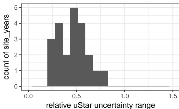
Figure C3. Histogram of ratio ( REddyProc / DP06 ) of uncertainty ranges of uStar (90% quantile - 10% quantile). The clustering around 0.5 shows that the estimated uncertainty with REddyProc is only about half the uncertainty estimated by DP06 .
