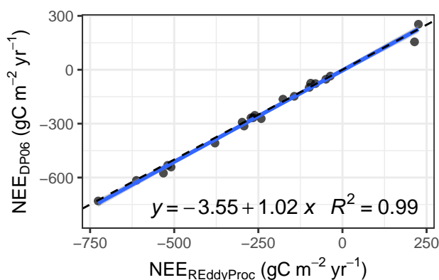
Figure 5. Strong correspondence in NEE based on uStar estimated by REddyProc and NEE based on uStar estimated by DP06 across site-years.
