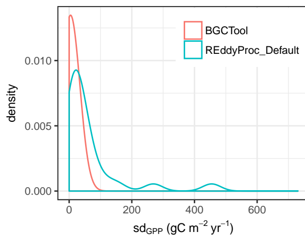
Figure C5. Density plot of estimated standard deviation of uncertainty of the annually aggregated GPP across sites due to uncertainty in parameters estimation during day-time based flux partitioning. Higher estimates with REddyProc are caused by taking into account the uncertainty in temperature sensitivity, E_0 .
