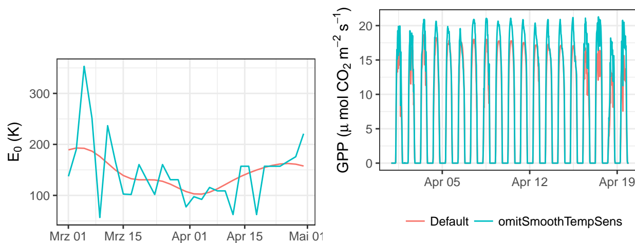
Figure C6. Effects of smoothing (top) successive estimates of temperature sensitivity, E_0 , on predicted GPP (bottom) for site PT-Esp.
