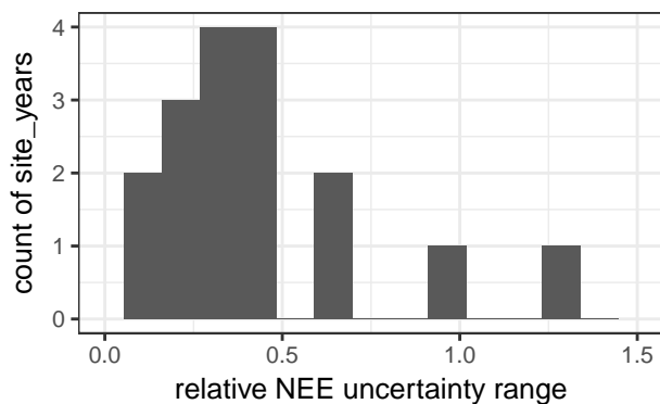
Figure C4. Histogram of ratio ( REddyProc / DP06 ) of uncertainty ranges of annual NEE (NEE based on 90% quantile of uStar threshold - NEE based on 10% quantile of uStar threshold). The clustering below a value of one indicates that the lower uncertainty in uStar threshold with REddyProc also propagates to lower uncertainty in annual NEE.
