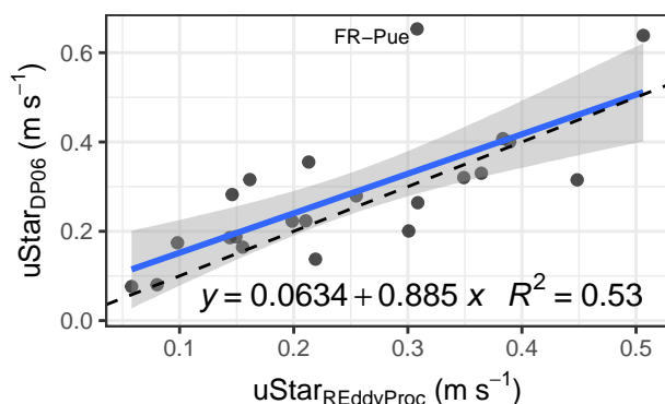
Figure 4. Large scatter but retained relationship between uStar derived with DP06 versus uStar derived with REddyProc across site-years as shown by a regression (solid line with shaded uncertainty bound) close to the 1:1 line (dashed).
