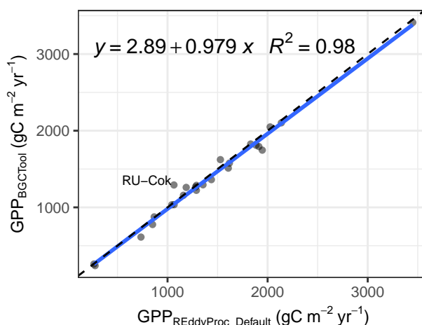
Figure 8. Prediction of annually aggregated GPP from REddyProc daytime partitioning agree with the BGC online tool across sites.
