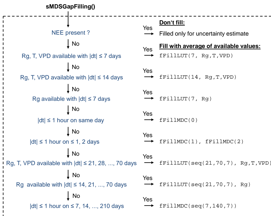
Figure 3. Flow diagram of the MDS gap-filling algorithm as implemented in REdDyProc. See table 1 for abbreviations.
