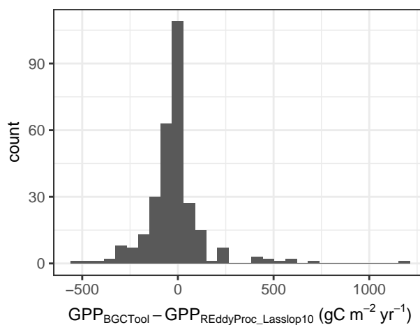
Figure C8. Histogram of difference between monthly GPP predictions of REddyProc with Lasslop10 compatibility options and the BGC online tool.
