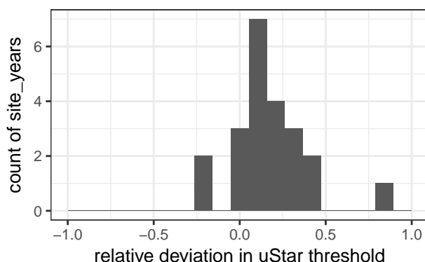
Figure C1. Histogram of differences between uStar threshold estimates of different methods (DP06 - REddyProc) normalized by the uncertainty range (90% quantile - 10% quantile estimated by DP06). Absolute values are smaller than one meaning that the difference between the methods is smaller than range of estimates by the DP06 method only. The clustering of values on the positive side suggests a bias towards larger values with DP06.
