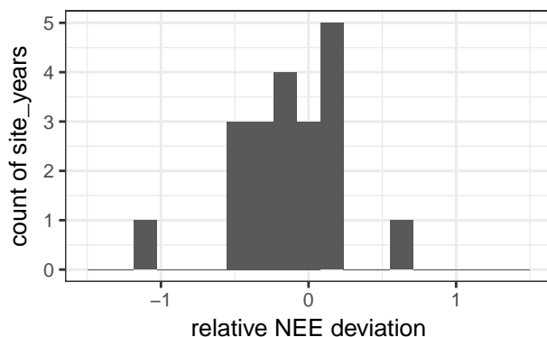
Figure C2. Histogram of differences between annual NEE based on uStar estimates of different methods (Papale - REddyProc) normalized by the uncertainty range of NEE due to uStar (NEE based on 90% uStar quantile - NEE based on 10% uStar quantile estimated by DP06). Absolute values are mostly smaller than one, meaning that the difference in annual NEE between methods is smaller than the uncertainty due to uncertainty of uStar threshold from DP06 only.
