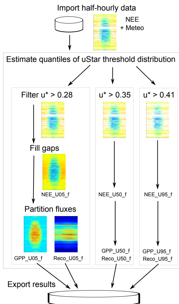
Figure 1. The workflow starts with importing the half-hourly (or hourly) data, here the year 1998 of site DE-Tha is plotted as an example. Next, a probability distribution of u^* threshold is estimated for each season. Gap-filling and flux-partitioning is performed for several quantiles of this distribution for an estimate of uncertainty. Finally the results are exported.
