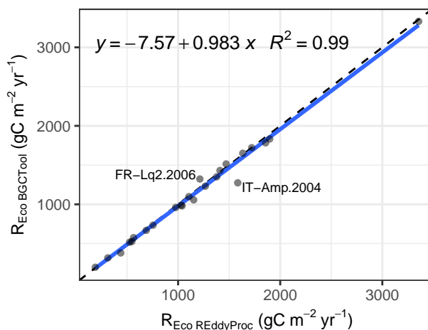
Figure 7. Predictions of annually aggregated ecosystem respiration, R_{eco} from REddyProc night-time partitioning agree with the predictions by the BGC online tool.
