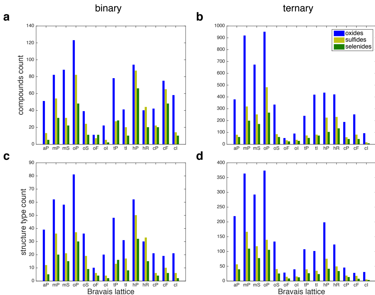
FIG. 11. Number of compounds ( a and b ) and structure types ( c and d ) for each Bravais lattice. Binaries are on the left ( a and c ) and ternaries on the right ( b and d ). Oxides are shown in blue, sulfides in light green and selenides in darker green. All six distributions (binary and ternary oxides, sulfides and selenides) are double peaked with a local minimum for the orthorhombic face and body centered lattices. The high symmetry cubic lattices are also relatively rare. This reflects the complex spatial arrangement of the compound forming electrons of the 6A elements, which does not favor the high symmetry of these structures.
