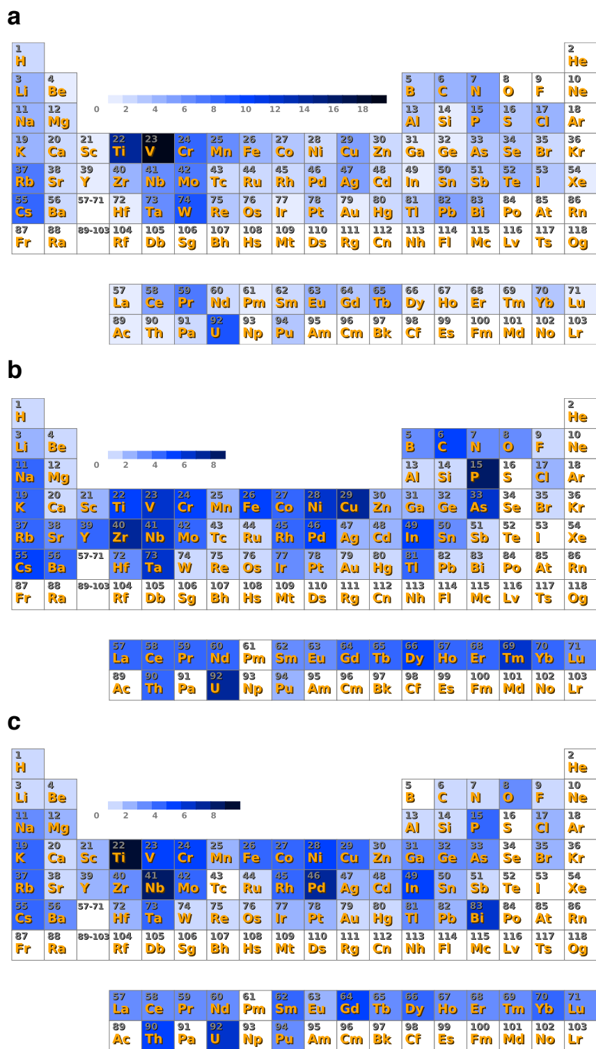
FIG. 3. Binary (a) oxide, (b) sulfide, and (c) selenide stoichiometries (number of different stoichiometries that include the respective element). The colors go from no stoichiometries (white) to the maximal number of stoichiometries (dark blue) which is different for each element, 19/8/9 for O/S/Se. Islands of high prevalence appear for the 4B and 5B transition metals and the heavy alkalis in all three compound families. Additional, smaller islands appear in the sulfides and selenides for the 8 and 1B transition metals and the 3A and 5A semi-metals.
