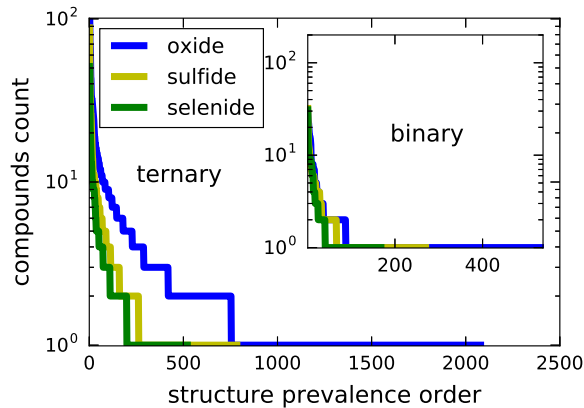
FIG. 1. Distributions of the compounds among structure types for binary (inset) and ternary compounds. Oxides are shown in blue, sulfides in yellow and selenides in green. The binary distributions differ mostly by the length of their single-compound prototypes tails, while the ternary distribution of the oxides deviates significantly from those of the sulfides and selenides.
