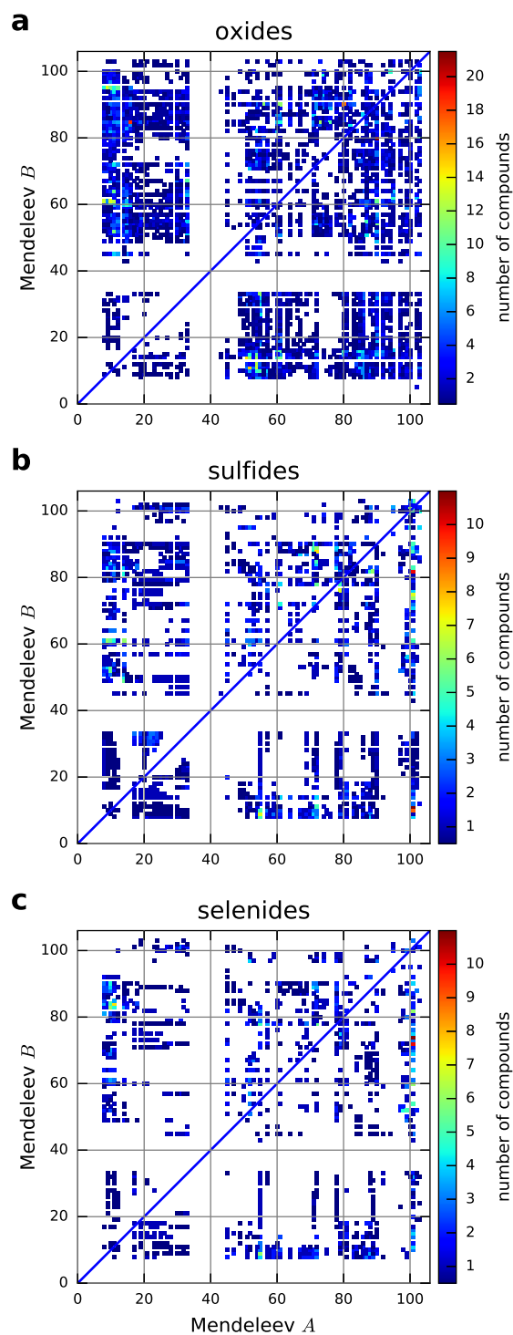
FIG. 8. Mendeleev maps of ternary (a) oxide A_xB_yO_z , (b) sulfide A_xB_yS_z and (c) selenide A_xB_ySe_z compounds. It is assumed that x \geq y with the x -axis indicating M_A and the y -axis M_B . If the stoichiometry is such that x = y , the compound is counted as 0.5A_xB_yO_z + 0.5B_xA_yO_z . A color scheme is used to represent the compound count for each composition, blue means the minimal number (one) and green means the maximal number which is different for each element.
