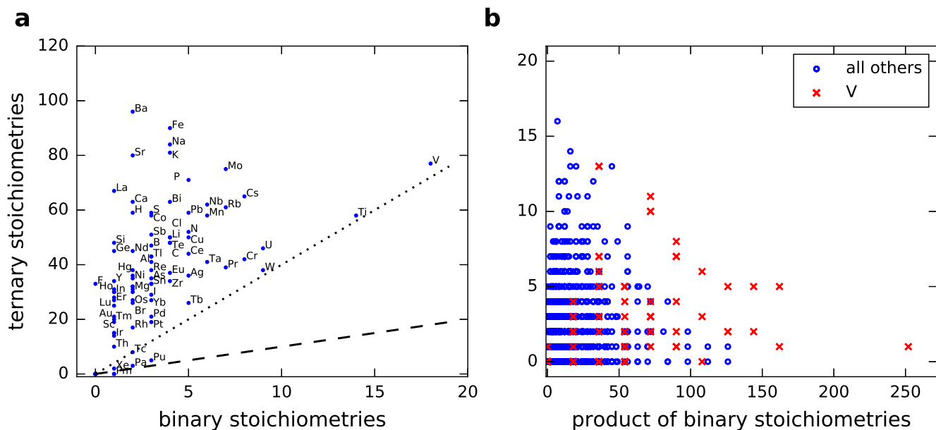
FIG. 6. (a) Prevalence of ternary oxide stoichiometries per atom as a function of the prevalence of its binary stoichiometries. The dashed line marks perfect similarity ( y = x ), and the dotted line marks the ratio y = 4x . (b) Number of oxide ternary stoichiometries as a function of product of participating elements numbers of oxide binary stoichiometries. The data for vanadium is shown with red crosses, all the rest is shown with blue circles.
