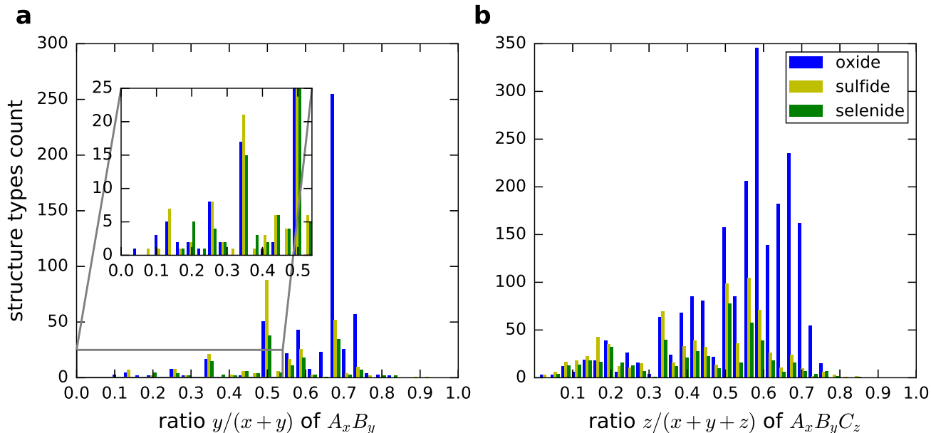
FIG. 2. The distribution of (a) binary stoichiometries and (b) ternary stoichiometries. Oxides are shown in blue, sulfides in yellow and selenides in green. The distributions of the selenides and sulfides are quite similar while those of the oxides deviate significantly, as detailed in the text.
