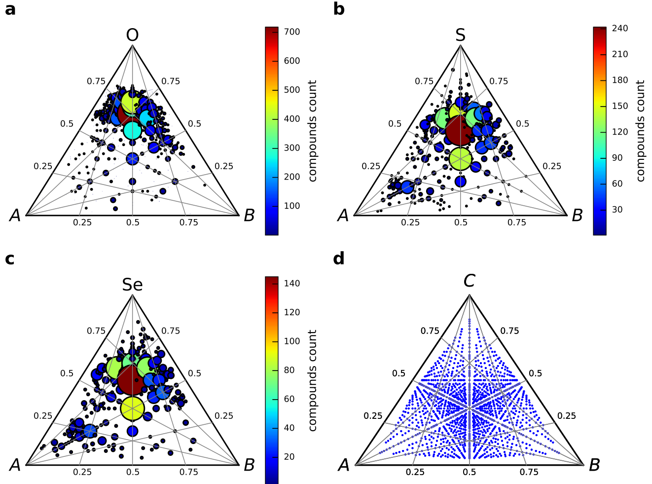
FIG. 4. Prevalence of stoichiometries among the ternary (a) oxide, (b) sulfide and (c) selenide compounds. (d) shows, for reference, all the possible stoichiometries with up to 12 atoms of each component per unit cell. In each figure, the smaller circles are normalized to the biggest one, which denotes the highest prevalence, i.e., 718 for oxides, 242 for sulfides, and 145 for selenides, in addition a heat map color scheme is used where blue means low prevalence and red means the highest prevalence for each element. The x and y axes denote the atomic fractions in the ternaries A_xB_yC_z , where C is O, S or Se, respectively. A and B are ordered by Mendeleev number where M_A > M_B .
