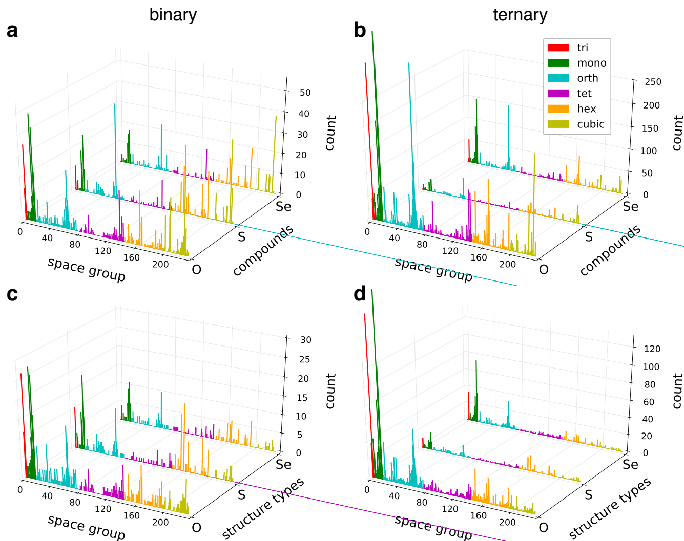
FIG. 12. Distribution of compounds and structure types among the 230 space groups. Binaries are on the left ( a and c ) and ternaries on the right ( b and d ). Compounds are depicted on the top ( a and b ) and structure types on the bottom ( c and d ).
