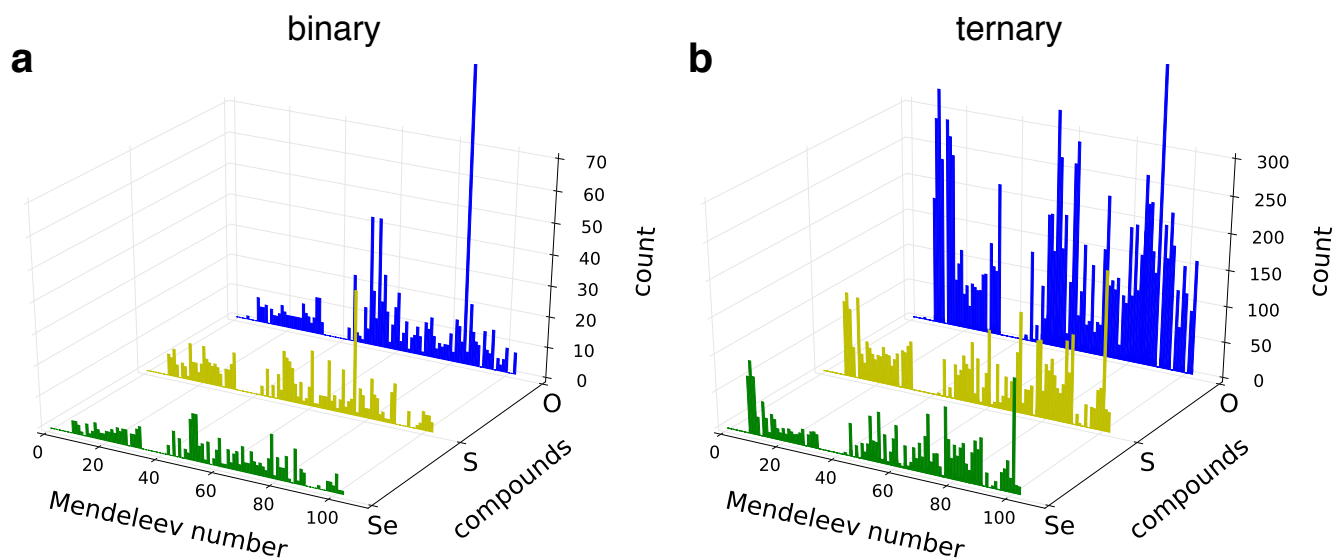
FIG. 7. Distribution of the elements in (a) binary and (b) ternary compounds. The binary oxides exhibit a structures distribution with two prominent peaks. The distributions of the binary sulfides and selenides are less structured and more similar to each other. The distributions of the ternary compounds have higher, wider peaks than their binary counterparts. The relative differences between the oxide, sulfide and selenide distributions remain similar to the distributions of the binaries.
