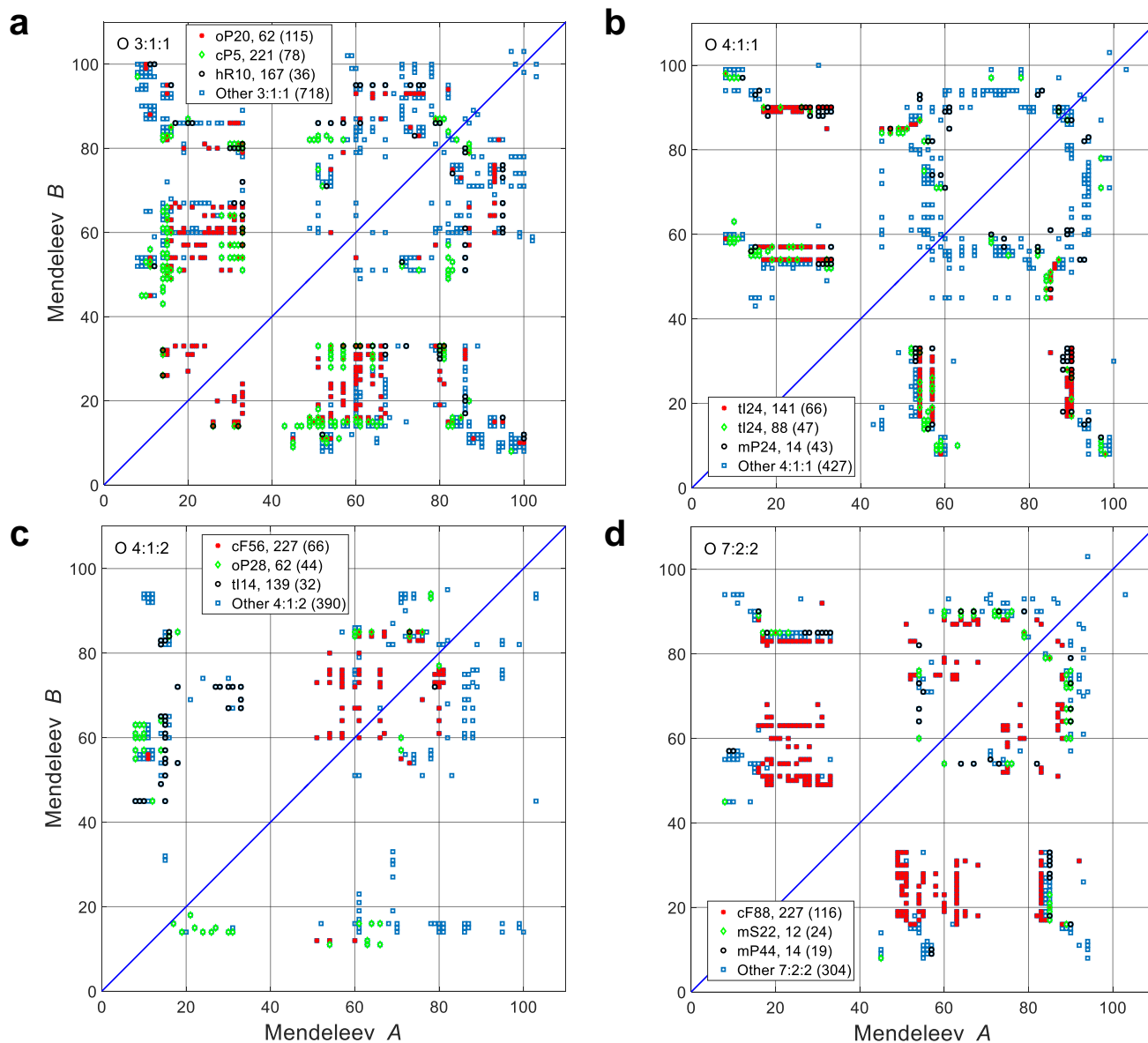
FIG. 9. Three leading structure types in each of the four leading stoichiometries in oxide ternaries: (a) A_1B_1O_3 , (b) A_1B_1O_4 , (c) A_1B_2O_4 , and (d) A_2B_2O_7 . The legend box appears at a region with no data points. The number in parenthesis is the number of compounds for this structure type, for “Other”, it refers to the total number of compounds with this stoichiometry.
