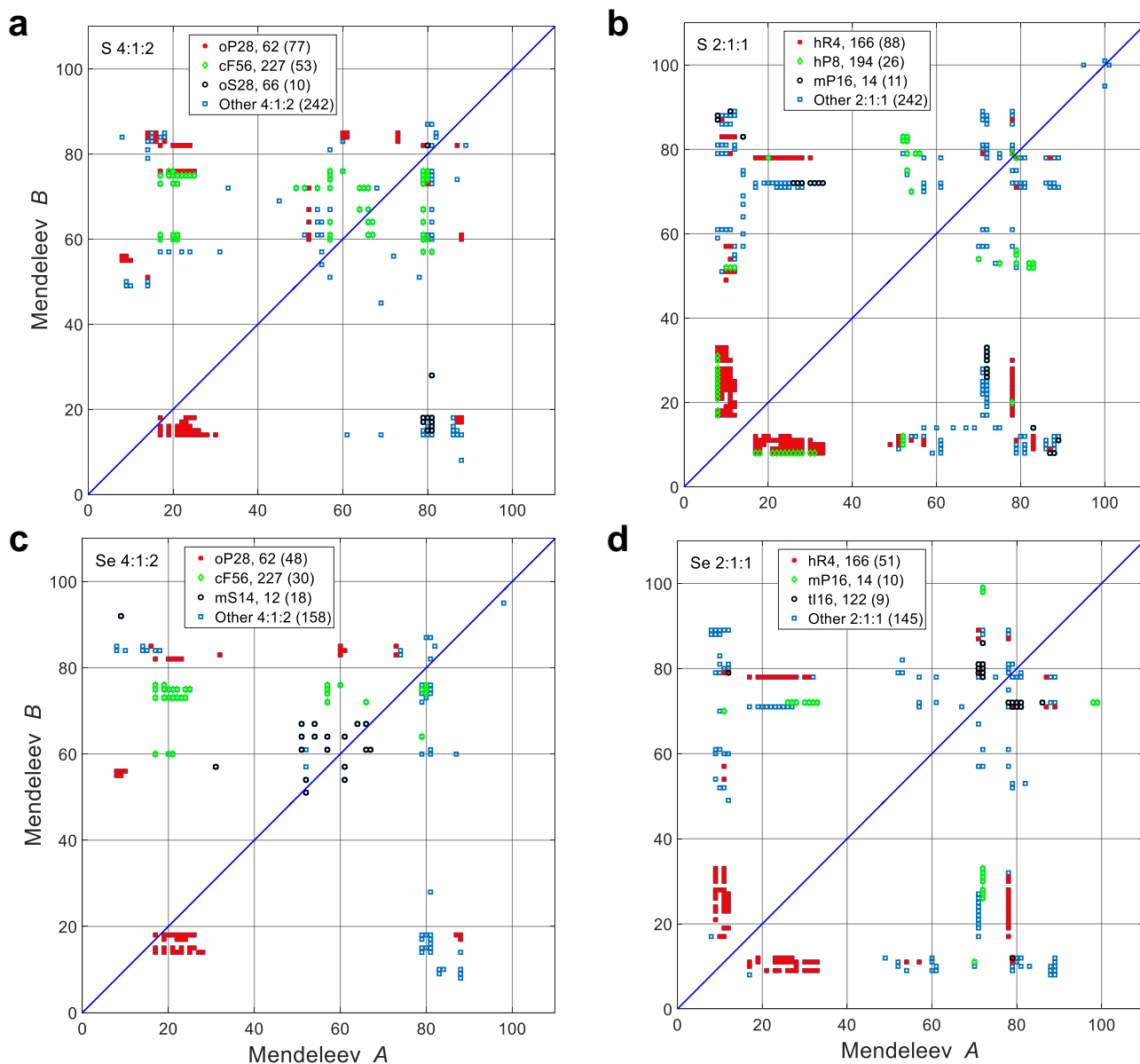
FIG. 10. Three leading structure types in each of the two leading stoichiometries in sulfur and selenium ternaries: (a) A_1B_2S_4 , (b) A_1B_1S_2 , (c) A_1B_2Se_4 , and (d) A_1B_1Se_2 . The number in parenthesis is the number of compounds for this structure type, for “Other”, it refers to the total number of compounds with this stoichiometry.
