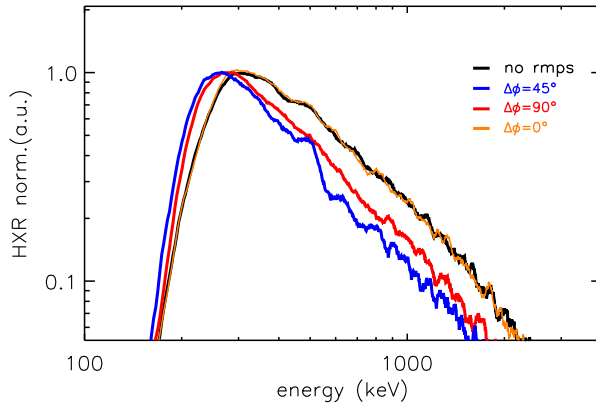
FIG. 8: (a): HXR energy spectrum from \text{LaBr}_3(\text{Ce}) scintillator diagnostic for standard shot (black, #33505) and for three with RMPs applied but with different \Delta\phi ( 45^\circ -blue curve #33506, 90^\circ - red curve #33112, 0^\circ - orange curve #33109).
