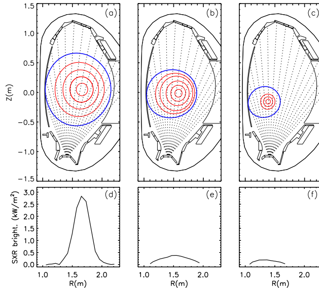
FIG. 2: Reconstruction of plasma equilibria at three different times for the shot #33108: panel (a) for t=0.98\text{s} , panel (b) for t=1.1\text{s} , panel (c) for t=1.18\text{s} . The dotted lines are the chords of the soft-X-ray tomography camera F. In (d),(e),(f) the associated soft-X-ray radiation as observed from the soft-x-ray tomography camera F.
