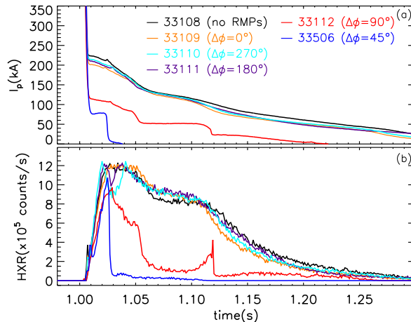
FIG. 4: (a) Plasma current during the post disruption phases for different values of \Delta\phi and (b) corresponding HXR emission from LaBr 3 (Ce) scintillator.
