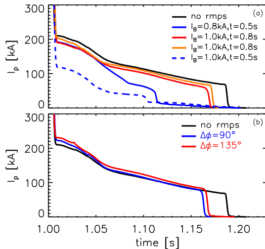
FIG. 13: (a) \Delta\phi = 45^\circ RMPs with different time of application and amplitude (black-#34150 reference shot without RMPs, blue solid-#34083, red-#34145 orange-#34146, blue-dashed: #33706- I_B = 1\text{kA} from t = 1\text{s} ); (b) Examples of discharges with RMPs applied from t = 1\text{s} (black-#34150, blue-#34143, red-#34144);
