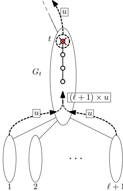
Figure 4: A parent group G_t with \ell + 1 children groups. The groups are depicted as ovals with edges connecting them. Each child group sends at most u units of demand to its parent group (dashed arrows). Thus, G_t receives at most (\ell + 1)u units of demand from its children. Inside G_t , the root t is a small star whose supporting facility has been closed. The demand of t , which is at most u , gets routed to the parent of G_t (assuming that it exists). Any other demand of G_t and all demand coming from its children is served within G_t .
