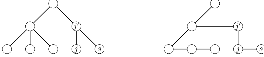
Figure 2: Making a tree binary: The left side shows one of the trees returned by Procedure Short-Trees( \mathcal{C}_{sc}, \emptyset ); the right side shows the corresponding tree after modification by Procedure Binary-Trees( G ). Observe that the father j' of s has been replaced by the left brother j of s .
