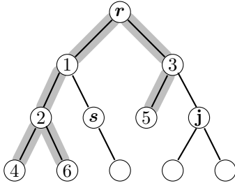
(a) Building groups: Edges highlighted in gray form a new group G_r with the root node r ; nodes s and j are roots of groups G_s and G_j , respectively. G_r is parent group of G_s and G_j . The numbers indicate a possible order in which the nodes have been added to G_r .
