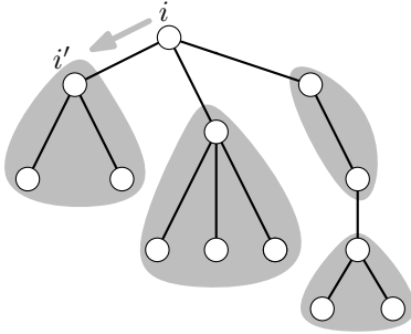
(a) A facility tree T . Shaded in gray are the facility stars that have been found in the while-loop of Procedure Facility-Stars( T ). Note that the root i has not been assigned to any star during the while-loop. If its opening \hat{y}_i is less than 1, it will be added to the son i' that satisfies i' = s(i) .
