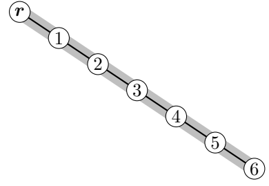
(b) The group G_r after the modification step: The group is now a chain and nodes are ordered from top to bottom in the order they were added to the group, that is, with non-decreasing distances to their fathers in the star tree.
