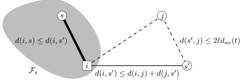
Figure 1: Let s \in \mathcal{C}_{sc} , j \in \mathcal{C} , i \in \mathcal{F}_s , and s' \in \mathcal{C}_{sc} be the closest star center to i . The distance d(i, s) (thick edge) is bounded by the distance d(i, s') (solid edge), which in turn is bounded by the detour over j (dashed path).
