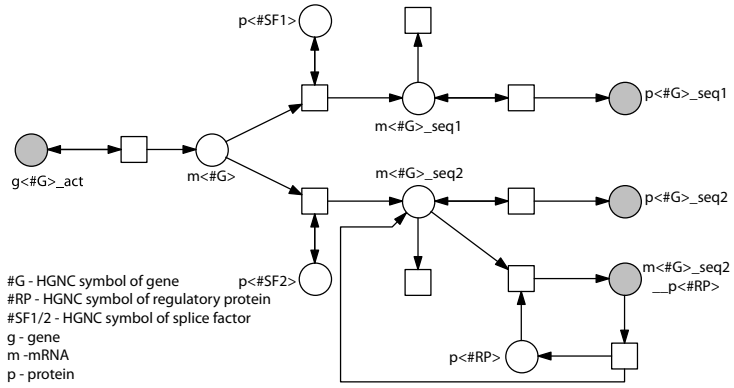
Figure 3.25: mRNA prototype modules for eukaryotes. The mRNA prototype module defines the synthesis of the mRNA (primary transcript) if its gene is transcriptionally active. Dependent on splice factors, the primary transcript is processed into mature transcripts. Transcripts may also interact with other regulatory proteins. Here, the transcriptionally active state of a gene g\langle\#G\rangle\_act triggers the synthesis of an mRNA m\langle\#G\rangle . Splice factor p\langle\#SF1\rangle triggers the processing of the mRNA m\langle\#G\rangle into the product m\langle\#G\rangle\_seq1 , which can either be degraded or start the synthesis of protein p\langle\#G\rangle\_seq1 . Splice factor p\langle\#SF2\rangle triggers the processing of the mRNA m\langle\#G\rangle into the product m\langle\#G\rangle\_seq2 , which can either be degraded, start the synthesis of protein p\langle\#G\rangle\_seq2 , or interact with a regulatory protein p\langle\#RP\rangle to form a complex m\langle\#G\rangle\_seq2\_p\langle\#RP\rangle (reversible). In this state, the processed mRNA cannot be translated. Note: Logical nodes indicate interface networks used to connect the mRNA module with corresponding protein and gene modules. (adapted from [116])
