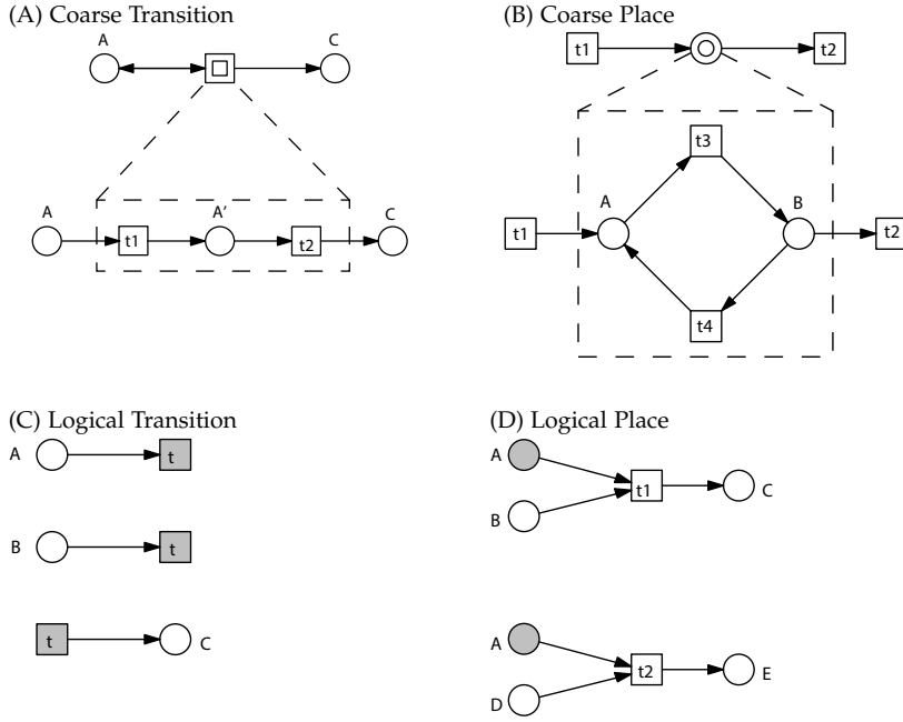
Figure 2.3: Coarse Nodes and Logical Nodes. Coarse transitions (A) and coarse places (B) yield hierarchically structured nets. Logical transitions (C) and logical places (D) connect remote parts of a net.
