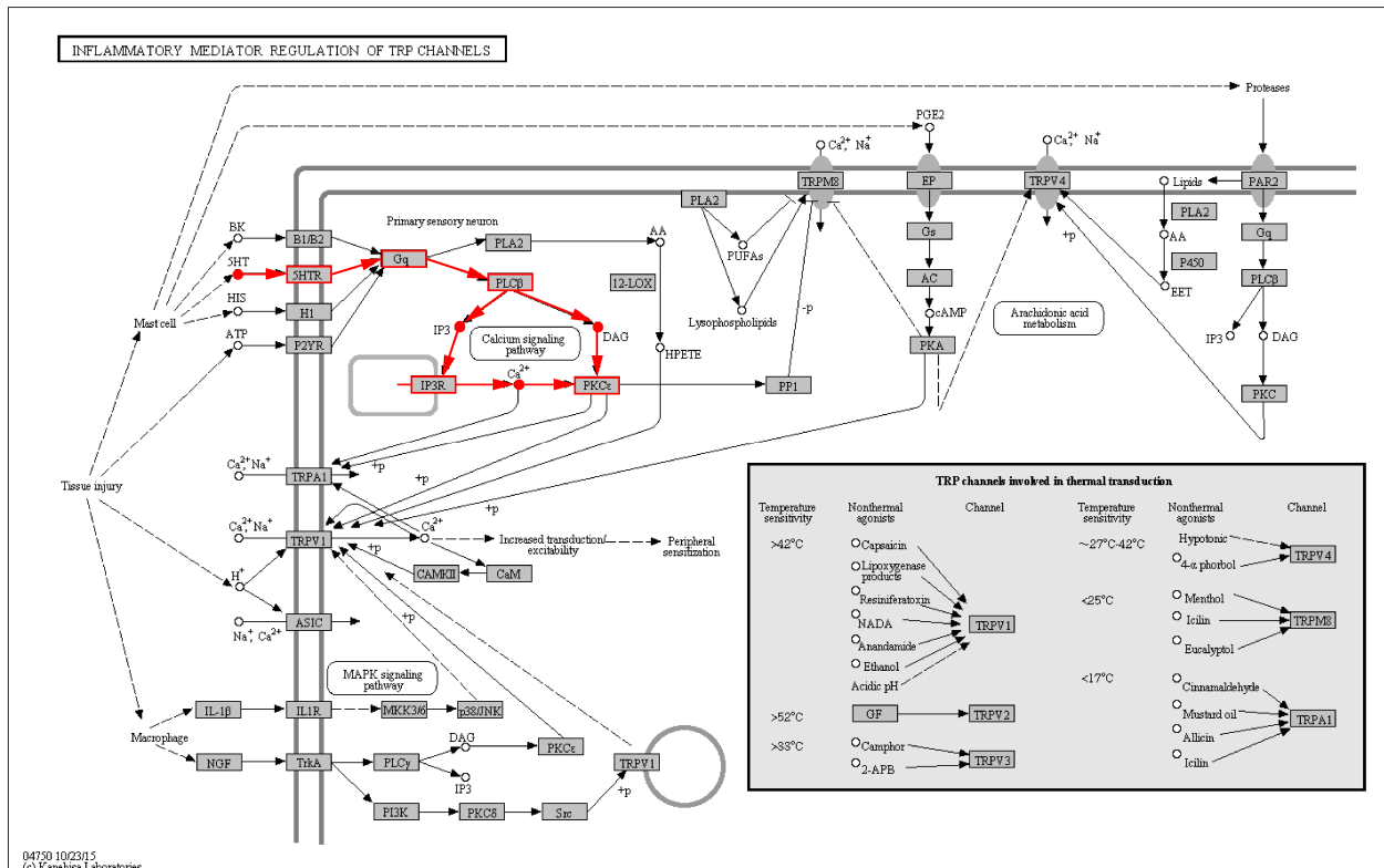
Figure 3.33: KEGG map for inflammatory mediator regulation of TRP channels (map04750). The PKC \epsilon pathway (depicted in red) is used as a running example for the modular Petri net transformation of SBML models.
