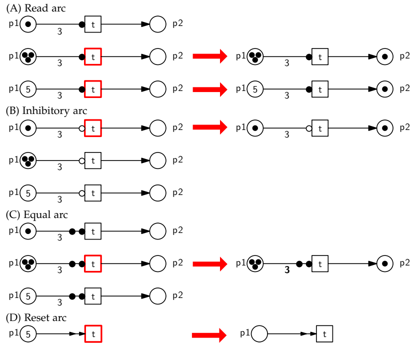
Figure 2.2: Regulatory arcs. Left side shows net before firing of transition t (only transitions marked in red are enabled). Right side shows net after firing of enabled transitions. (A) Read arc - transition t can only fire, if the marking on place p_1 is equal to or greater than the arc-weight. (B) Inhibitory arc - transition t can only fire, if the marking on place p_1 is less than the arc-weight. (C) Equal arc - transition t can only fire, if the marking on place p_1 is equal to the arc-weight. In (A)-(C) token remain on place p_1 after firing of transition t . (D) Reset arc - transition t can fire independent of the marking on place p_1 . The firing of transition t deletes all tokens on place p_1 .
