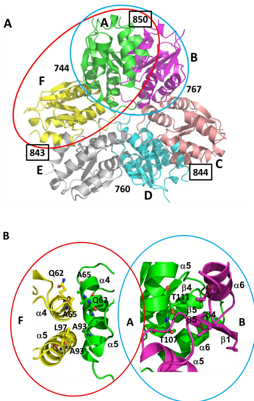
Figure 4. Mutational and structural analysis suggests hexamer disassembly into MgsA dimers. A. The disassembly of the hexamer (molecules colored and labeled as in Fig. 3) into dimers could result in two different dimers one leaving the active sites of one subunit in contact with the neighboring molecule (AF, indicated by a red ellipsoid) or disrupt the active site connecting surface (AB, indicated by a cyan ellipsoid). The numbers depicted indicate the average surface area (in \text{\AA}^2 ) of the individual molecules involved in interaction with the neighboring molecule. See text for details. B. Magnification of the interfaces AF and AB. The point mutations tested for interference with hexamer-formation of MgsA are indicated and only those located at the interface formed by the MgsA molecules A and F prevent hexamerization. Thus the monomers that interact to form the stable dimer require the other dimer interface (e.g. AB).
