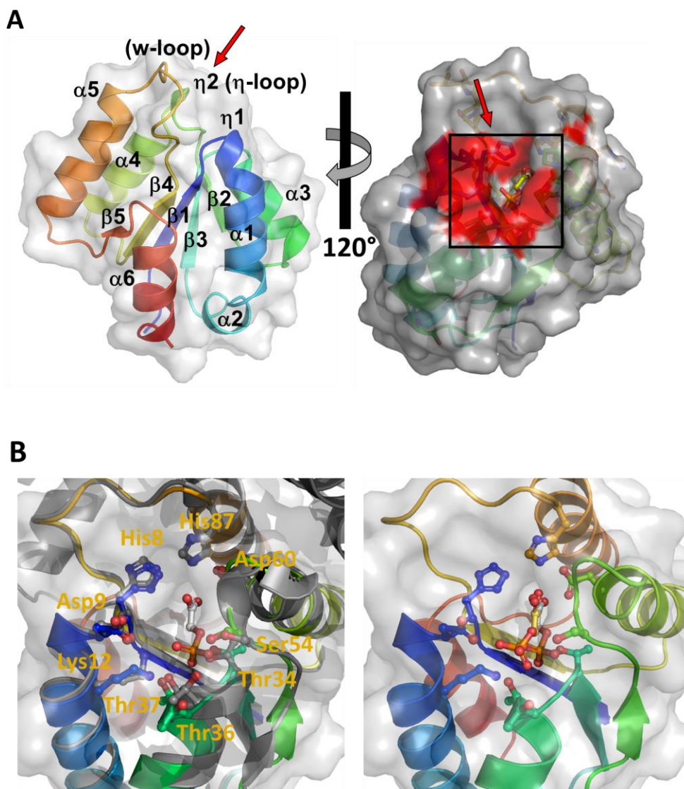
Figure 2. The structure of B. subtilis MgsA exhibits an overall globular shape. A. The central five-stranded \beta -sheet is flanked by six \alpha helices. Coloring in rainbow from N- (blue) to C-terminus (red). The surface structure is depicted in gray; the individual secondary structure motifs are indicated and numbered as \alpha -helices ( \alpha ) or \beta -strand ( \beta ) from the N to the C-terminus. The panel on the right shows a surface representation of an MgsA monomer in gray with the surface region of important active site residues highlighted in red. B. Left: Magnification of the active site as deduced from an overlay with the E. coli MgsA (gray) with 2-phosphoglycolic acid (ball and stick mode, PDB 1EGH) bound, serving as reference ligand. Cavity conformation and arrangement of active site residues are highly conserved (See also Fig. S3, S5). Identical residues of B. subtilis MgsA within the Mgs-family involved in ligand binding are depicted with their side chains in ball and stick mode with the C-atoms labelled according to Fig. 2A, with oxygen in red and nitrogen in blue. Residue numbering according to B. subtilis MgsA. Right: Result of a docking experiment with the substrate dihydroxyacetone phosphate (Carbons in yellow, phosphorus in orange) and phosphoglycolohydroxamic acid (PDB 1IK4) as reference.
