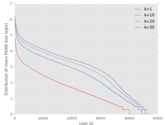
Figure 1: Distribution of the size of exposure sets. The values on Y axis are in logarithmic scale with base 10.
