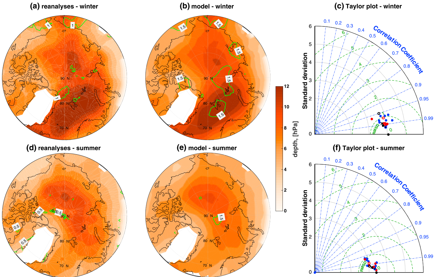
Figure 4. Spatial distribution of (a, b, d, and e) cyclone mean depth (hPa) and (g, h, j, and k) size (km) in (a, b, g, and h) winter and (d, e, j, and k) summer from multireanalysis and multimodel ensemble. The green isolines indicate the standard deviations across the models or reanalyses. Taylor plots for (c and f) depth and (i and l) size are also given (same legend as in Figure 1).
