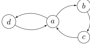
■ Figure 1 A graph G_e = (V_e, E_e) with two simple cycles sharing a single node.
