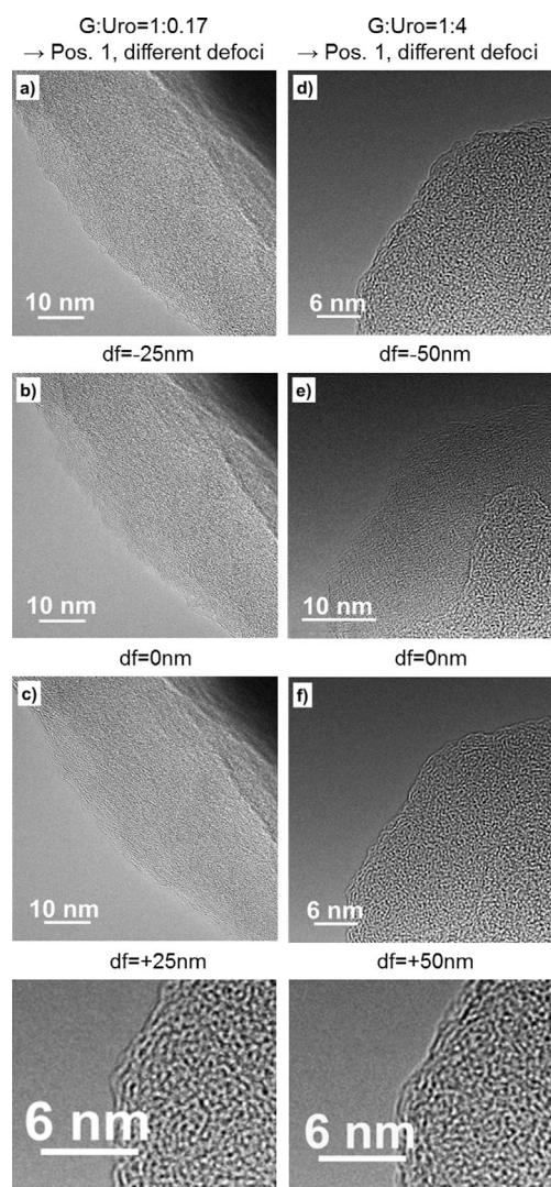
Figure 6. HRTEM images of N-HTCs with 1:0.17 (a–c) and 1:4 (d–f) G/Uro, obtained by applying different defocus (df) values. The bottom row shows cropped HRTEM images to highlight the isotropic carbon structures.
