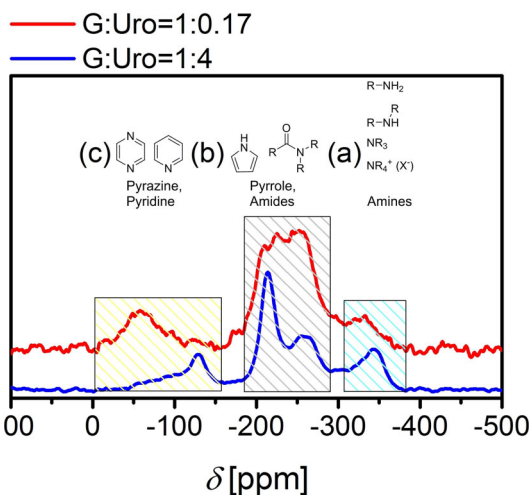
Figure 19. ^{15}\text{N} CP MAS NMR spectrum, with 30 kHz spinning frequency, for 1:0.17 (red) and 1:4 G/Uro (blue).
