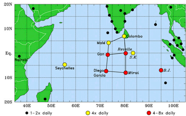
FIG. 1. Map showing the DYNAMO enhanced sounding network with color coding of dots indicating frequency of soundings during the SOP. Note that soundings at Sagar Kanya (SK) and Baruna Jaya (BJ) sites were available only for short periods during the SOP.
