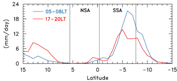
FIG. 8. Latitudinal cross section of TRMM 3B42 rainfall averaged over 72^{\circ} – 80^{\circ} E for 0500–0800 LT (blue) and for 1700–2000 LT (red). Light vertical lines show latitudinal limits of the enhanced sounding arrays.
