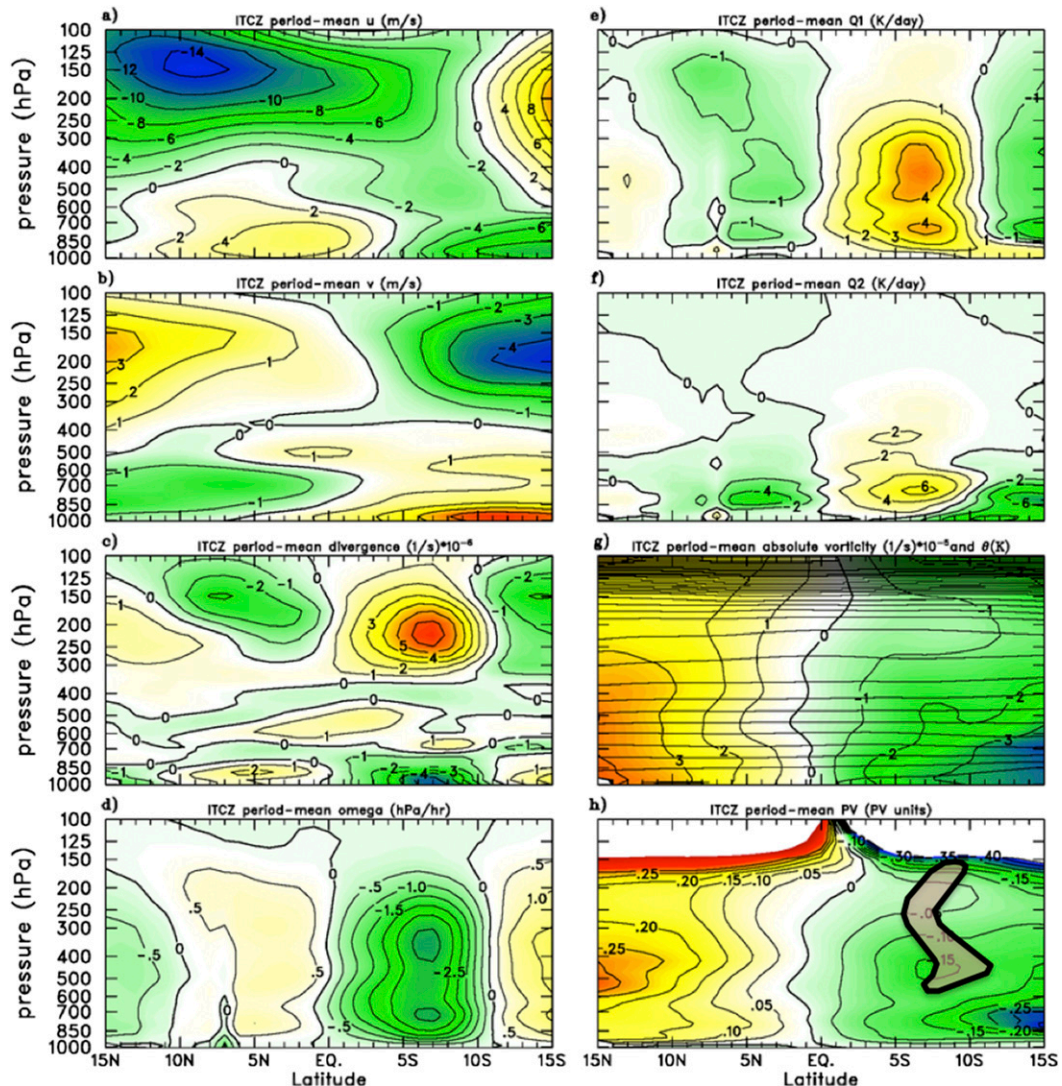
FIG. 5. ITCZ period-mean (1–14 Oct 2011) latitudinal cross section averaged over 72^{\circ} – 80^{\circ} E for (a) zonal wind field, (b) meridional wind field, (c) divergence, (d) vertical p velocity, (e) apparent heating, (f) apparent drying, (g) absolute vorticity (color) and potential temperature (contours with 5-K increment), and (h) potential vorticity. In Fig. 5h the shaded region represents the area where the meridional PV gradient is reversed, satisfying the Charney–Stern necessary condition for combined barotropic–baroclinic instability.
