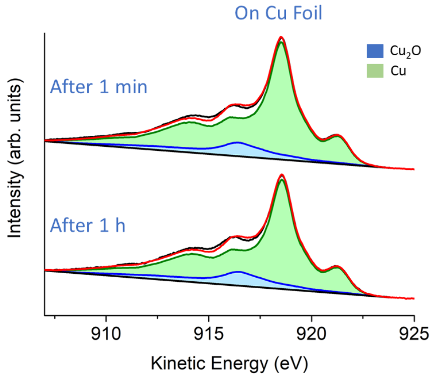
Figure S4: Cu AES LMM Spectra of 250 nm Cu-Cubes on a Cu Foil measured quasi in situ after 1 minute and 1 hour of \text{CO}_2\text{RR} at -1.0V vs RHE.
