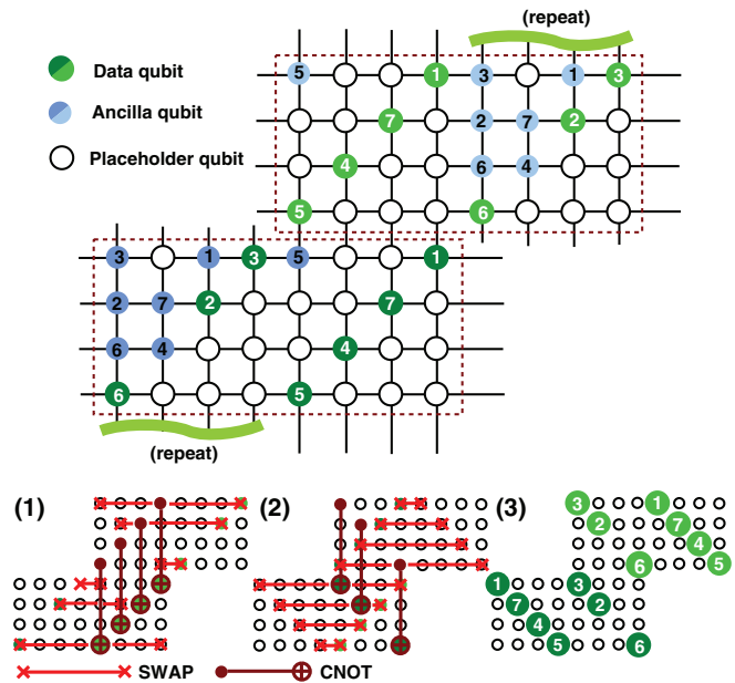
Fig. 4: (Colour on-line) A possible fault-tolerant scalable architecture based on the cavity grid. Top: the unit cell of a periodic arrangement, with two logical qubits, each made up of seven data qubits (grouping indicated by dashed rectangles), together with ancilla and placeholder qubits. Bottom: the sequence of SWAP and CNOT gates shown in (1) and (2) implements a transversal CNOT between the logical qubits, producing the final arrangement (3); see main text.
