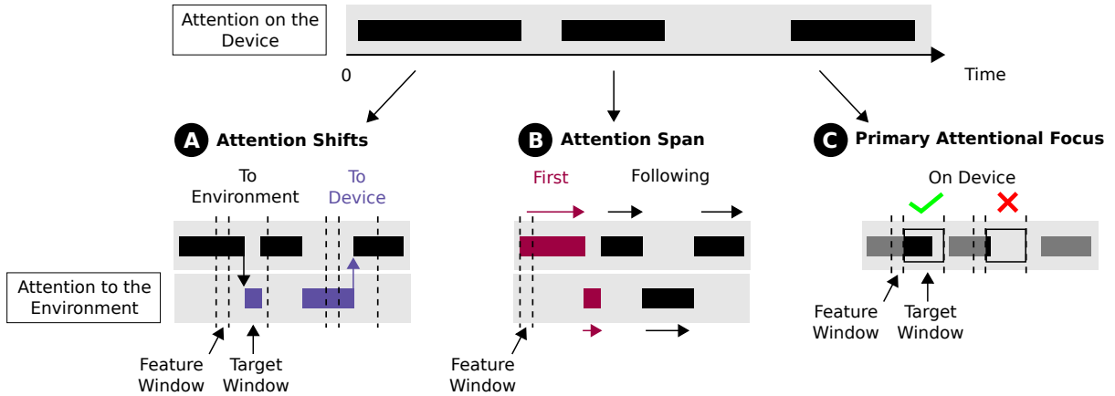
Fig. 2. Overview of the different prediction tasks explored in this work: Prediction of attention shifts to the environment and (back) to the device, the duration of the first and total (first and all following) attention spans, as well as the primary attentional focus, i.e. whether attention is primarily on or off the device.
