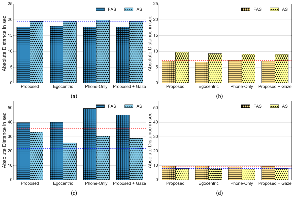
Fig. 10. Performance for predicting the first and total attention spans on the phone (a,b) and on the environment (c,d) during (a, c) working and (b, d) waiting time segments for the different feature sets. The mean attention span length on the training set for the first and total attention spans are indicated by the red and blue dashed lines, respectively.
