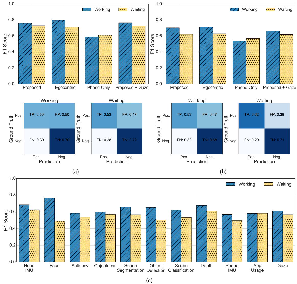
Fig. 7. Performance for predicting shifts to the environment during working and waiting time segments for the different feature sets for a) one-second and b) five-second target window with the corresponding confusion matrices for our proposed feature set, and c) a more detailed feature analysis of b).
