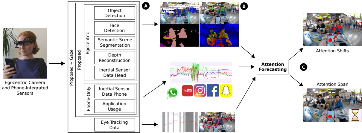
Fig. 3. Overview of our method for attention forecasting during mobile interactions. Taking information on users’ visual scene, phone and head inertial data, as well as on mobile app usage as input (A), our method extracts rich semantic information about the user’s visual scene using state-of-the-art computer vision methods for object and face detection, semantic scene segmentation, and depth reconstruction (B). The method then extracts and temporally aggregates phone and visual features and takes eye tracking data into account to predict attention shifts and attention span (C).
