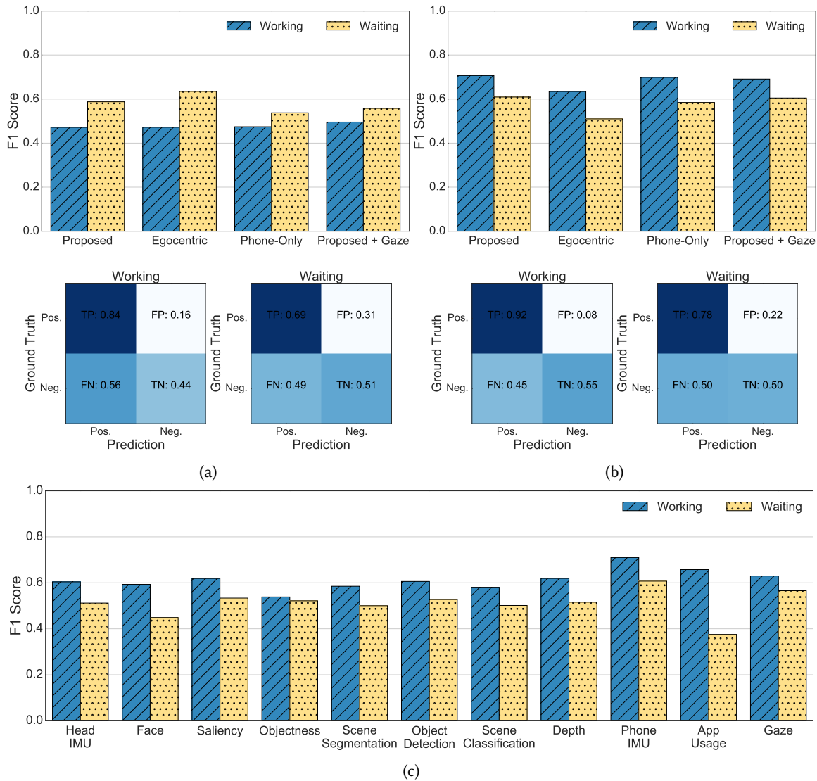
Fig. 8. Performance for predicting shifts to the mobile phone during working and waiting time segments for the different feature sets for a) one-second and b) five-second target window with the corresponding confusion matrices for our proposed feature set, and c) a more detailed feature analysis of b).
