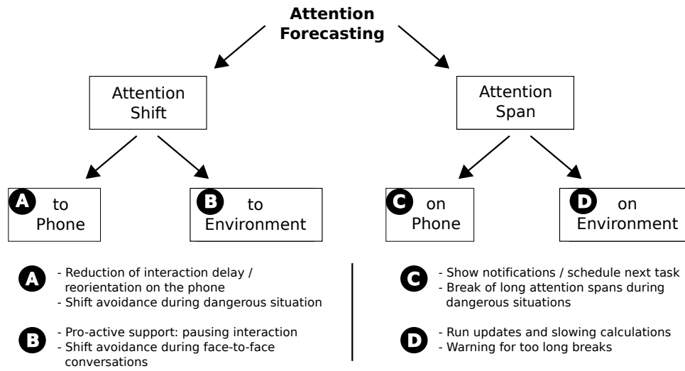
Fig. 12. Potential applications of attention forecasting (attention shifts and attention spans) in future attentive user interfaces.
