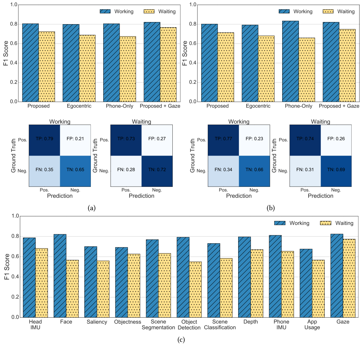
Fig. 11. Performance for primary attentional focus on mobile phone during working and waiting time segments for the different feature sets for a) one-second and b) five-second target window with the corresponding confusion matrices for our proposed feature set, and c) a more detailed feature analysis of b).
