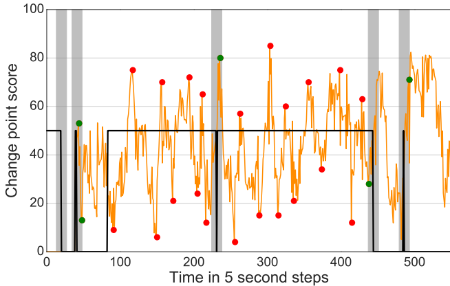
Figure 5: Change point detection example with ground-truth privacy sensitivity level shown in black. The grey vertical bars indicate the margin around the change points. The red dots indicate all detected change points; the green dots only correctly detected change points.
