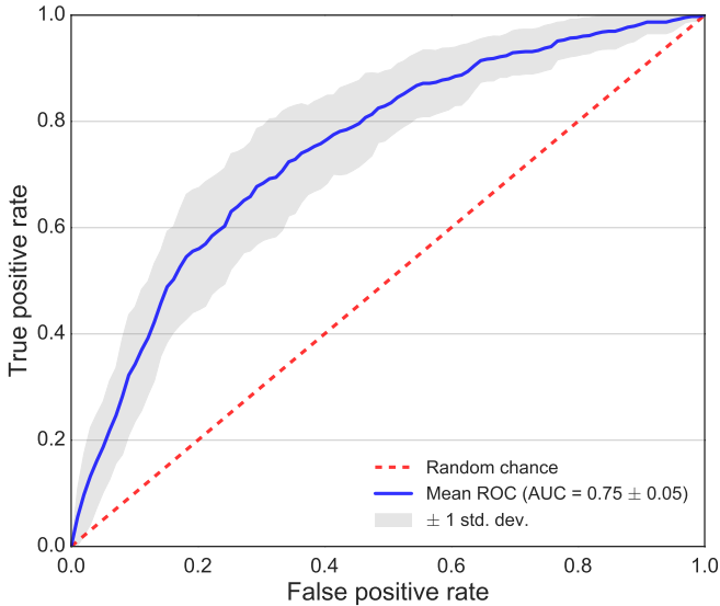
Figure 9: Received operating characteristic (ROC) curve as a result of leave-one-person-out cross validation for detecting privacy-sensitive situations using the first-person camera.
