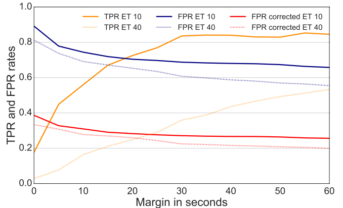
Figure 10: True positive rate (TPR) and false positive rate (FPR) over all participants for different offsets and extrema threshold (ET) values for the extrema detection. The corrected FPS rate describes the performance in combination with the vision based deep-learning method when checking the first frame after re-opening the camera shutter.
