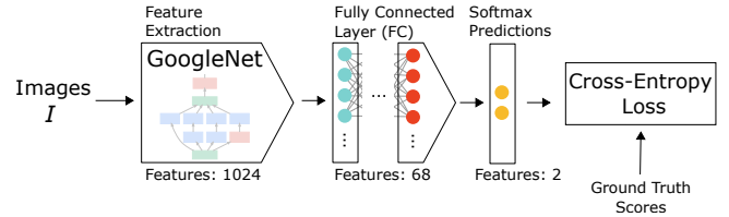
Figure 4: Our method for detecting privacy-sensitive situations is based on a pre-trained GoogleNet model that we adapted with a fully connected (FC) and a Softmax layer. Cross-entropy loss is used for training the model.
