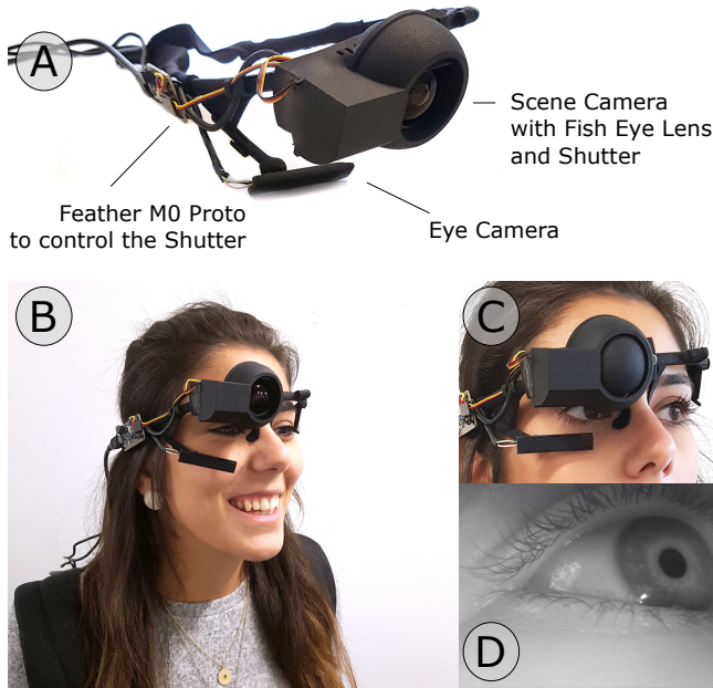
Figure 3: PrivacEye prototype, with labelled components (A), and worn by a user with an USB-connected laptop in a backpack (B). Detection of privacy-sensitive situations using computer vision closes the camera shutter (C), which is re-opened based on detected changes in users’ eye movement (D).
