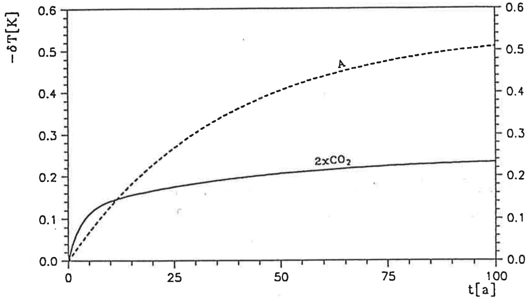
Figure 7: Cold start temperature errors for the model ECHAM-1/LSG determined from the impulse response function inferred from the “ 2\times\text{CO}_2 ” experiment (full line) and from the Scenario A simulation (dashed line).
