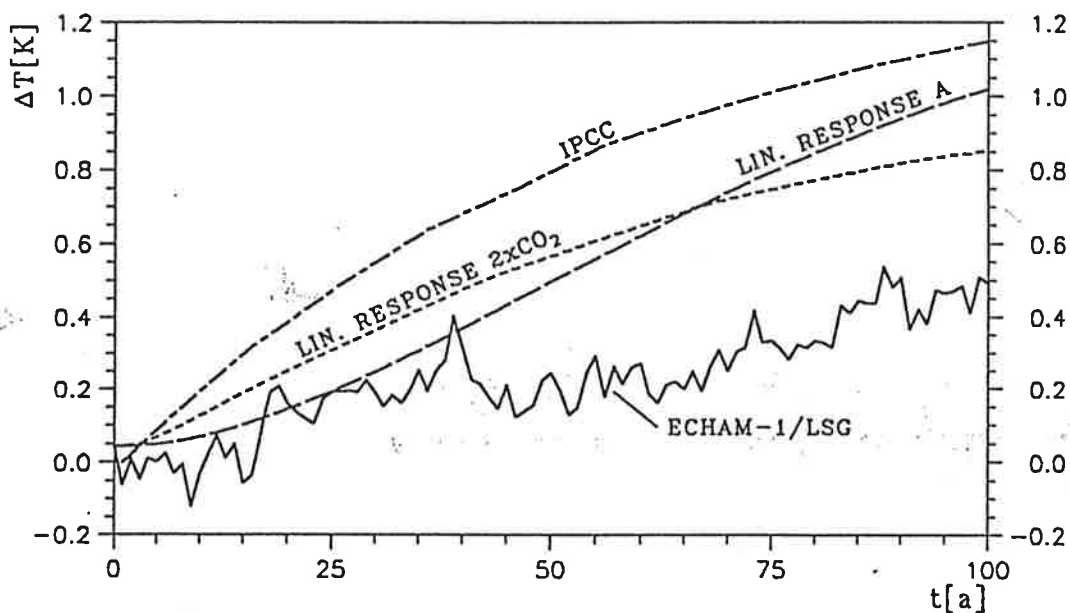
Figure 9: Temperature response of the coupled model ECHAM-1/LSG for Scenario D, its approximations by the linear response models inferred from the “2×CO 2 ” experiment and the Scenario A simulation, and the estimated IPCC response.
