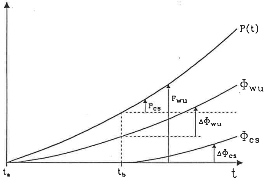
Figure 1: Definition of the cold start-problem. \Phi_{wu} and \Phi_{cs} denote the responses to the forcings F_{wu} and F_{cs} , respectively. The change since time t_b is larger for the warm-up case “ wu ” than for the cold start case “ cs ”.
