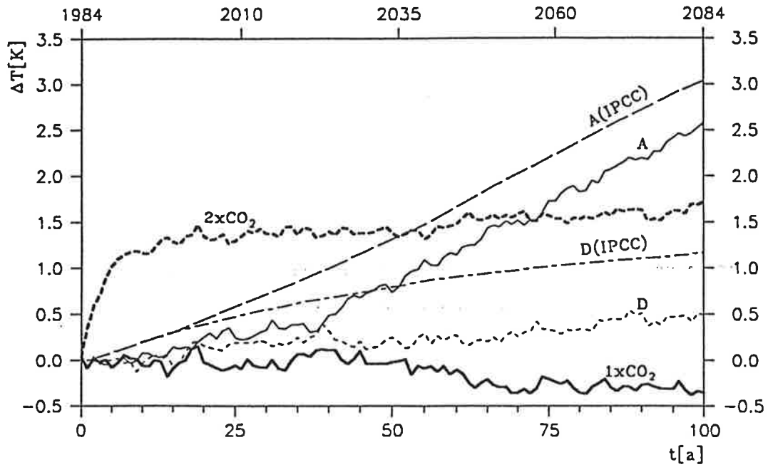
Figure 5: Change of the global mean near surface (2m) temperature due to increased \text{CO}_2 concentration as simulated with ECHAM-1/LSG (Scenarios A and D, “ 2\times\text{CO}_2 ”, and “ 1\times\text{CO}_2 ” = control) and as estimated by IPCC (Scenarios A und D). All changes are defined relative to the mean of the years 1–10 of the control simulation.
