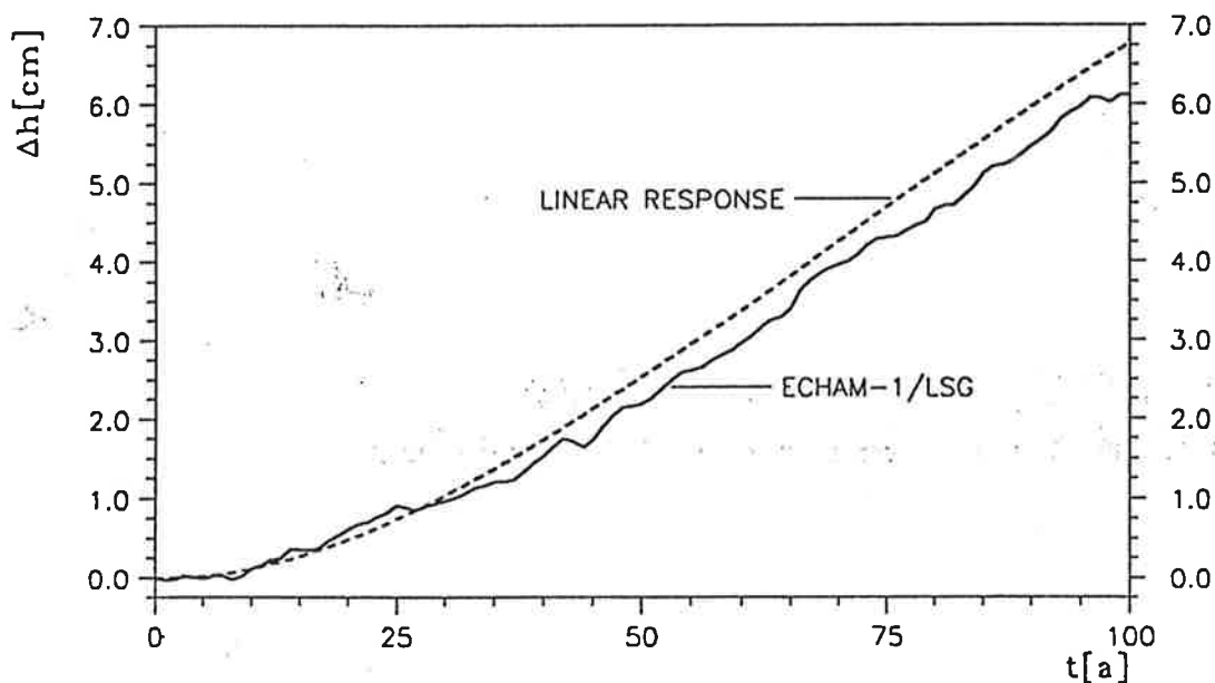
Figure 15: Sea level response of ECHAM-1/LSG for Scenario D (full line), and its approximation by the linear response model (dashed line). The impulse response function is based on Scenario A.
