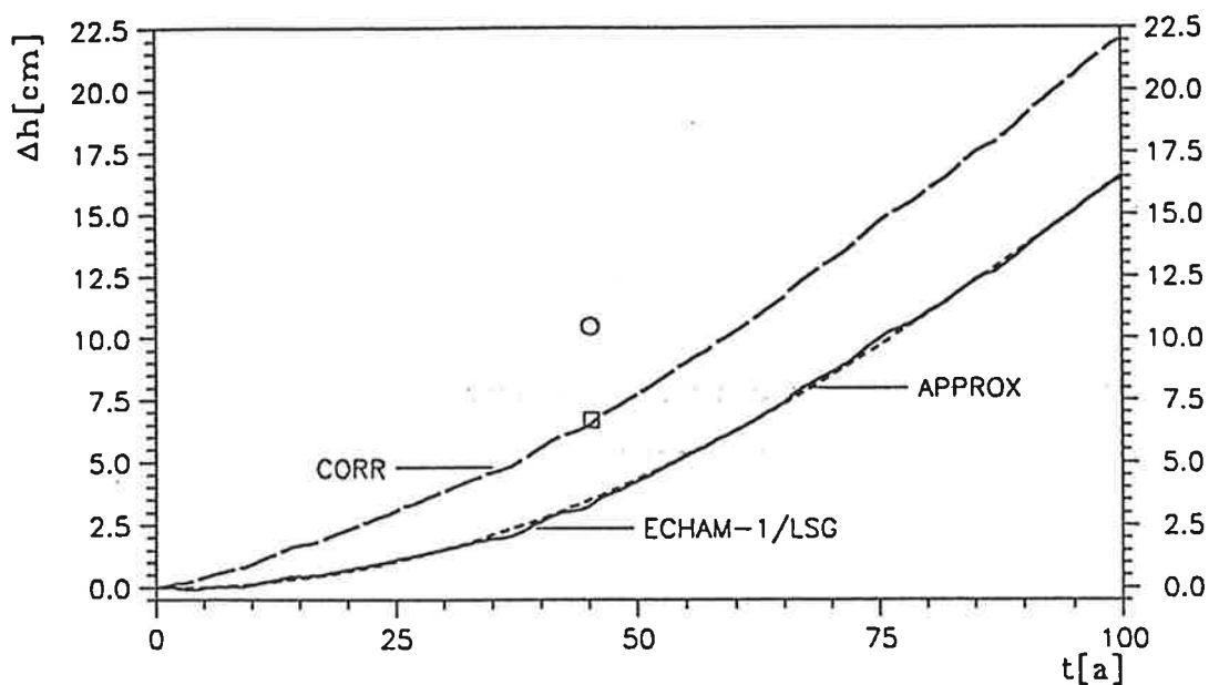
Figure 14: Scenario A sea level rise relative to the control integration: simulation by ECHAM-1/LSG, approximation of the ECHAM-1/LSG curve by a fit (APPROX), and the cold start error corrected simulation by ECHAM-1/LSG (CORR). “o” (best estimate) and “□” (low estimate) denote the IPCC Scenario A estimate (thermal expansion only).
