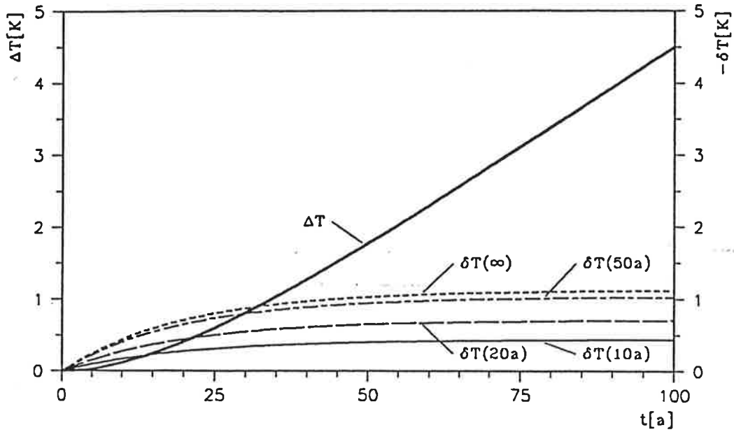
Figure 3: Temperature response \Delta T (heavy line) to linear forcing in the cold start case and the underestimation -\delta T (thin lines) of the (true) warm-up response for several warm-up times ( t_b - t_a = 10 a, 20 a, 50 a, \infty ).
