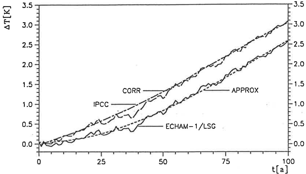
Figure 10: Temperature response for Scenario A: simulation by ECHAM-1/LSG, estimation by IPCC, approximation of the ECHAM-1/LSG curve by a fit (APPROX), and the cold start error corrected simulation by ECHAM-1/LSG (CORR).
