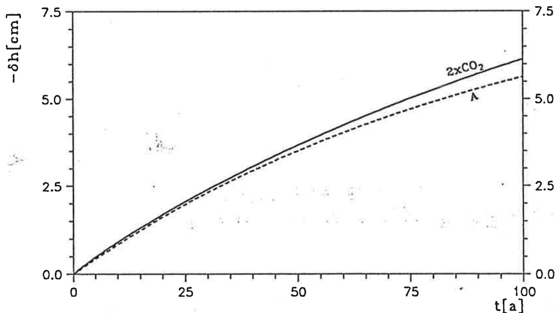
Figure 13: Errors in sea level height due to the cold start for the model ECHAM-1/LSG based on the impulse response functions determined from the \text{CO}_2 “doubling” experiment (full line) and from the Scenario A simulation (dashed line).
