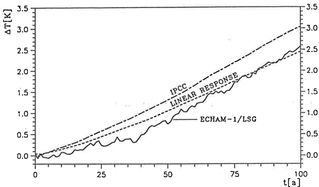
Figure 8: Temperature response of the coupled model ECHAM-1/LSG for Scenario A, its approximation by the linear response model inferred from the “2×CO 2 ” experiment and the estimated IPCC response.
