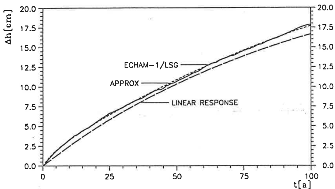
Figure 12: Response of the global height of sea level to an instantaneous \text{CO}_2 “doubling” (“ 2\times\text{CO}_2 ” – “ 1\times\text{CO}_2 ”) for ECHAM-1/LSG (full line), and its approximation by a fit (APPROX, dotted line) and by a linear response model based on Scenario A (LINEAR RESPONSE, dashed line).
