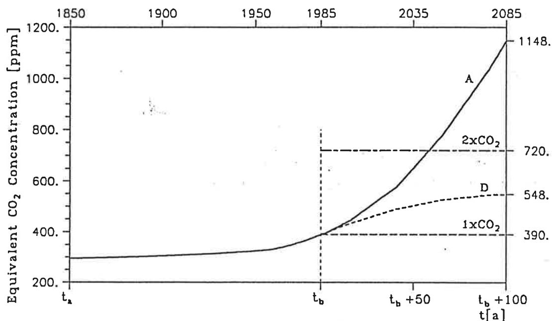
Figure 4: Equivalent CO 2 concentrations for Scenarios A and D, the instantaneous CO 2 “doubling”, and the control simulation from Houghton et al. (1990).
