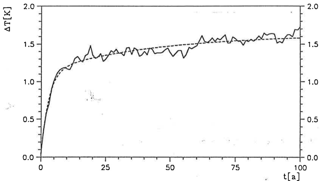
Figure 6: Temperature response of the coupled model ECHAM-1/LSG to an instantaneous \text{CO}_2 “doubling” (full line) and its approximation by a two-exponential linear response model (dashed line).
