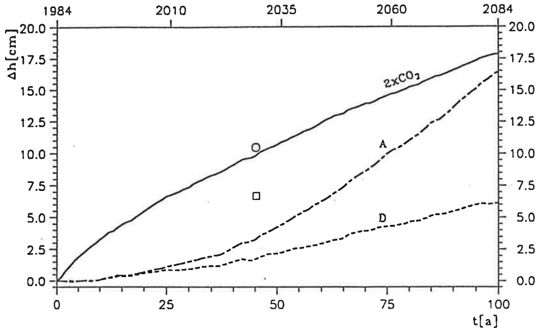
Figure 11: Change of sea level height relative to the control simulation in the three ECHAM-1/LSG integrations (lines). "O" (best estimate) and "□" (low estimate) denote the IPCC Scenario A estimates (thermal expansion only).
