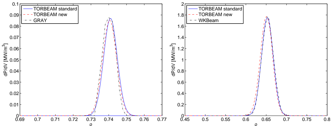
Fig. 3. Power deposition profiles obtained with TORBEAM standard procedure (blue solid) and TORBEAM new procedure (red dashed), for (a) an ITER scenario (left, also GRAY profile shown, black dashed-dotted) and (b) an off-axis ASDEX Upgrade scenario (right, also WKBeam profile shown, black dashed-dotted).
