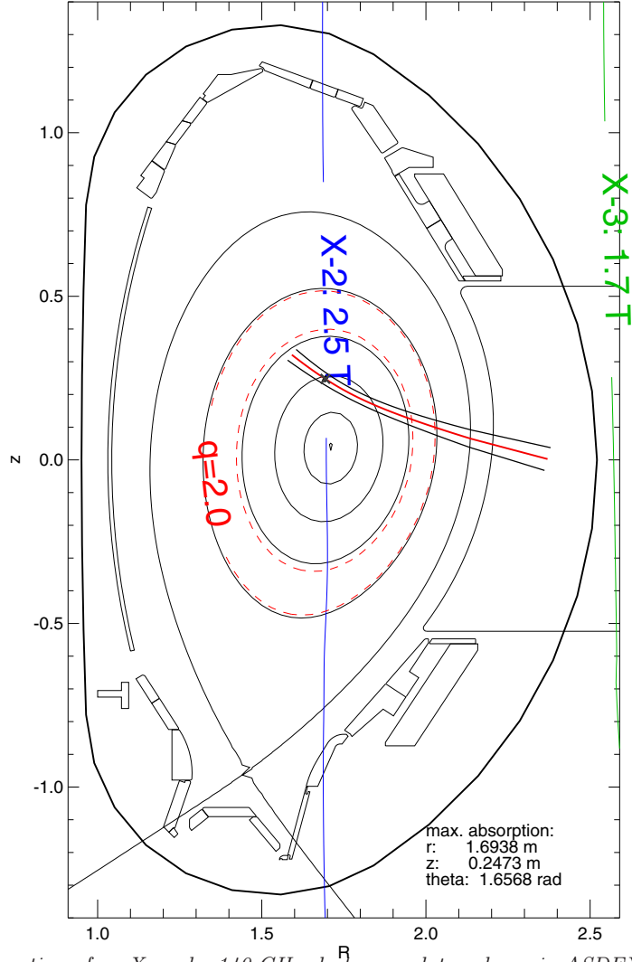
Fig. 1. Propagation of an X-mode, 140 GHz electron cyclotron beam in ASDEX Upgrade as calculated by TORBEAM, visualized as a projection along the cylindrical angle \varphi . The beam, launched at (R, Z) = (2.38, 0) m, is represented through its reference ray (tracing the maximum of the Gaussian amplitude envelope, red) and the beam width (“peripheral rays”) representing the intersection of the 1/e level of the amplitude with a vertical plane. The vertical lines show the position of the second (X-2, blue) and third (X-3, green) cyclotron harmonics.
