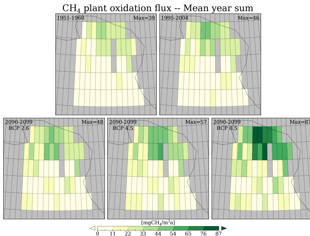
Figure B.5: Modelled rhizospheric methane oxidation flux as mean year sum over 10 years periods in \text{mgCH}_4 \text{m}^{-2} \text{a}^{-1} . Please note the details at the top of every subfigure.
