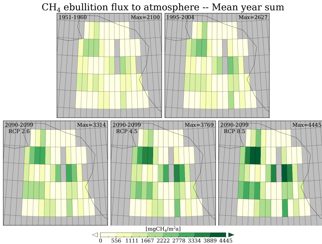
Figure B.6: Modelled methane ebullition flux to the atmosphere as mean year sum over 10 years periods in mgCH 4 m -2 a -1 . Please note the details at the top of every subfigure.
