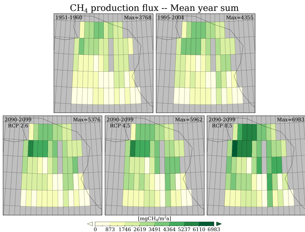
Figure 3.14: Modelled methane production flux as mean year sum over 10 years periods in mgCH 4 m -2 a -1 . Please note the details at the top of every subfigure.
