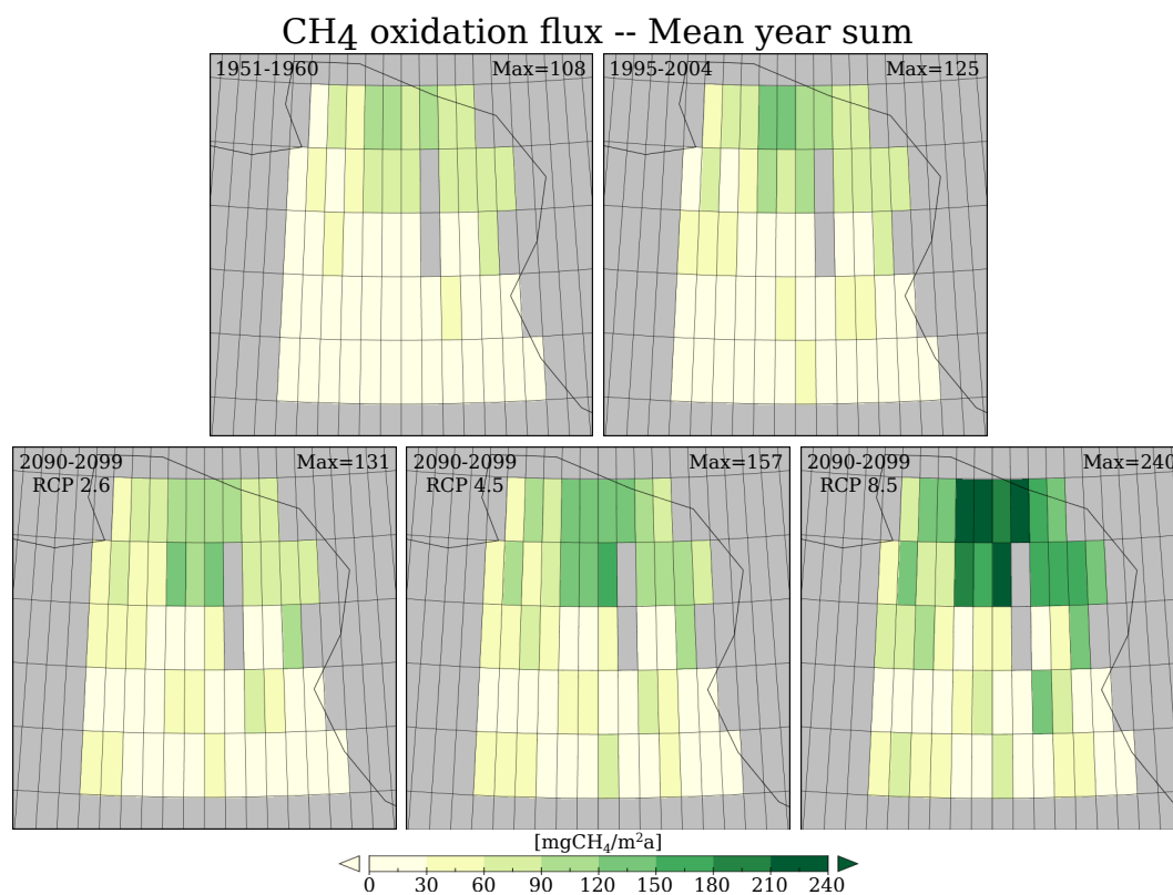
Figure B.4: Modelled bulk soil methane oxidation flux as mean year sum over 10 years periods in \text{mgCH}_4 \text{m}^{-2} \text{a}^{-1} . Please note the details at the top of every subfigure.
