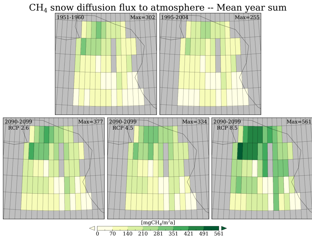
Figure B.7: Modelled methane diffusion through snow flux to the atmosphere as mean year sum over 10 years periods in mgCH 4 m -2 a -1 . Please note the details at the top of every subfigure.
