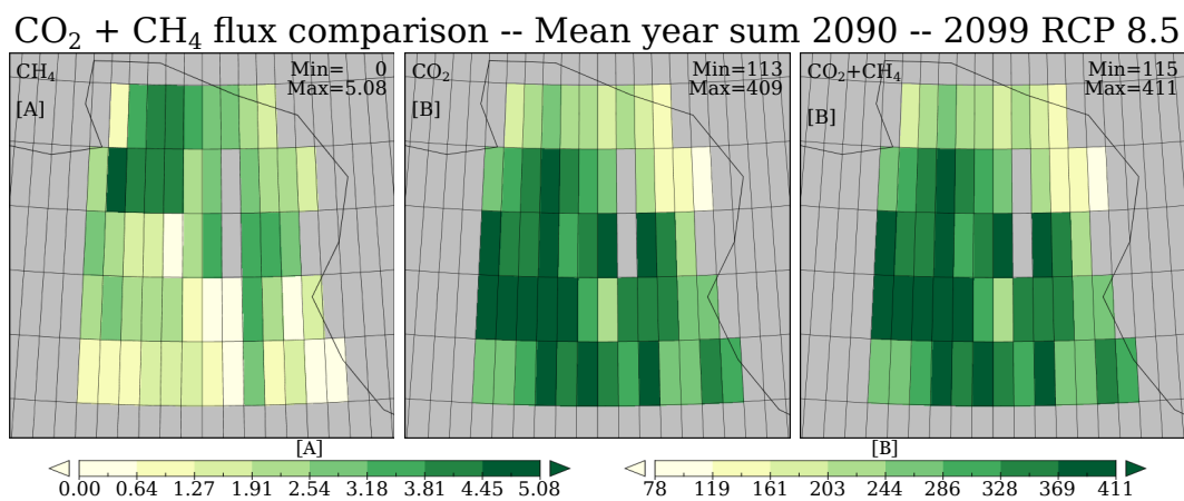
Figure 3.13: Modelled soil respiration fluxes as mean year sum for 2090–2099 under RCP8p5 in g of C per m 2 and per year. Please note the different scales [A] and [B] and the details at the top of every subfigure.
