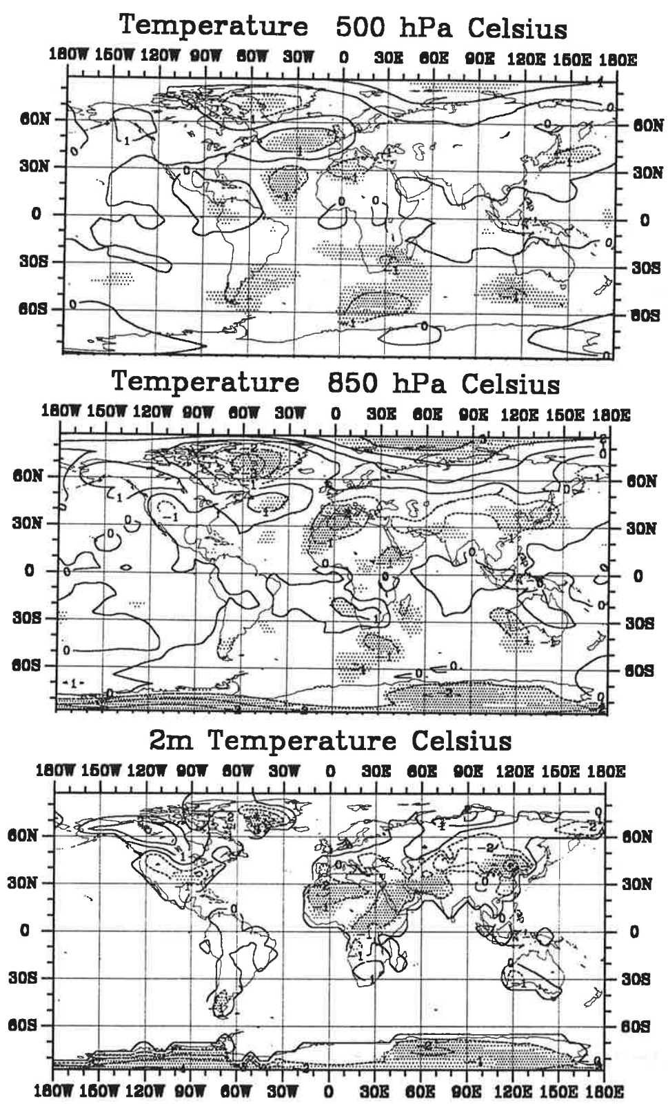
Figure 9: Anomalies of the air temperature in the lower troposphere. Shading indicates statistically significant (error chance 5%) differences between Control and Experiment for months 31 to 60 on the basis of a local t-test, degrees of freedom reduced to 15.
