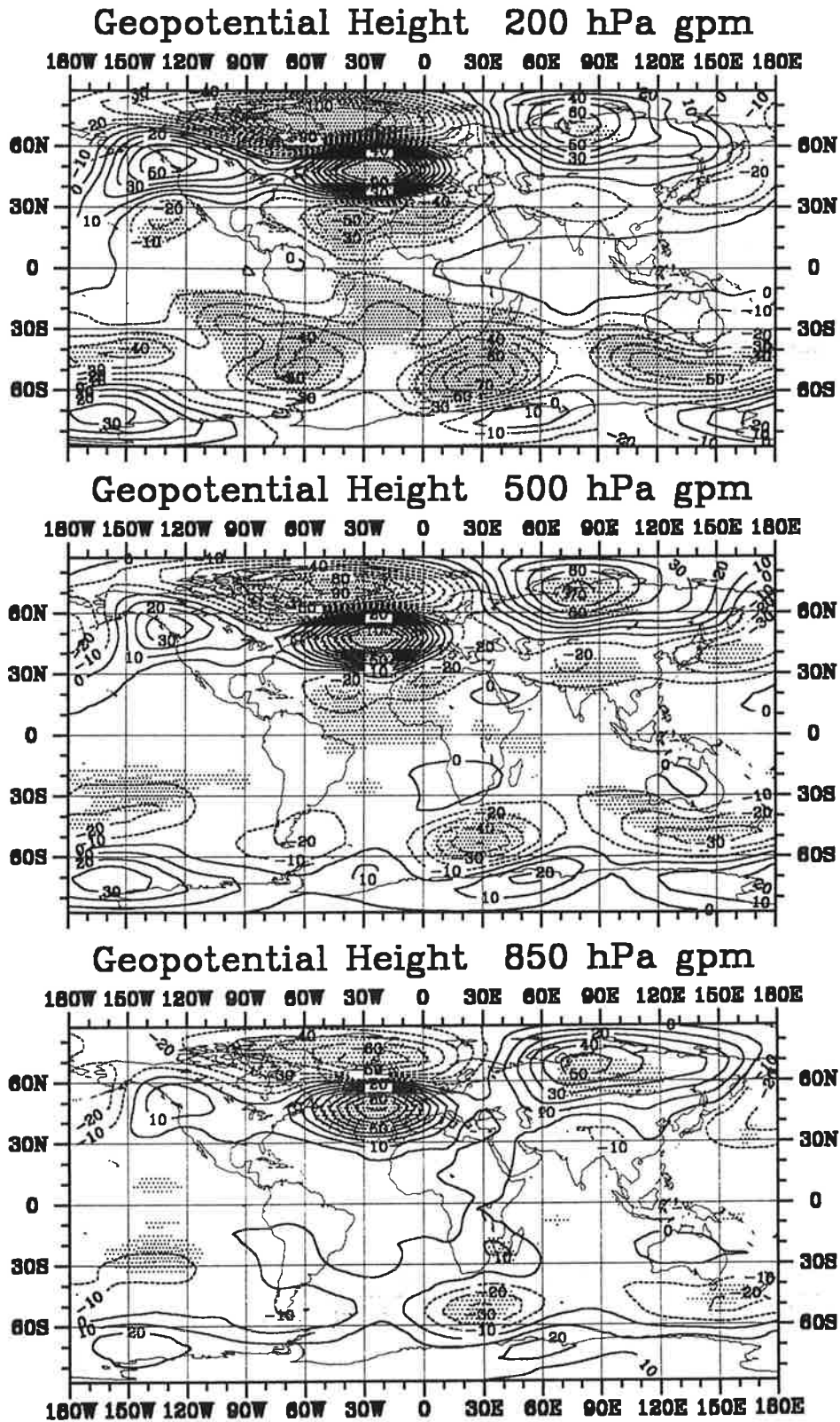
Figure 7: Anomalies of the geopotential height at different tropospheric levels. Shading indicates statistically significant (error chance 5%) differences between Control and Experiment for months 31 to 60 on the basis of a local t-test, degrees of freedom reduced to 15.
