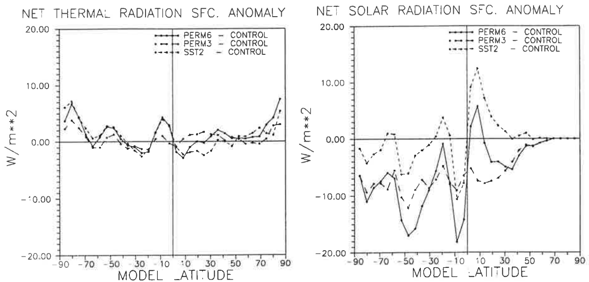
Figure 4: Net anomaly [ W/m^2 ] at the surface for thermal (Fig. 4a) and solar (Fig. 4b) radiation for different Permanent January Experiments. PERM3 is the actual volcano experiment. SST2 is forced by tropical sea surface temperature anomalies as observed in January 1983, and PERM6 is a combination of volcanic and SST forcings.
