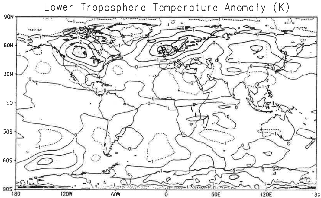
Figure 11: Anomaly of the air temperature near surface [K] as observed December 1991 through February 1992 from MSU satellite data (Spencer and Christy, 1991), Anomalies calculated from mean for 1982-1990.
