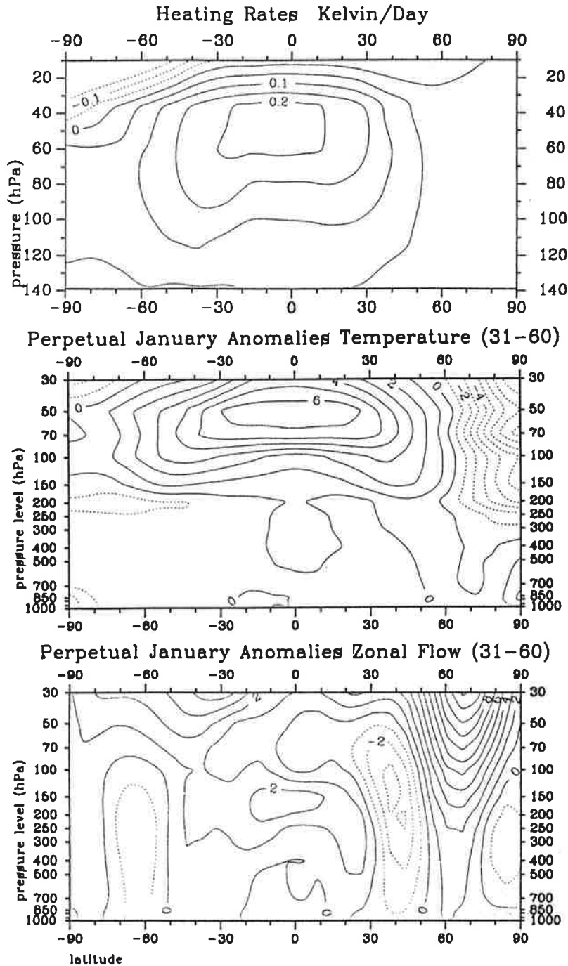
Figure 3: Cross sections of the zonal mean values of: a) Heating rate anomalies [K/d], as determined from the radiative transfer model for January 1983 or 1992 (top). b) Temperature anomalies [K] for Perpetual January Experiment (month 31 to 60) minus Control (middle). c) Zonal wind anomalies [m/s] for Perpetual January Experiment minus control (month 31 to 60) (bottom).
