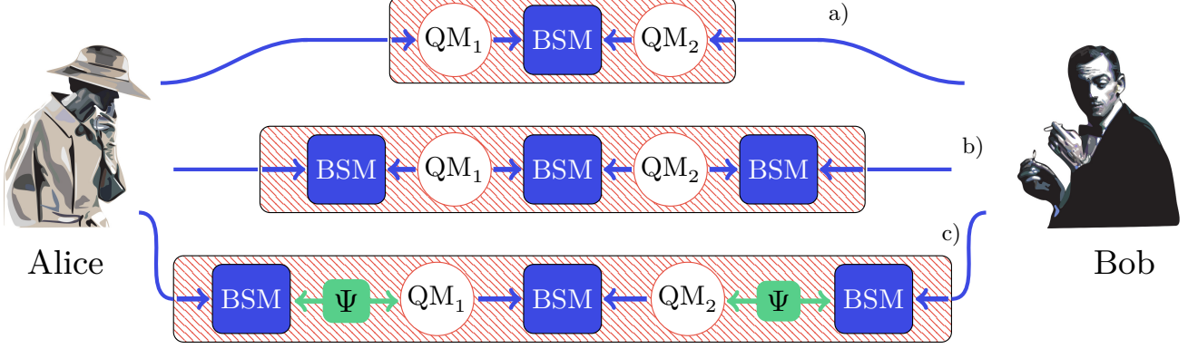
FIG. 13. Three different setups for the memory-assisted measurement-device-independent quantum key distribution (MA-MDI QKD). Here, BSM stands for Bell state measurement. The first setup a) corresponds to the scheme of MA-MDI QKD with direct heralding. Specifically, the implementation of this setup requires that a photonic state can be transferred into a quantum memory QM_1 and QM_2 in a heralded fashion. That is, following the transfer attempt, one obtains the information whether the state of the photon emitted at Alice or Bob has been successfully transferred to the desired quantum memory. The second setup b) with indirect heralding is a modification of the first one. Here the requirement of the heralded state transfer has been dropped, at the cost of probabilistic Bell state measurements between two photonic qubits at the outer BSM stations. Finally, the setup in c) is a modification of b), which uses sources of entangled photons ( \Psi ). In this way, the attempt to transfer the quantum state of the photon into the memory is performed only after a successful Bell state measurement. This can increase the rate per unit time, since writing unto and resetting the memory is a time-consuming process.
