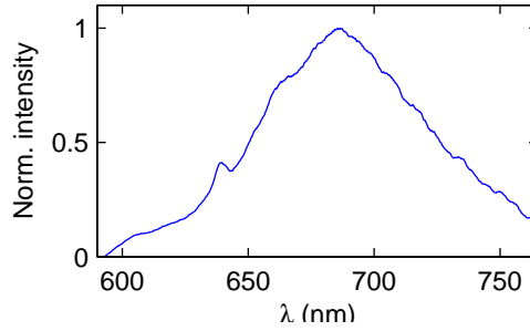
Figure 7.1.: Spectrum of the NV center at room temperature
