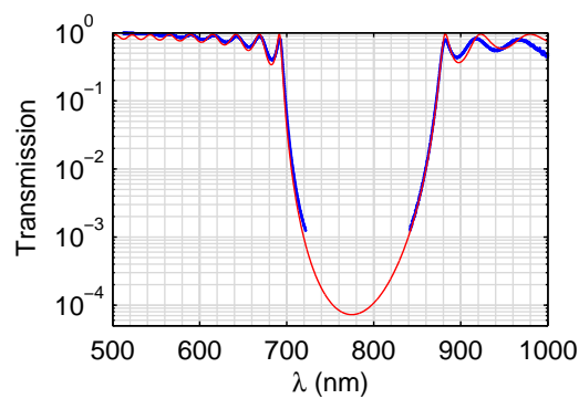
Figure 5.17.: Layertec coating: Measured (blue dots) and simulated (red line) mirror transmission.
