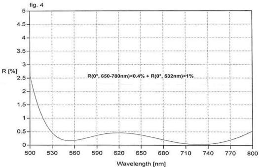
Figure 5.18.: Layertec coating manufacturer specifications.
