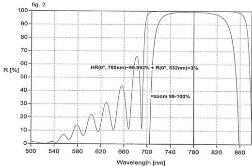
Figure 5.18.: Layertec coating manufacturer specifications.
