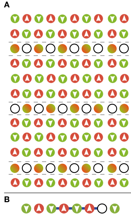
Figure 7.1. Striped phase. (A) Illustration of stripes of holes in AFM background at 1/8 doping as found in (La_{1.28}Nd_{0.6}Sr_{0.12})CuO_4 [201]. The holes are mobile along the horizontal stripes forming 1d-subsystems with spin-charge separation. The two-colored circles are spins, which are aligned along the horizontal direction but not along the vertical direction due to their delocalization. (B) In a one-dimensional AFM background a hole can move without energy cost as indicated by the blue track of the hole.
