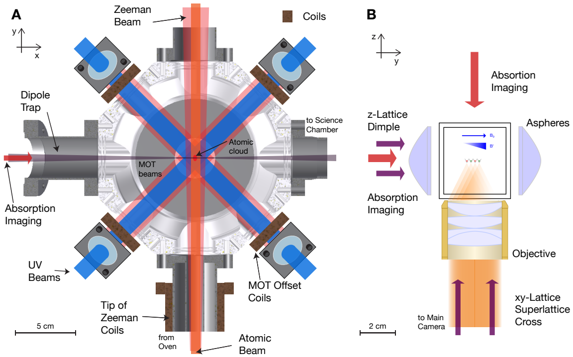
Figure 3.2. Overview MOT and Science chamber. (A) MOT chamber seen from top with its most important elements. MOT coils (not shown) are horizontal. (B) Science chamber (glass cell) seen from front with high-resolution lenses. The main images are taken by collection of fluorescence light through the objective. Absorption images are only used for characterization of the cooling steps.
