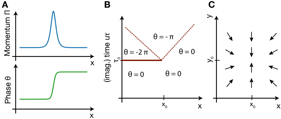
Figure A.2. Vortex in the Luttinger liquid A A localized momentum (top) is associated with a kink in the phase \theta_\rho . B A momentum kick e^{i2\phi_\rho} at time \tau_0 and position x_0 thus changes the phase \theta_\rho = 0 by -2\pi for x < x_0 . The excitation spreads with time, leading to a winding of the phase \theta_\rho around (x_0, \tau_0) . Such momentum kicks are generated by umklapp scattering events in a lattice, when two particles with quasi momenta q_1, q_2 scatter into q_3, q_4 with \sum_i q_i = Q , where Q is a lattice momentum. These processes drive the system into a Mott insulator. C The \theta_\rho -vortex is topologically equivalent to a vortex in a classical spin XY-model, so the Mott transition in one-dimension is in the universality class of the BKT-transition [54].
