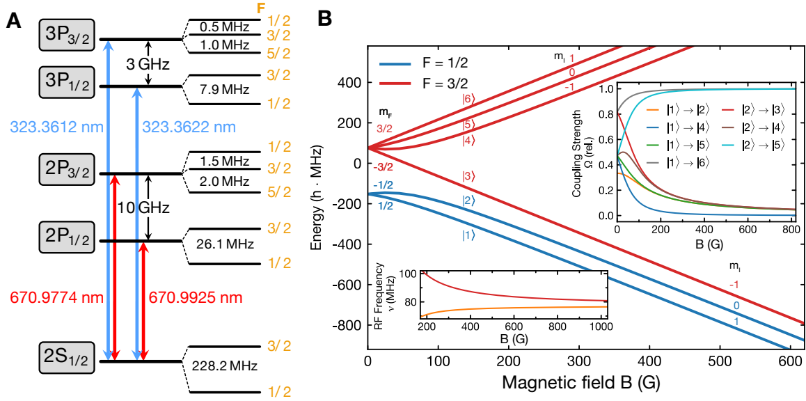
Figure 3.3. States of {}^6\text{Li} . (A) The 2S , 2P , and 3P states with fine and hyperfine structure and their splittings. Image taken from [89]. (B) Breit-Rabi diagram of {}^6\text{Li} with the Zeeman regime on the left ( F -Basis) and the Paschen-Back regime on the right ( JI -Basis). Left inset shows the energy splitting of the three lowest states, which approach \sim (2\pi\hbar) \cdot 80\text{ MHz} at high magnetic fields. Right inset shows the transition strength (Rabi frequency) for magnetic RF transitions between states of the 2S manifold normalized to a pure electron rotation i.e. |m_J, m_I\rangle \rightarrow |m_J + 1, m_I\rangle . At high magnetic field the coupling between the |1\rangle, |2\rangle , and |3\rangle state become very small.
