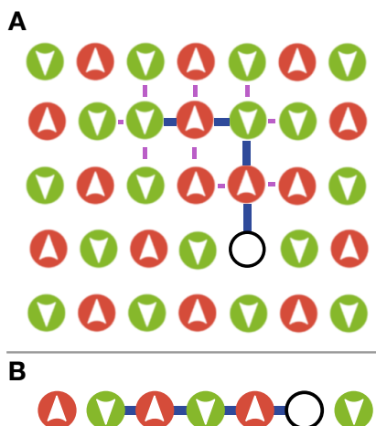
Figure 1.2. Hole propagation in AFM background. (A) In two dimensions, the propagation of a hole along some path (blue line) produces a string of flipped spins with an associated energy cost. Broken bonds are indicated in purple. (B) In one dimension, a hole is free to propagate through an AFM spin chain without an energy cost.
