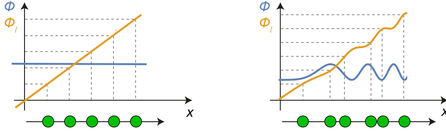
Figure A.1. Luttinger labeling field. Illustration of the labeling fields \phi_l(x) and \phi(x) . For crystallized particles \phi_l(x) grows linearly and \phi(x) is constant. Different functions allow to describe any particle distribution. Note that density fluctuations are proportional to the gradient of \phi , (\rho(x) - \rho_0) \sim -\nabla\phi(x) .
