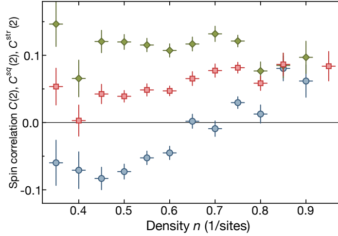
Figure 7.12. Comparison of spin correlations. Spin correlation C(d = 2) in blue, spin string correlations C^{str}(d = 2) in green and squeezed space correlations C^{sq}(\tilde{d} = 2) in red as a function of local density.
