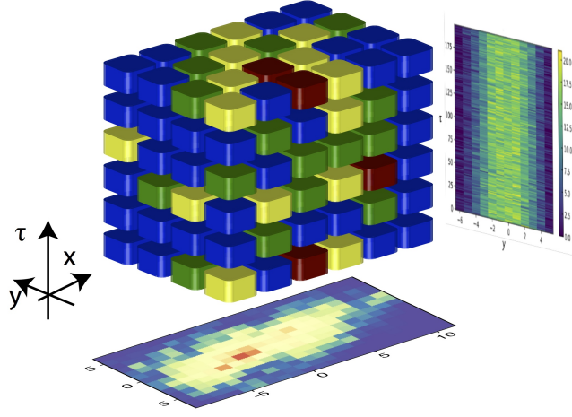
Figure 6.1. Cube of data. Illustration of the raw data consisting of holes (blue), spin ups (yellow), spin downs (green) and doublons (red) on every site of the lattice (x,y) and on every image (\tau) . Averaging of the density along \tau gives the mean density (bottom) and along x gives the atom number per chain per shot (right).
