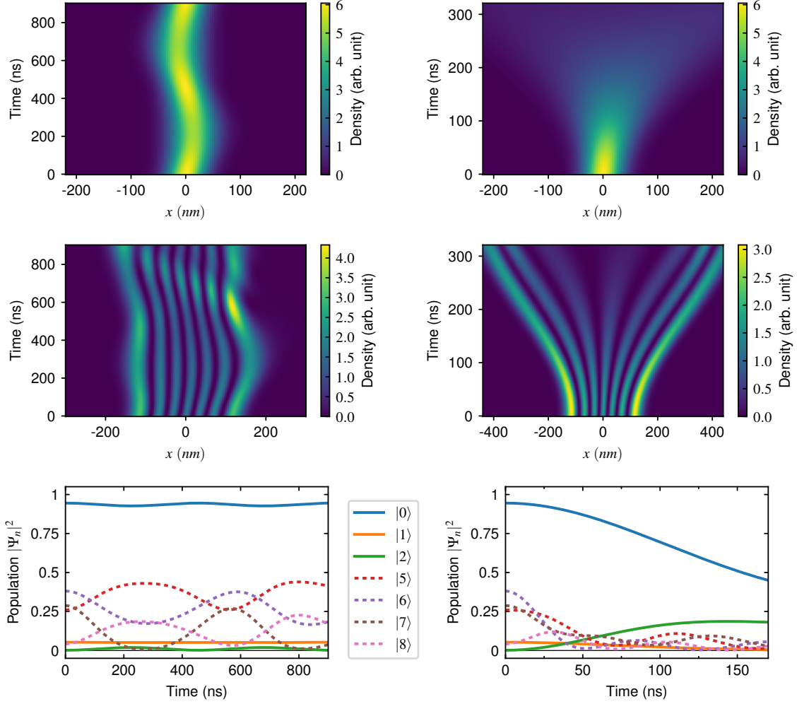
Figure 4.6. Time evolution of the P-state. A ground state atom starting in an h.o. eigenstate n = 0 ( first row ) or n = 6 ( second row ) absorbs a photon a time t = 0 and is excited to the P state. In a 1064 nm lattice for lithium ( first column ) the optical potential is only 25% weaker than in the ground state. The time evolution of the real space density |\Psi_n(x)|^2 mainly reflects the momentum kick by the photon and shows a weak breathing due to the changed trap frequency. The evolution of the overlap with the S-state h.o. eigenstates ( bottom row ) shows how much stronger the levels mix for the initial n = 6 state (dashed) compared to n = 0 case (solid). The distribution at t = 0 is due to the recoil of the absorbed photon and the lifetime in the P-state is 27.1 ns. The second column shows the dramatic effect if the P-state potential is the inverse of the S-state potential (near resonant case). The unbound wave function rapidly expands and is even accelerated outwards, causing large heating in such a lattice.
