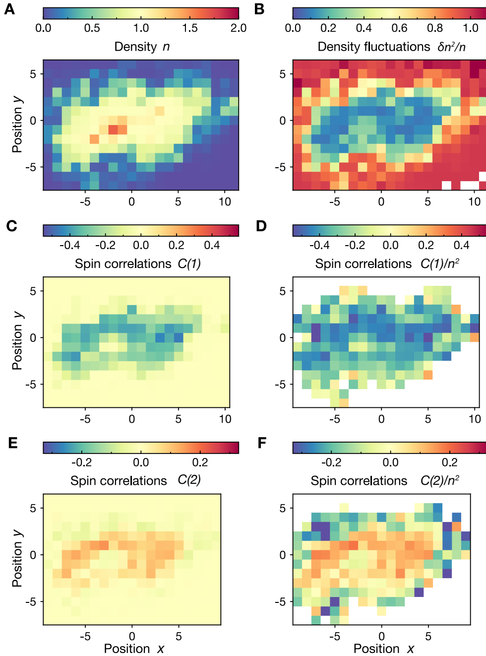
Figure 6.12. Overview of density and spin correlations. The spatial distributions of (A) the local density n_r , (B) the on-site density fluctuations \delta n_r^2/n_r^2 , (C) the bare nearest-neighbor spin correlations C_r(d_x = 1) and (D) these normalized to (singlon) density squared C_r(d = 1)/(n_r^s)^2 , (E) the bare next-nearest-neighbor spin correlations C_r(d = 2) and (F) these normalized to density squared C_r(d = 2)/(n_r^s)^2 . The region of the Mott insulator with density one (yellow in A) and low density fluctuations (blue in B) shows the strongest spin correlations (C,E). After normalization to density (D,F), larger regions show strong correlations demonstrating that spin correlations exist in the doped regime. White areas do not have sufficient statistics to display a result.
