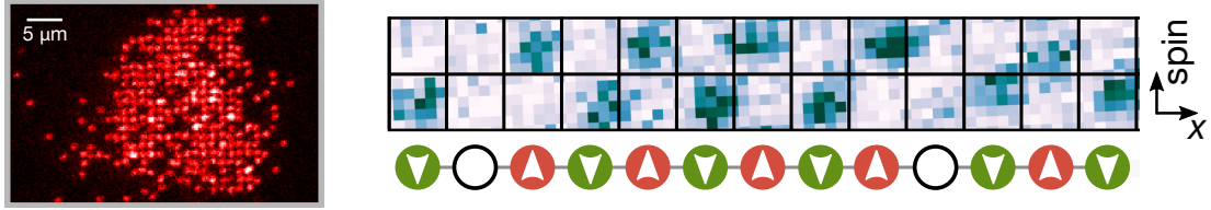
Figure 1.1. Images of individual atoms in a quantum many-body state. Left: Image of {}^6\text{Li} atoms in an optical lattice. Every red dot is one atom. Right: Zoom into a one-dimensional chain of atoms imaged with spin encoded in the vertical position showing antiferromagnetic order and holes.
