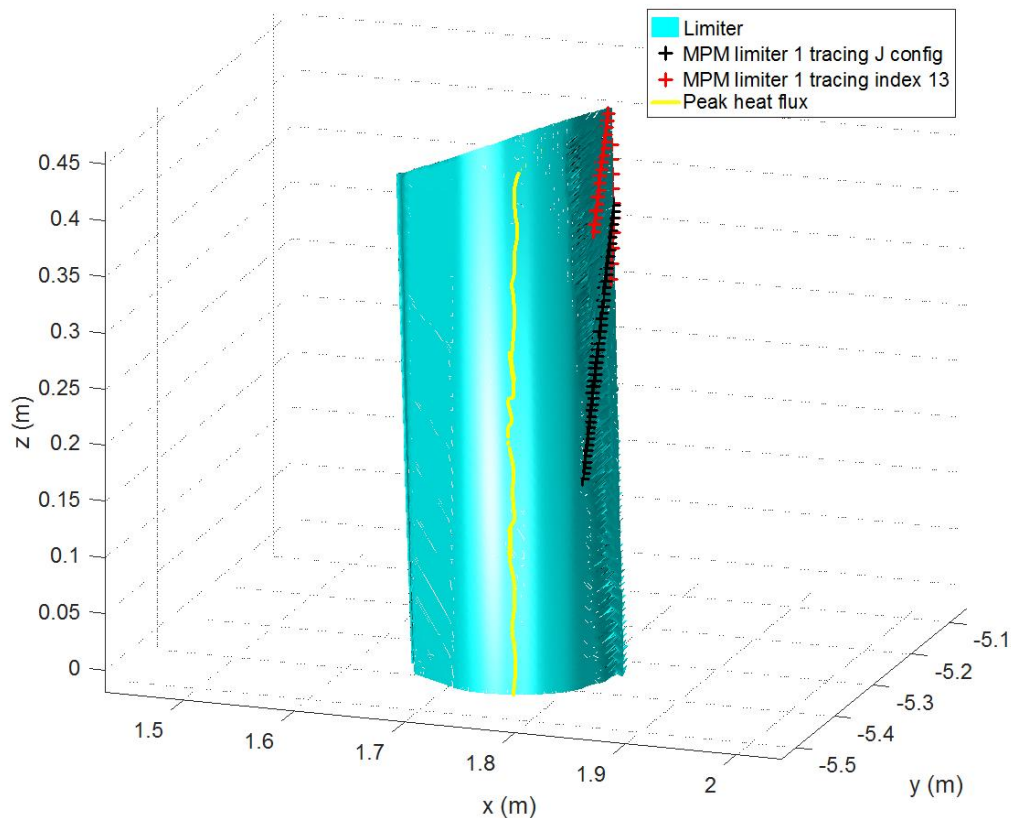
Figure 7 shift of the footprint of the combined probe mapped on the limiter in backward direction, black: limiter J-configuration, red: iota index 13 configuration
