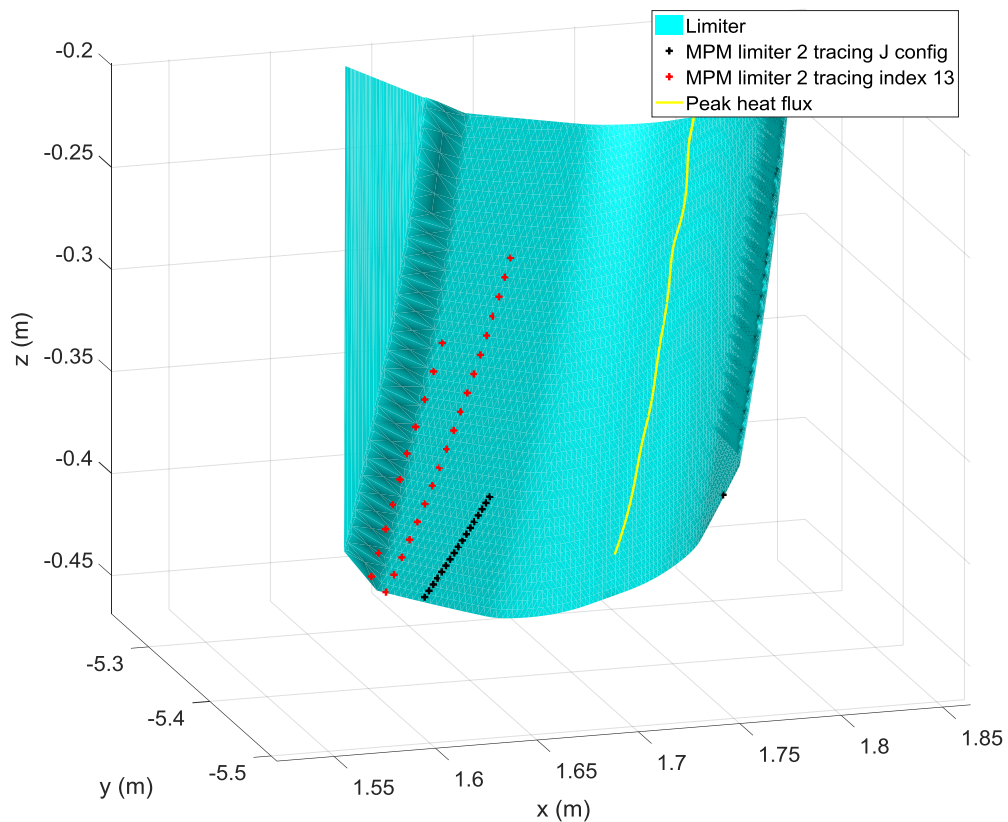
Figure 6 shift of the footprint of the combined probe mapped on the limiter in forward direction, black: limiter J-configuration, red: iota index 13 configuration
