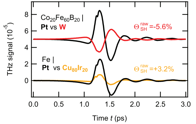
Figure 5. Comparison of THz-emission raw data from Pt, W, and \text{Cu}_{80}\text{Ir}_{20} . THz waveforms emitted from FMINM structures where NM is W (red) and \text{Cu}_{80}\text{Ir}_{20} (orange) in comparison to a FMI Pt reference structure with the same layer thicknesses (black curves). The values of \Theta_{SH}^{raw} indicate the spin Hall angles of the respective NM materials estimated by calculating the ratios of the bare THz-signal amplitudes (RMS) and assuming a spin Hall angle of 12.0% for the Pt reference.
