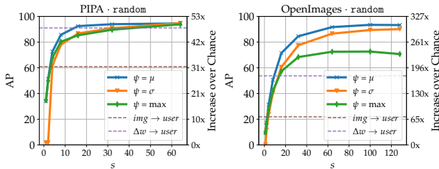
Figure 8: Effect of aggregation on image-classification task. s is the size of the aggregated image set and \psi is the aggregation strategy.
