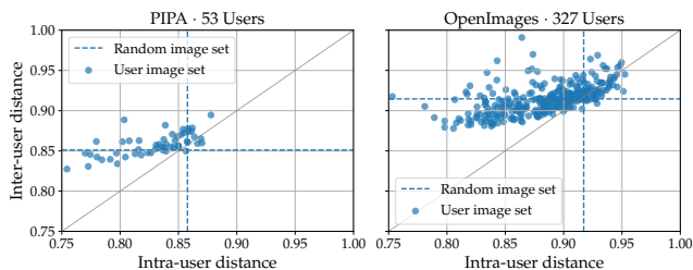
Figure 3: Distinctiveness of users data. Each point represents distances computed over the images of a single user.
