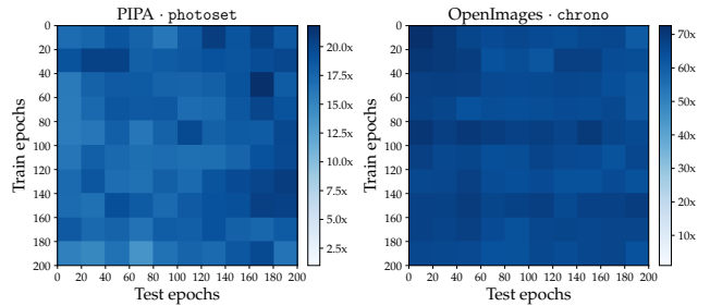
Figure 9: Effect of the epoch t on the identification attack \Delta w_i^t \rightarrow u_i . For instance, the top-right cell denotes when the MLP was trained on updates \Delta w_i^t, t \in [0, 20] and evaluated on \Delta w_i^{t'}, t' \in [180, 200]
