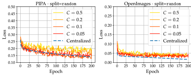
Figure 4: Training Loss of FedAvg obtained by varying C , the fraction of clients sampled each round
