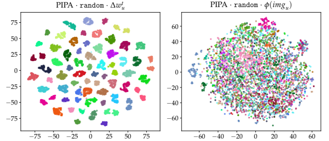
Figure 7: t-SNE visualization of model updates \Delta w_i (left) and images x_i (right). Colors indicate users.
