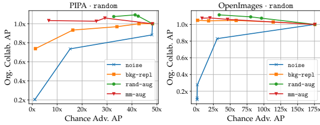
Figure 11: Mitigation strategies against closed-world identification MLP attack. Top-left is the ideal region.
