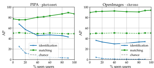
Figure 10: Open-world evaluation across both identification and matching attack models.
