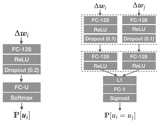
(a) MLP model for Identification Attack (Section 6.1)
