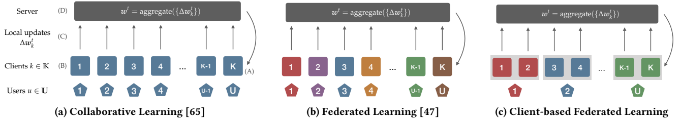
Figure 1: Learning from decentralized data visualized w.r.t to client’s data distribution. Colors of clients and users indicate their data distribution.
