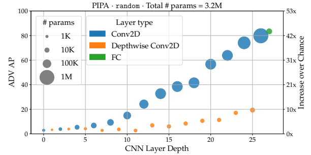
Figure 5: Identification performance by depth. Bubble sizes indicate the number of parameters in each layer. Last two layers contains 1M and 19K parameters respectively.
