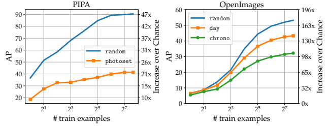
Figure 6: Adversary’s MLP identification attack performance w.r.t # of examples per user used to train
