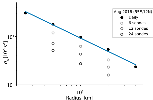
FIG. 10. Comparison of day-to-day variability in D (closed circle) with estimates of its measurement error as a function of circle radius and as estimated using 6, 12, or 24 sondes (open circles). Variability in D is quantified by the vertical average of the temporal standard deviation of D with height. Error is quantified by vertically averaging the RMSE. In all cases the vertical averaging is over the lower troposphere, defined as the layer between the surface and 5 km.
