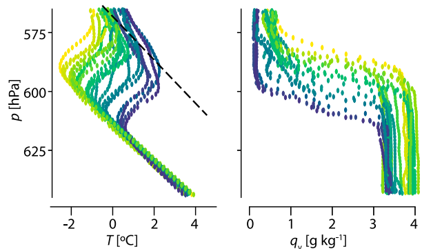
FIG. 8. (left) Temperature and (right) specific humidity in a roughly 1\text{-km} -deep layer (between 650 and 560 \text{ hPa} ) about the melting level for the sondes launched during C1 and C2 of RF03. Individual soundings are colored by the height of the 2 \text{ g kg}^{-1} specific humidity isosurface, which systematically descends from the east (where it is highest) to the west, across the circle. The dashed line shows the slope of a dry adiabatic temperature profile.
