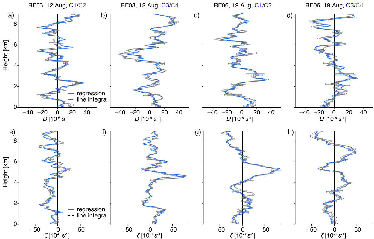
FIG. 4. Vertical profiles of (a)–(d) large-scale mass divergence and (e)–(h) vorticity estimated from the dropsonde wind measurements performed during (a),(b),(e),(f) RF03 (12 Aug) and (c),(d),(g),(h) RF06 (19 Aug) along each circular flights (the first circle is in blue, and the second one is in gray), using either the regression method (solid line) or the line integral method (dashed line). Horizontal bars represent plus and minus one standard error of the regression estimate, and for the sake of clarity, they are shown at selected vertical levels only.
