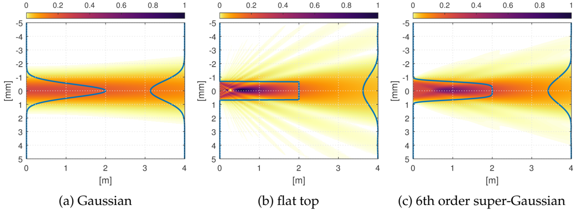
Fig. 2.1: Diffraction effects for different beam profiles. Direction of propagation is along the x -axis, lateral size of the beam is along the y -axis. Propagation is simulated in 3D with monochromatic beams ( \lambda=800 nm). Plotted lines show the near-field and far-field intensity distribution (cross section through the center of the beam). Colors indicate the intensity distribution during propagation.
