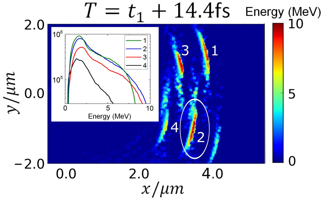
Figure 4.29: Almost at the end of the second step after approximately \geq 3 - 4\mu\text{m} of propagation, which corresponds to the simulated Rayleigh length ( 4.4\mu\text{m} ), at T = t_1 + 14.4\text{fs} the electrons gained extra 5 MeV. \varphi_{\text{CEP}} = 0.9\pi .
