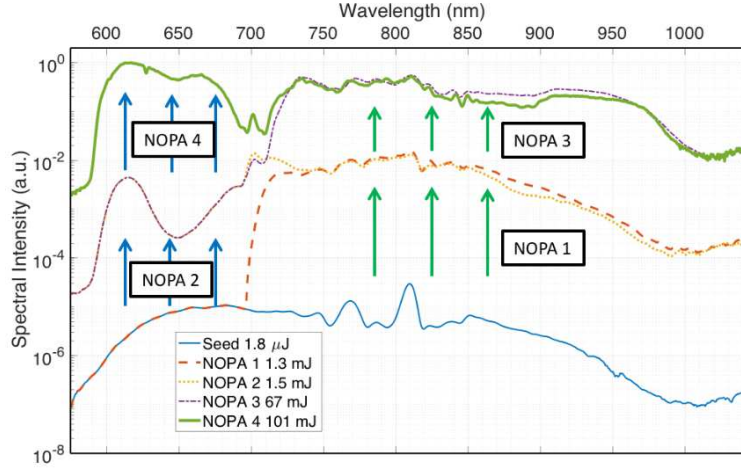
Figure 1.3: Two-color-pumped sequential amplification, spanning a spectrum from 580 to 1020 nm with an energy of about 100 mJ. Figure obtained from [158].
