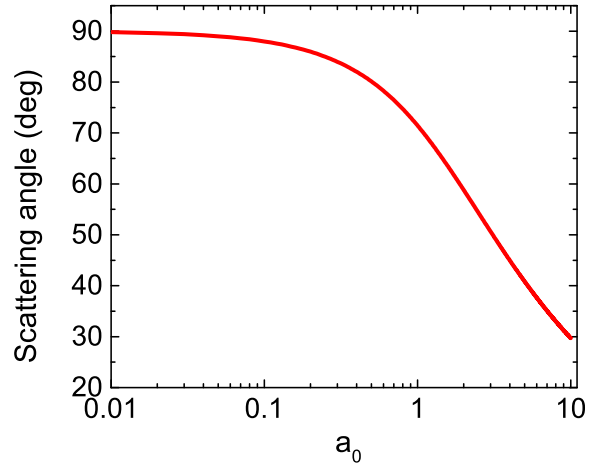
Figure 2.5: Scattering angle as a function of the normalized laser vector potential a_0 , calculated from Eq.(2.26) without cycle averaging for \beta_0 = 0 .
