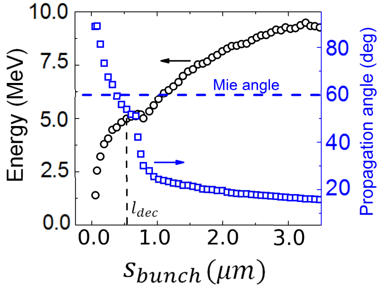
Figure 4.27: Energy and propagation angle evolution of the electrons as a function of the bunch distance from the target surface s_{bunch}
