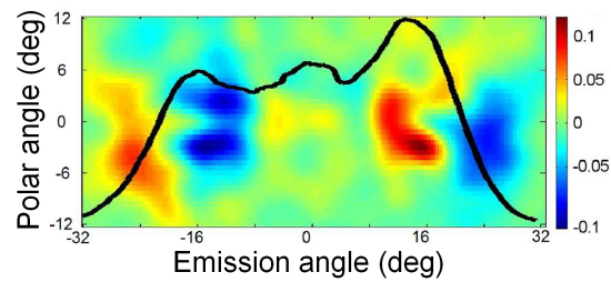
Figure 4.33: 2D asymmetry in angular distribution and 1D integrated distribution along the polar angle (black line) from 3D PIC simulations. Mind the different color bars.
