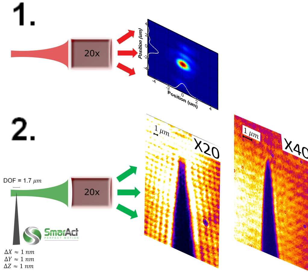
Figure 4.11: Alignment of each target. First step: scan the long-working distance objective position until the laser spot position is at its minimum size (image plane), then proceed to mark the laser spot (maximum) position. Second step: keeping the objective's position fixed and the laser blocked, the target is positioned with 1 nm accuracy to match the marked laser position vertically and horizontally. Finally, the longitudinal axis is scanned and the needle position is set equidistant to the positions z_1 and z_2 , where the image becomes blurry (out of focal plane).
