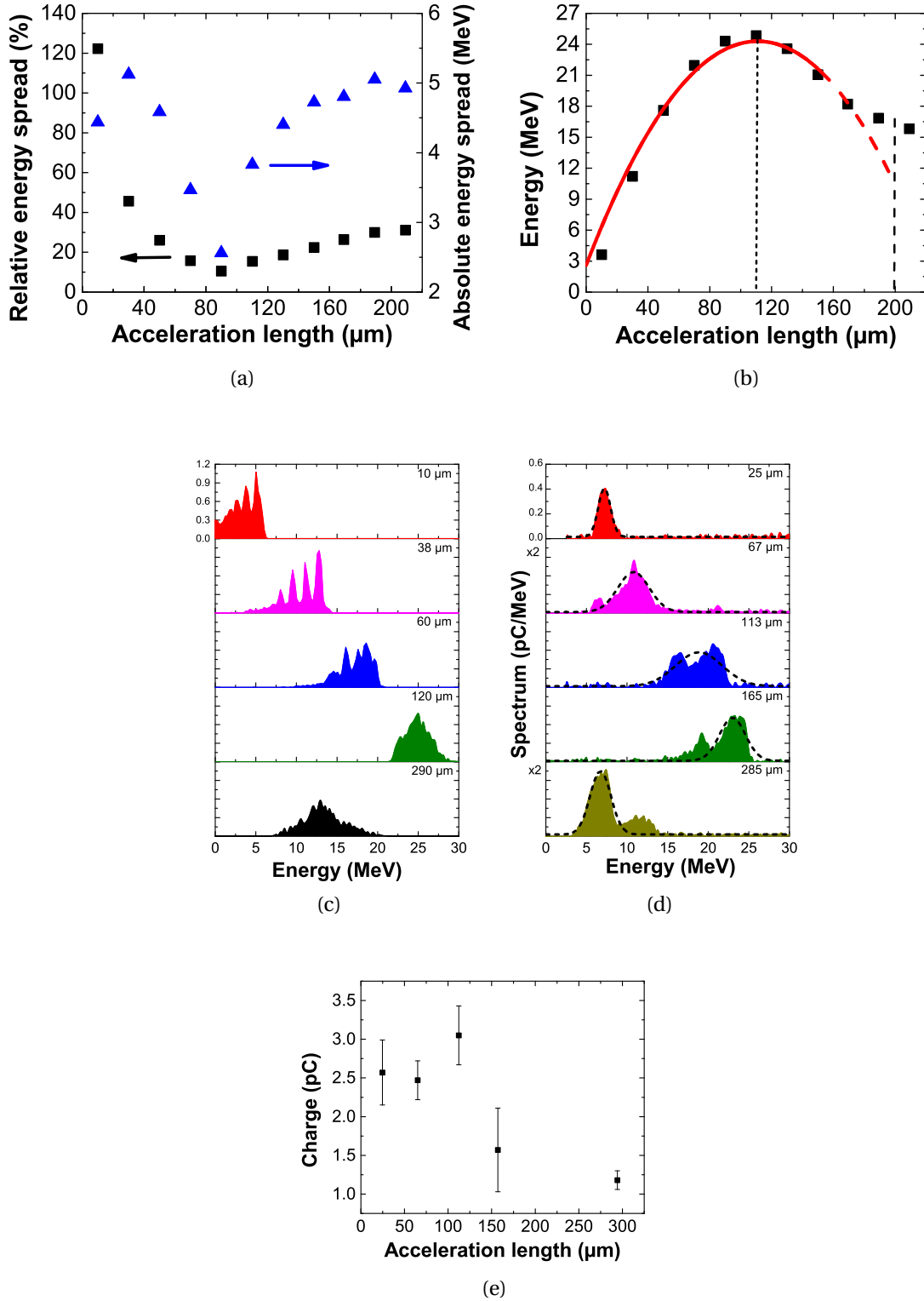
Figure 3.21: (a), (b) and (c) Simulation results of a wakefield excited by an 8-fs laser pulse with a normalized electric field of a_0 = 0.75 at a density of 4 \times 10^{19} \text{cm}^{-3} (d) Typical experimental shots for different acceleration lengths, labeled on the top-right corner; (e) Measured averaged charge as a function of the acceleration length.
