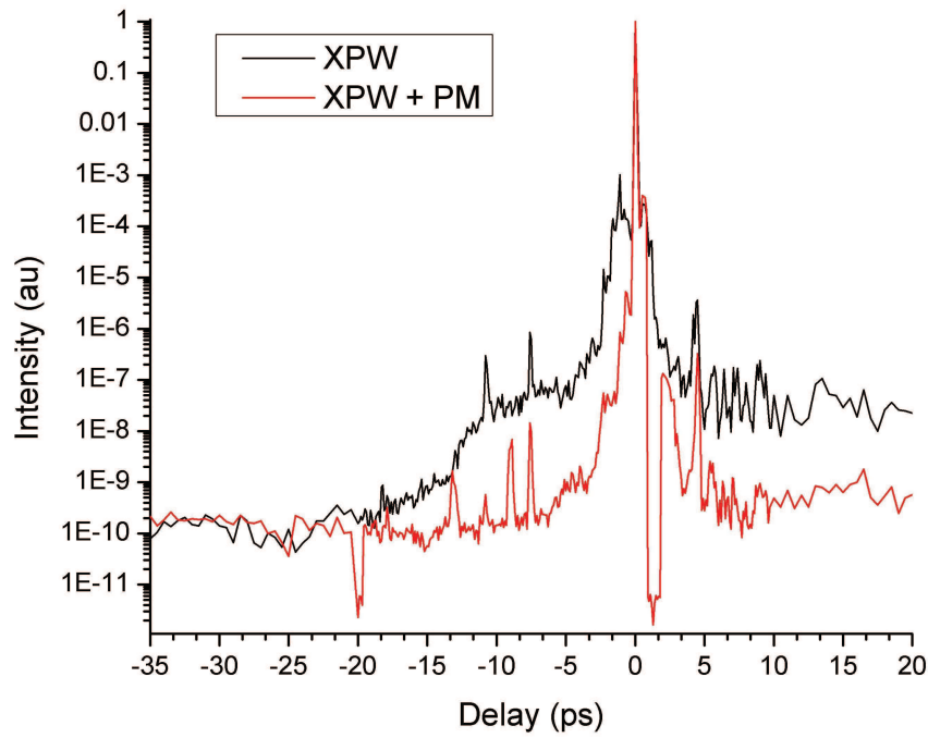
Figure 1.5: LWS-20's high-dynamic temporal intensity contrast by implementing XPW or XPW and subsequent PM. Figure obtained from [128].
