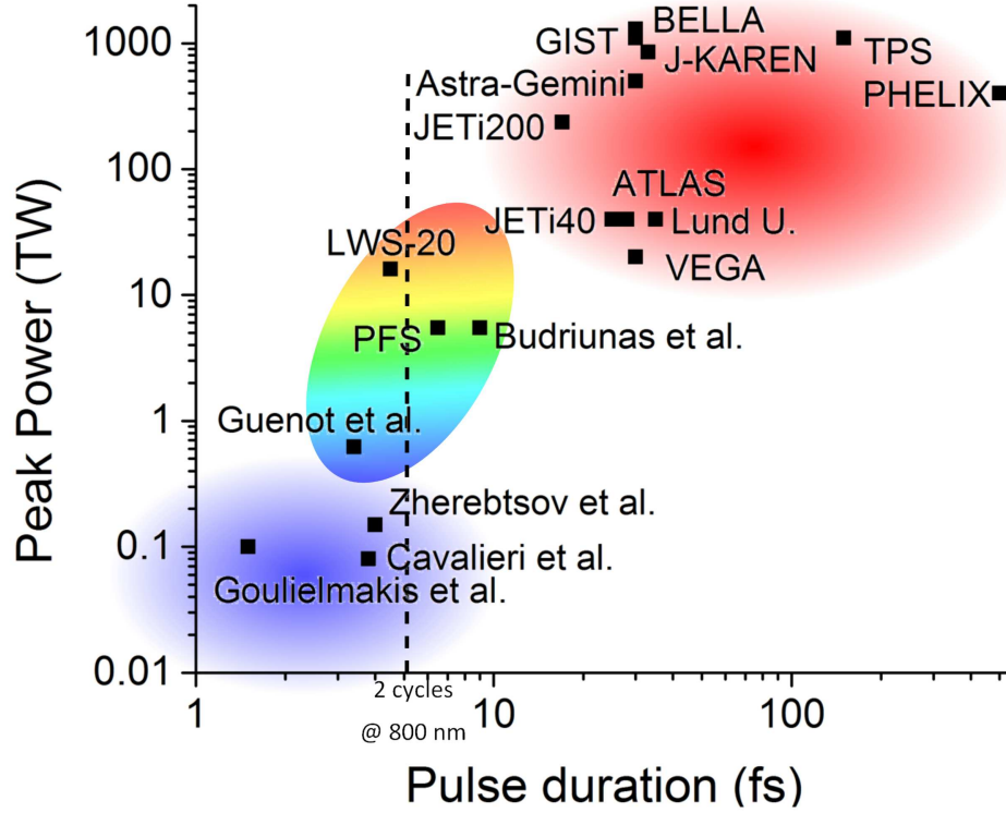
Figure 1.1: Laser scenario in 2017. Typical laser systems corresponding to relativistic plasma physics are highlighted in red: ATLAS [14], Lund Laser Center (LLC) [35], 20 TW VEGA system [129], JETi200 [75], Astra-Gemini [70], the Petawatt system at the Gwangju Institute of Science and Technology [80], the BELLA project [88], the J-KAREN system [3], the Texas Petawatt System (TPS) [52] and the PHELIX laser [4]. Find a complete review on Petawatt lasers in [32]. Some examples of few-cycle sub-mJ laser systems working in the attosecond field are marked in blue: Cavalieri et al.[20], Zharebtsov et al.[167] and down to single-cycle regime from Goulielmakis et al.[59]. Single-cycle pulses with higher energies (mJ-level) are becoming available as well, as reported by Guénot et al.[60]. Finally, few-cycle multi-10 mJ lasers such as: the Petawatt-Field Synthesizer (PFS) [78] and the work of Budriunas et al. [16], together with the sub-2 cycle LWS-20 [158] used in this thesis, fill the gap between these research areas. As observed in the figure above, the LWS-20 is the few-cycle most powerful laser in the world.
