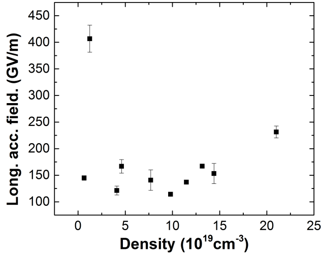
Figure 3.17: Measured longitudinal accelerating field for different densities. The two data points at the lowest densities correspond to the [29, 120].
