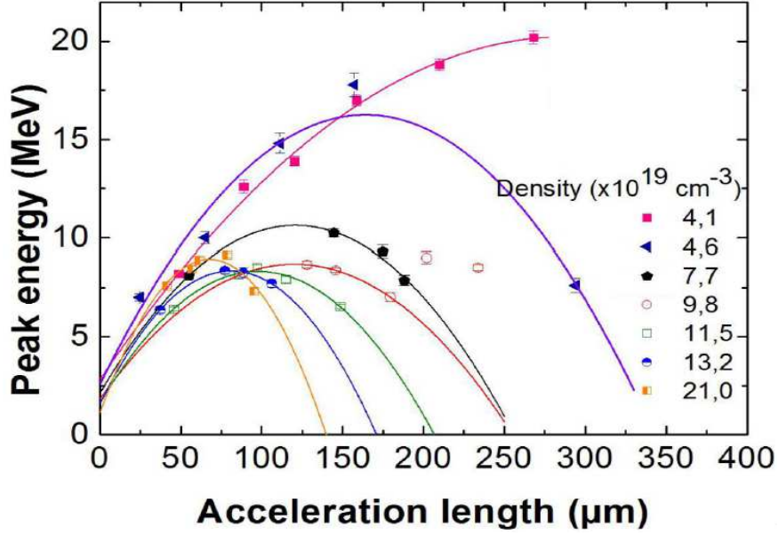
Figure 3.13: Peak energy of the electron spectrum for sub-10-fs laser pulses vs. acceleration lengths for various electron densities. The error-bars indicate standard error over 50 shots. The lines are fits using Eq.(3.24).
