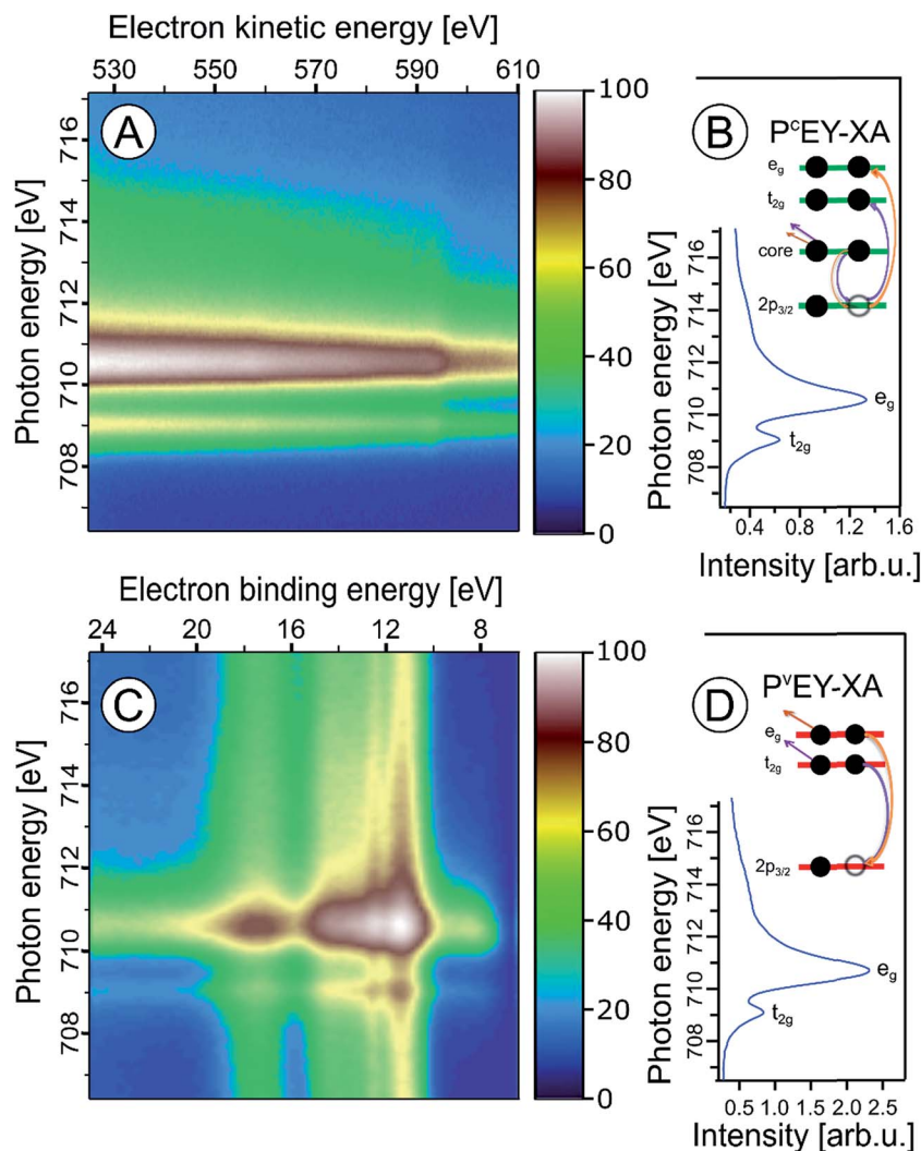
Fig. 6 Fe 2p 3/2 resonant photoelectron spectra from 10 wt% \alpha -Fe 2 O 3 NPs in 0.1 M HNO 3 aqueous solution, covering the 2p-3p 3/2 (A) and 2p-3d 3d (C) Auger-electron emissions after Fe 2p 3/2 \rightarrow t 2g and 2p 3/2 \rightarrow e g excitation, respectively. Spectra were recorded for photon energies between 707 and 716 eV. The respective P C EY- and P V EY-XA spectra, and illustrations of the relevant energies, excitations and the relaxation channels are displayed in (B) and (D).
