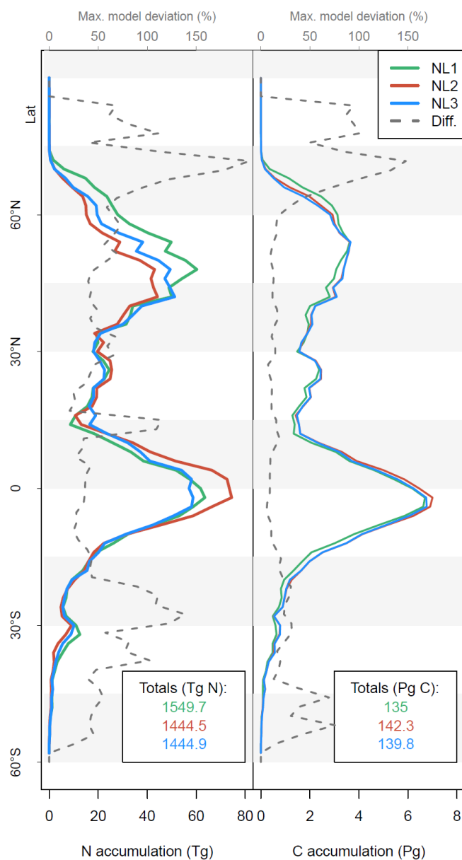
Figure 5: Nitrogen (N, left) and carbon (C, right) accumulation during global simulations of elevated atmospheric CO 2 concentrations (eCO 2 ) using three different N loss algorithms between 1850 (285 ppm CO 2 ) and 2100 (936 ppm CO 2 ), depicted per 2° latitudinal band and as global totals (coloured numbers). "Diff." shows the respective maximum deviation between the three models as the percentage of the three model mean. The global total values corresponded to average yearly accumulation of: 6.20, 5.78, 5.78 Tg N yr -1 ("NL1", "NL2", "NL3") and 0.54, 0.57, 0.56 Pg C yr -1 .
