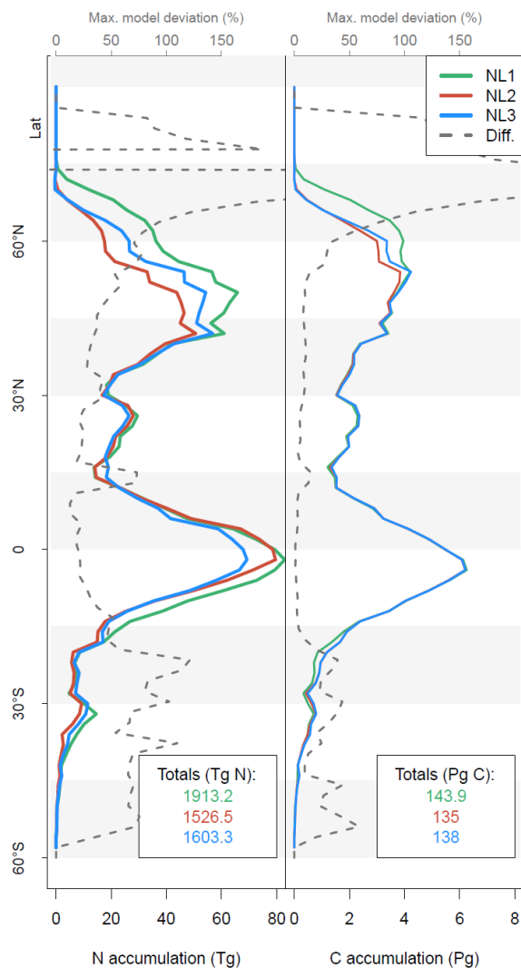
Figure A1: Nitrogen (N, left) and carbon (C, right) accumulation during global simulations of elevated atmospheric CO 2 concentrations (eCO 2 ) using three different N loss algorithms between 1850 (285 ppm CO 2 ) and 2100 (936 ppm CO 2 ), depicted per 2° latitudinal band and as global totals (coloured numbers). "Diff." shows the respective maximum deviation between the three models as the percentage of the three model mean. The global total values corresponded to average yearly accumulation of: 7.65, 6.11, 6.41 Tg N yr -1 ("NL1", "NL2", "NL3") and 0.58, 0.54, 0.55 Pg C yr -1 . The difference to Fig. 5 was the usage of an O-CN terrestrial biosphere model version that employed fixed C:N stoichiometry in all soil and vegetation pools (Meyerholt and Zaehle, 2015).
