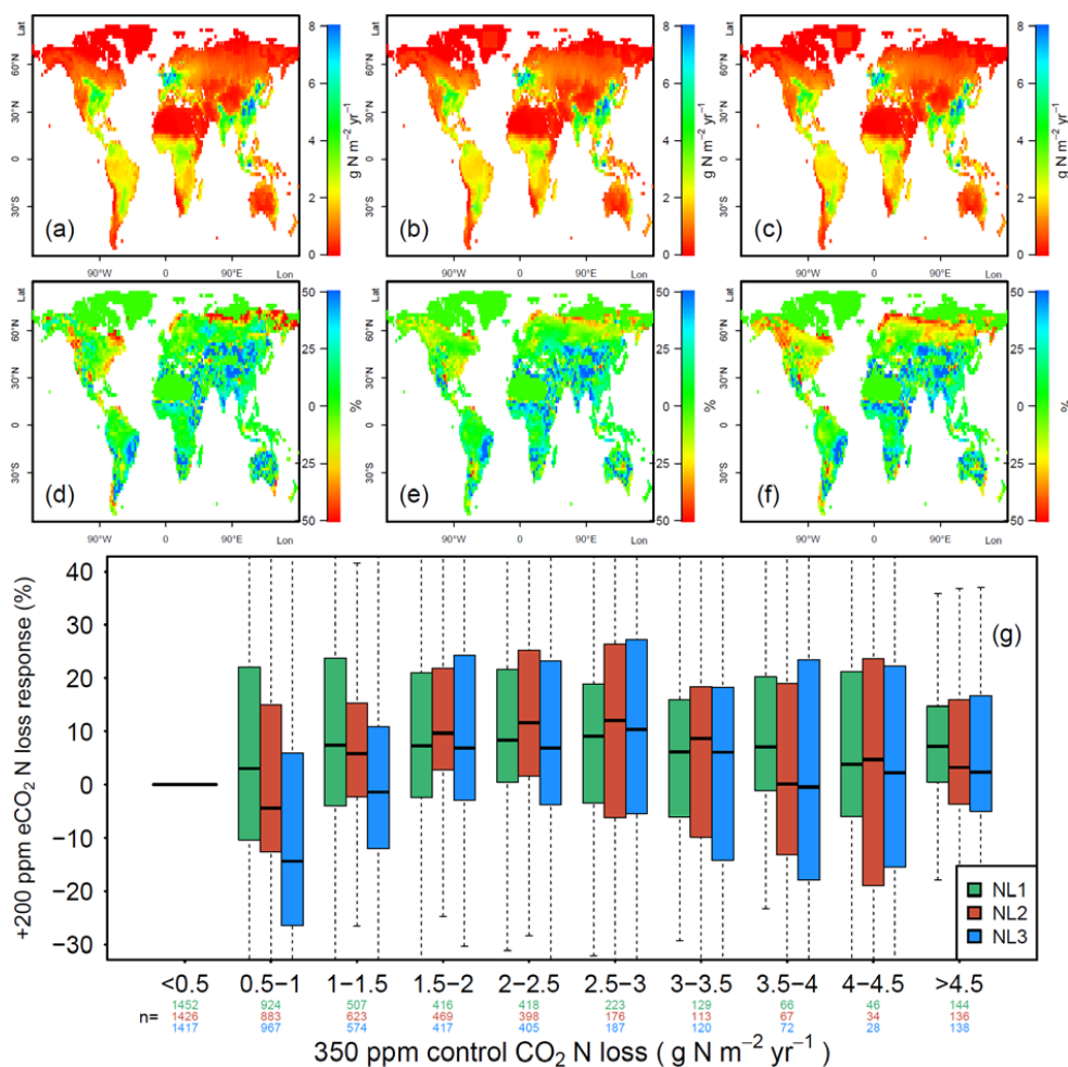
Figure A2: (a), (b), (c): Global nitrogen (N) loss rates ( \text{g N m}^{-2} \text{yr}^{-1} ) for the control runs (350 ppm atmospheric \text{CO}_2 concentration), using the N loss algorithms "NL1" (a), "NL2" (b), and "NL3" (c). (d), (e), (f): Global N loss responses (%) to elevated atmospheric \text{CO}_2 concentrations ( \text{eCO}_2 , +200 ppm). (g): Global response ratios (%) plotted against the corresponding control N loss rates, binned in intervals of 0.5 \text{ g N m}^{-2} \text{yr}^{-1} . Boxes show median and quartiles, whiskers show the largest/smallest outliers that lie below/above 1.5 times the interquartile range. Further outliers were omitted. Coloured numbers indicate the number of 2^\circ \times 2^\circ grid cells that fell into the respective N loss range. The 350-550 ppm difference in atmospheric \text{CO}_2 concentrations approximately corresponded to the 1988 - 2052 time span in our global simulations. The difference to Fig. 4 was that these simulations also included transient climate and N deposition rates according to the RCP8.5 scenario.
