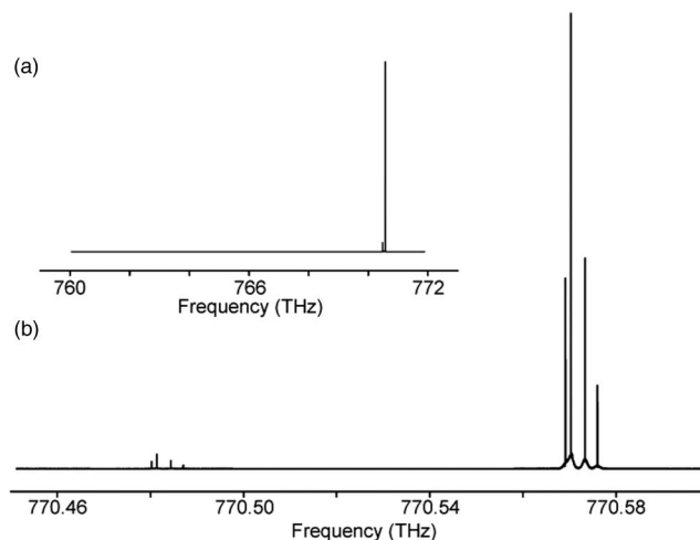
Fig. 3. Experimental dual-comb two-photon spectra of the sub-Doppler hyperfine transitions of ^{85}\text{Rb} and ^{87}\text{Rb} . (a) The span is broader than 10 THz. (b) The lines around 770.48 THz are assigned to the 5S_{1/2} - 5D_{3/2} transitions, and those around 770.57 THz are assigned to the 5S_{1/2} - 5D_{5/2} transitions.
