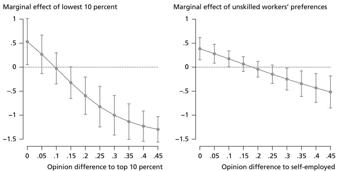
Figure 4 Marginal effect of low-income and unskilled workers' opinions on policy change
