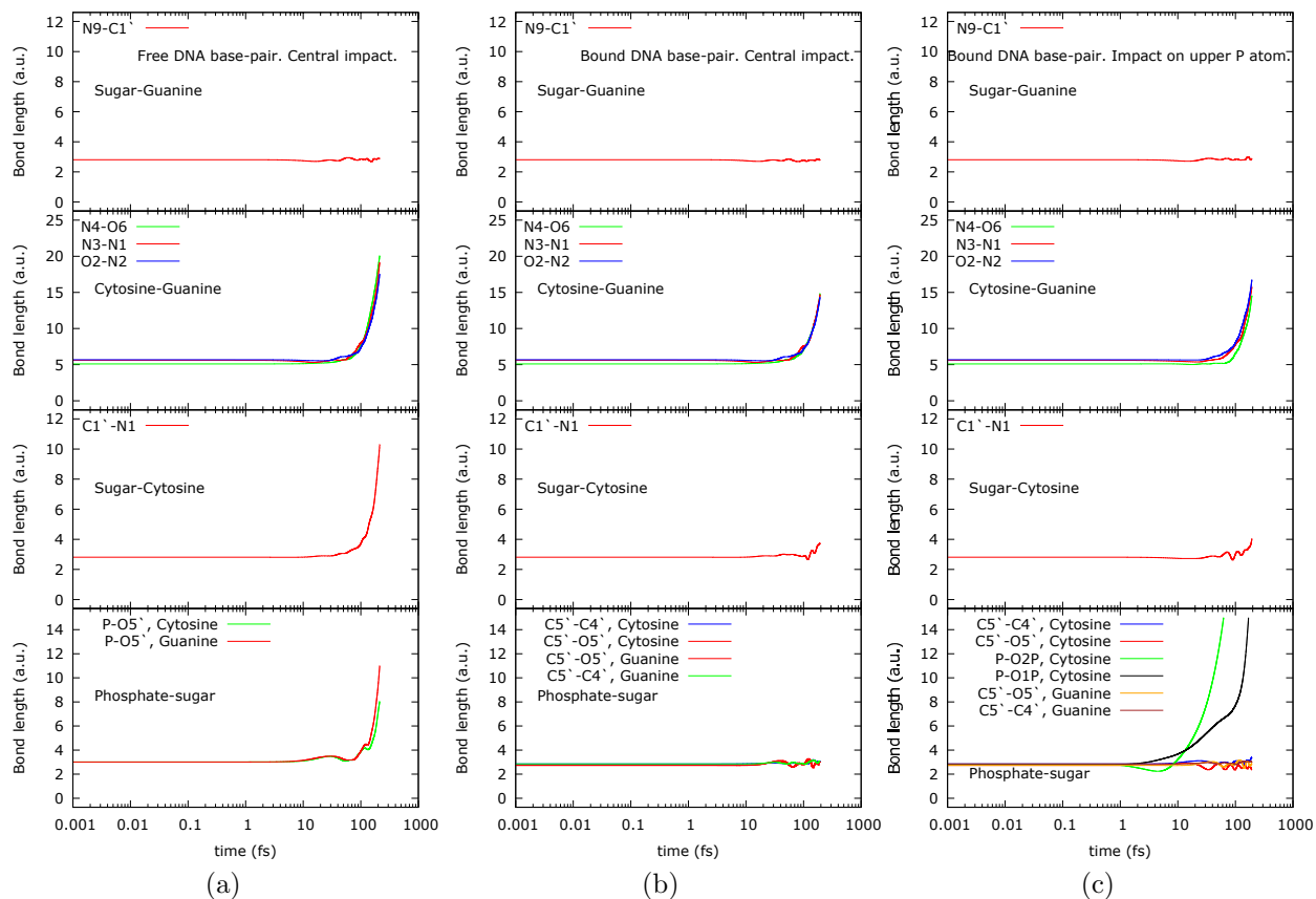
Figure 3: Length of some important DNA bonds as a function of time during and after a collision with a 4 keV proton for cases in which a) all atoms are free and the proton impacts on the bp center, b) all atoms are free except four oxygen atoms that would link the bp to their neighbors and the proton impacts on the bp center, and all atoms are free except four oxygen atoms that would link the bp to their neighbors and c) the proton impacts on one of the phosphorus atoms.
