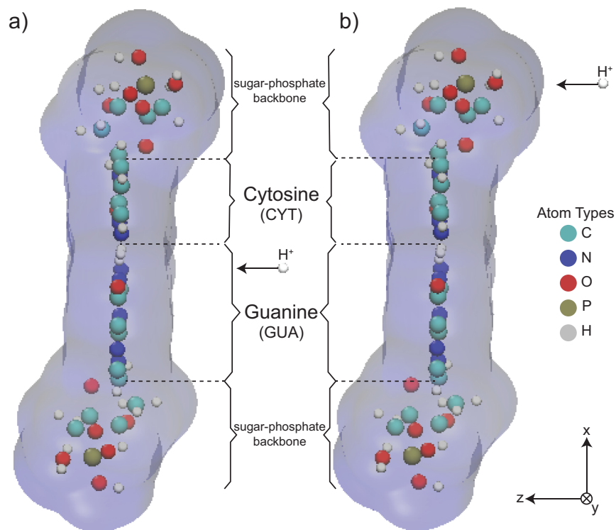
Figure 1: Proton-DNA collision setups.
