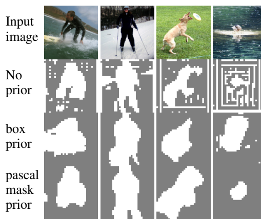
Figure 5: Effect of priors on generated masks
