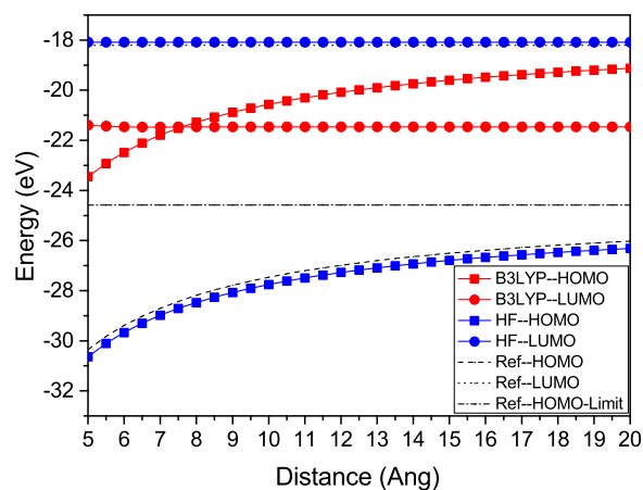
FIG. 3. HOMO and LUMO orbital energies as a function of the donor-acceptor distance for the N-2 \text{Be} \cdots \text{He} system. HF predicts the energies well with the correct HOMO-LUMO energy ordering in both short and long distances. However, B3LYP predicts an unphysical energy crossing at around 7.5 Å and therefore gives non-Aufbau results after the crossing.
