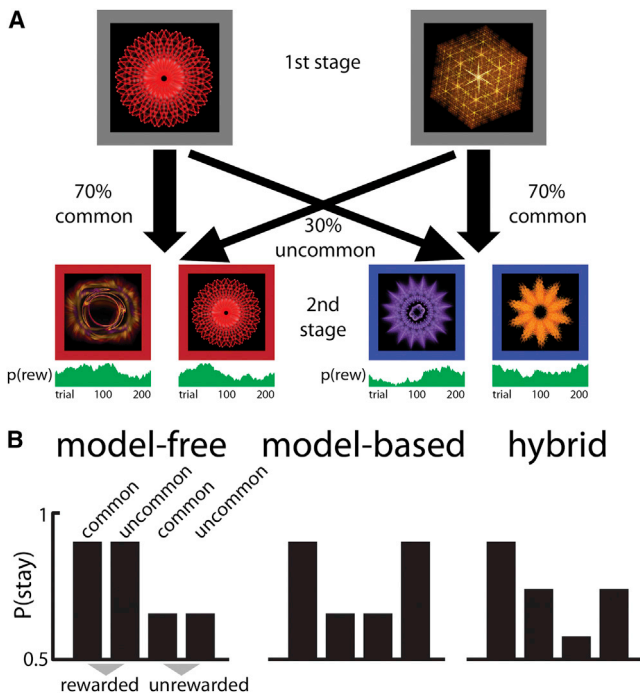
Figure 1. Task Design
