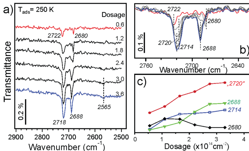
Fig. 4 (a) IRA spectra of D 2 O adsorption on Fe 3 O 4 (111) at 250 K at increasing dosage (x10 14 cm -2 ). (b) The same spectra are superimposed to highlight spectral changes. The first and the last spectra are marked in red and in blue, respectively. (c) Integral intensity (in arb. units) of the deconvoluted bands as a function of D 2 O dosage.
