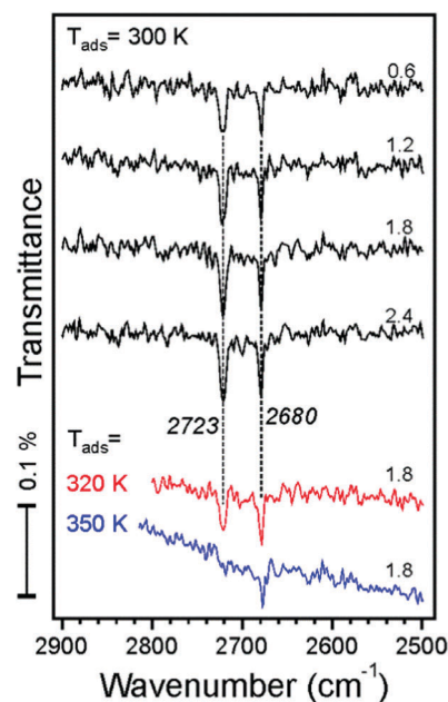
Fig. 3 IRAS spectra recorded after dosing the \text{Fe}_3\text{O}_4(111) film to \text{D}_2\text{O} molecular beam pulses (accumulative dosage ( \times 10^{14} \text{ cm}^{-2} ) is indicated). The spectra are offset for clarity.
