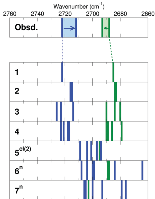
Fig. 13 Stick representation of \text{O}_w\text{D} (blue) and \text{O}_s\text{D} (green) stretching modes ( \text{cm}^{-1} ) calculated for structures shown in Fig. 9, 11 and 12 (see also Fig. S4 in the ESI.†). Note that all calculated wavenumbers are red-shifted by 14 \text{ cm}^{-1} in order to facilitate the comparison with the experimental results shown on top panel. Original numbers are presented in Table S1 in the ESI.†
