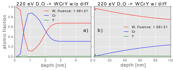
Figure 8: Simulated WCrY depth-resolved target composition after a fluence of 1 \cdot 10^{21} D ions/cm 2 without (a) and including diffusion (b)
