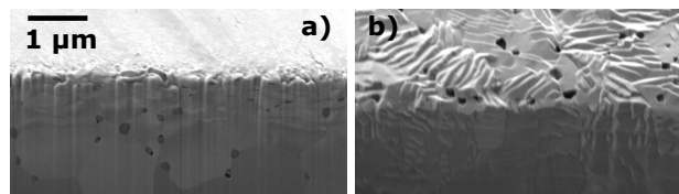
Figure 4: SEM picture of upper edge of FIB cut for SA11 before (a) and after plasma exposure (b)
