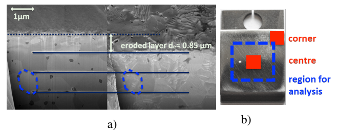
Figure 2: a) comparison of FIB marker positions relative to the surface before and after plasma for sample SA21, b) sample geometry for smart alloys with centre and corner positions for FIB craters
