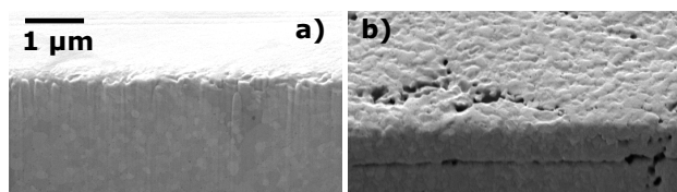
Figure 7: SEM picture of upper edge of FIB cut for SA22 before (a) and after plasma exposure (b)
