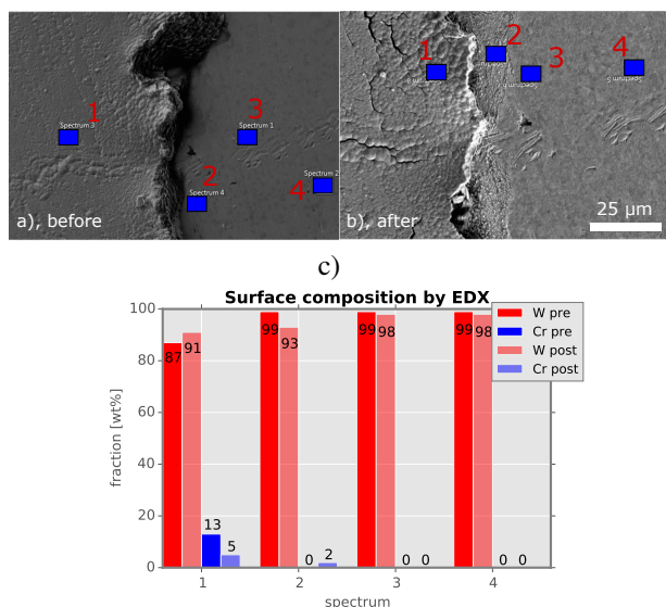
Figure 6: EDX spectra on coated W24 sample a) before and b) after plasma. Left side of sample with spectrum 1: deposited WCrY, c): EDX spectra 1-4: surface composition of W and Cr in wt%, not displayed O- and C-content add up to 100 wt%
