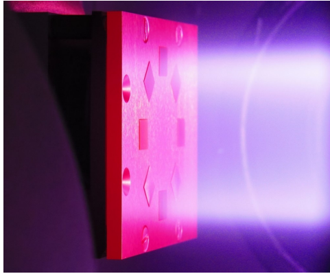
Figure 1: Plasma exposure of WCrY and W samples in PSI-2
