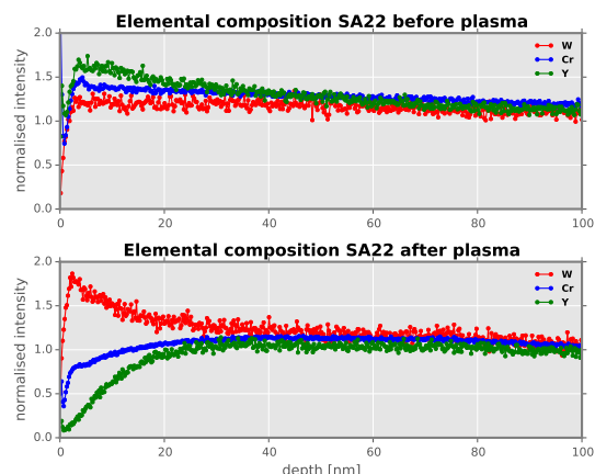
Figure 5: SIMS-analysis for W, Cr and Y in PE2
