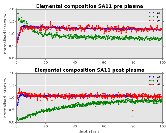
Figure 3: SIMS-analysis for W, Cr and Y in PE1
