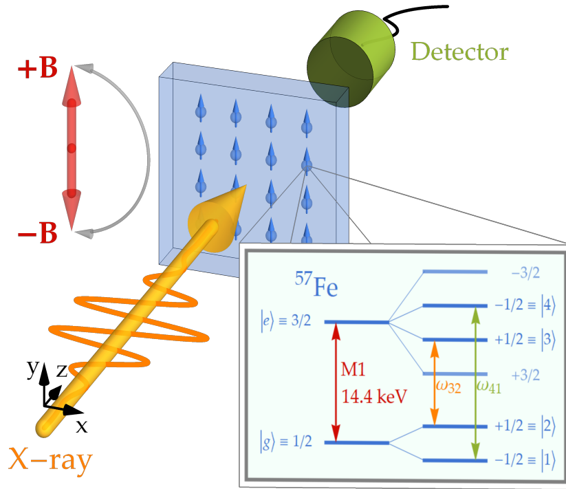
Figure 1. NFS setup. The x-ray (orange line and arrow) propagating along the z -direction impinges on the Mössbauer target. The probe experiences a magnetic field \mathbf{B} , that can be switched off, retrieved and can be rotated by \pi , inverting the quantization axis. The inset shows the level scheme of the ground g and first excited e state of the ^{57}\text{Fe} sample including the magnetic sublevels.
