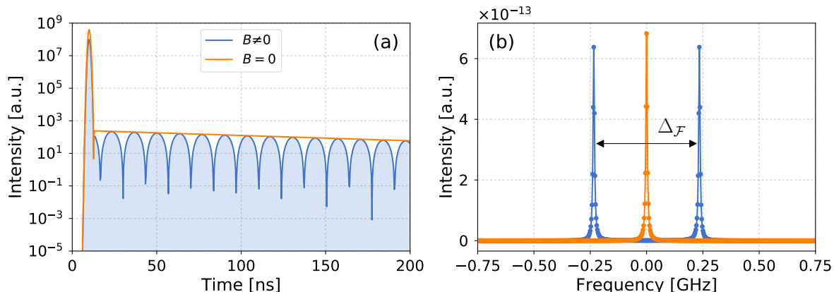
Figure 2. (a) Time spectrum for a constant magnetic field and optical thickness \xi = 0.5 (blue line) and in the absence of any hyperfine magnetic field with \xi = 0.25 (orange line). The peak at t = 10 ns shows the incoming Gaussian pulse. The magnetic field introduces an absolute-cosine-like oscillation known as quantum beat. (b) Corresponding frequency spectrum. In the absence of the magnetic field, the spectrum consists of a single peak at the nuclear transition frequency \omega_0 . The magnetic field introduces the splitting into the two transition frequencies \omega_{41} and \omega_{32} separated by \Delta_{\mathcal{F}} .
