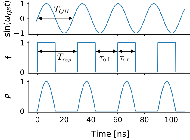
Figure 7. Basic components of the analytical model. The combination of the sinusoidal signal \sin(\omega_{QB}t) given via the quantum beat and the periodic sequence f determined by the B-field switching leads to the periodic function P .
