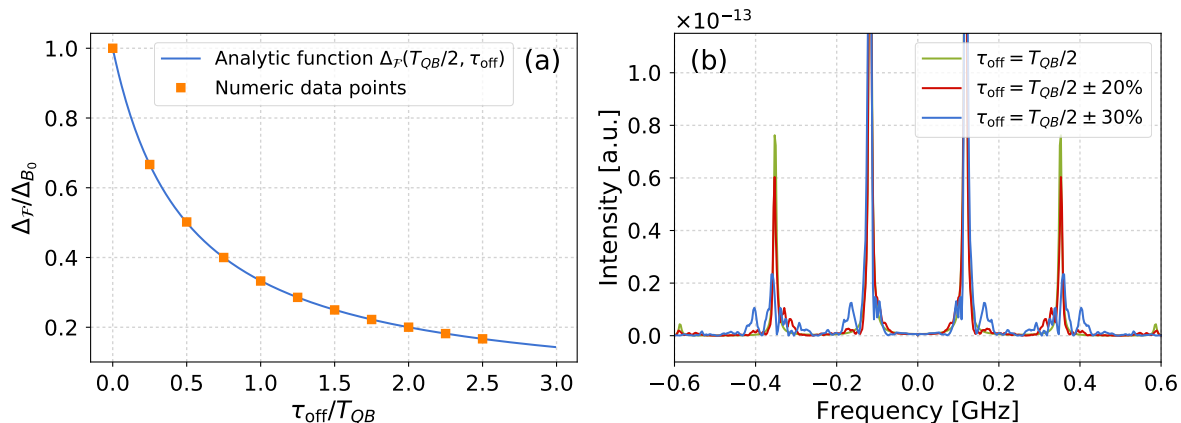
Figure 8. (a) Peak distance \Delta_{\mathcal{F}} as a function of the storage time \tau_{\text{off}} . Numeric data points are shown together with the analytic solution given by Eq. (13). (b) Frequency spectra for regular stepwise switching schemes with random variations in \tau_{\text{off}} . For both graphs \tau_{\text{on}} = T_{QB}/2 and \xi = 0.5 have been considered.
