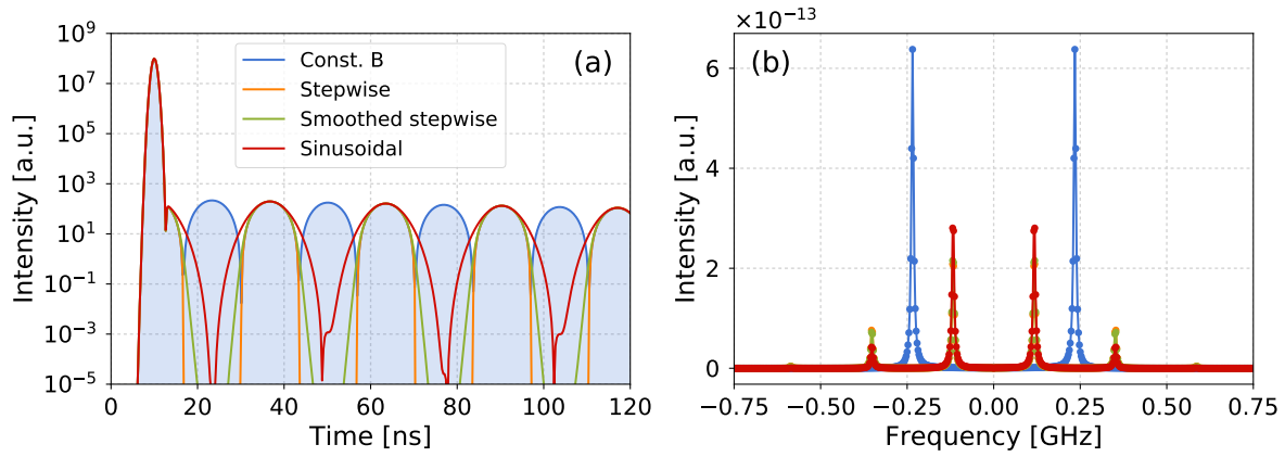
Figure 10. (a) Time and corresponding frequency spectra (b) for abrupt (orange line), smoothed (green line) and sinusoidal (red line) magnetic switching sequences in comparison to the case of a constant magnetic field (blue line). The smoothing radius for the exponential step was set to \varepsilon = 0.5 ns. For all cases we considered \tau_{\text{on}} = \tau_{\text{off}} = T_{QB}/2 and \xi = 0.5 .
