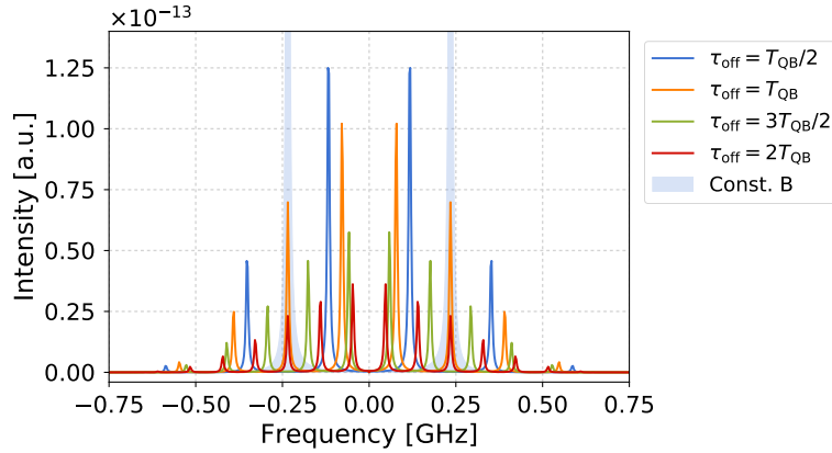
Figure 4. Frequency spectra for different \tau_{\text{off}} values and constant \tau_{\text{on}} = T_{QB}/2 . With increasing storage time, the peaks multiply and narrow towards \omega_0 while the overall intensity drops. For illustration purposes, the spectrum for \tau_{\text{off}} = T_{QB}/2 was manually downscaled by 40%.
