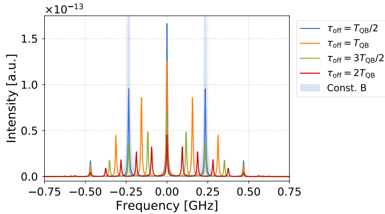
Figure 6. Frequency spectra in the case of the inverted stepwise switching scheme for several storage times \tau_{\text{off}} and constant \tau_{\text{on}} = T_{QB}/2 . For illustration purposes, the spectrum for \tau_{\text{off}} = T_{QB}/2 was manually downscaled by 40%.
