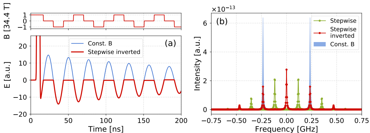
Figure 5. (a) \mathbf{E} -field amplitude time spectrum for the inverting sequence at \tau_{\text{on}} = \tau_{\text{off}} = T_{QB}/2 . The magnetic field orientation is inverted after every storage. (b) Comparison of the frequency spectra of the inverting and regular stepwise switching for the same choice of \tau_{\text{on}} and \tau_{\text{off}} .
