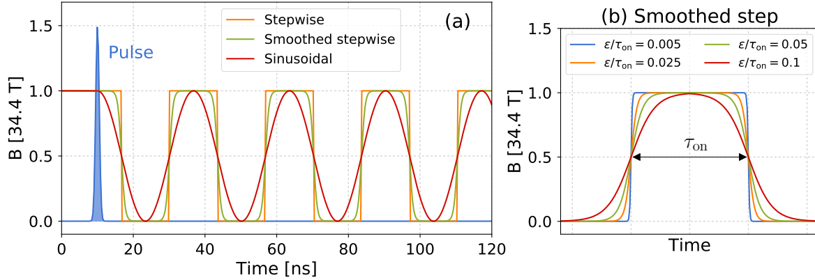
Figure 9. (a) Magnetic field modulations: stepwise (orange line), smoothed stepwise (green line) and sinusoidal (red line). (b) Examples of smoothed stepwise functions with several \varepsilon values.
