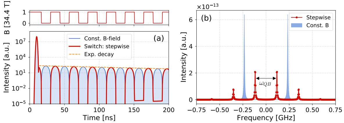
Figure 3. (a) Time and (b) frequency spectra for \tau_{\text{on}} = \tau_{\text{off}} = \frac{T_{QB}}{2} (red line). The periodically manipulated scattered field intensity is presented together with the case of a constant magnetic field B_0 = 34.4 T (blue line). For the computations an optical thickness of \xi = 0.5 was used.
