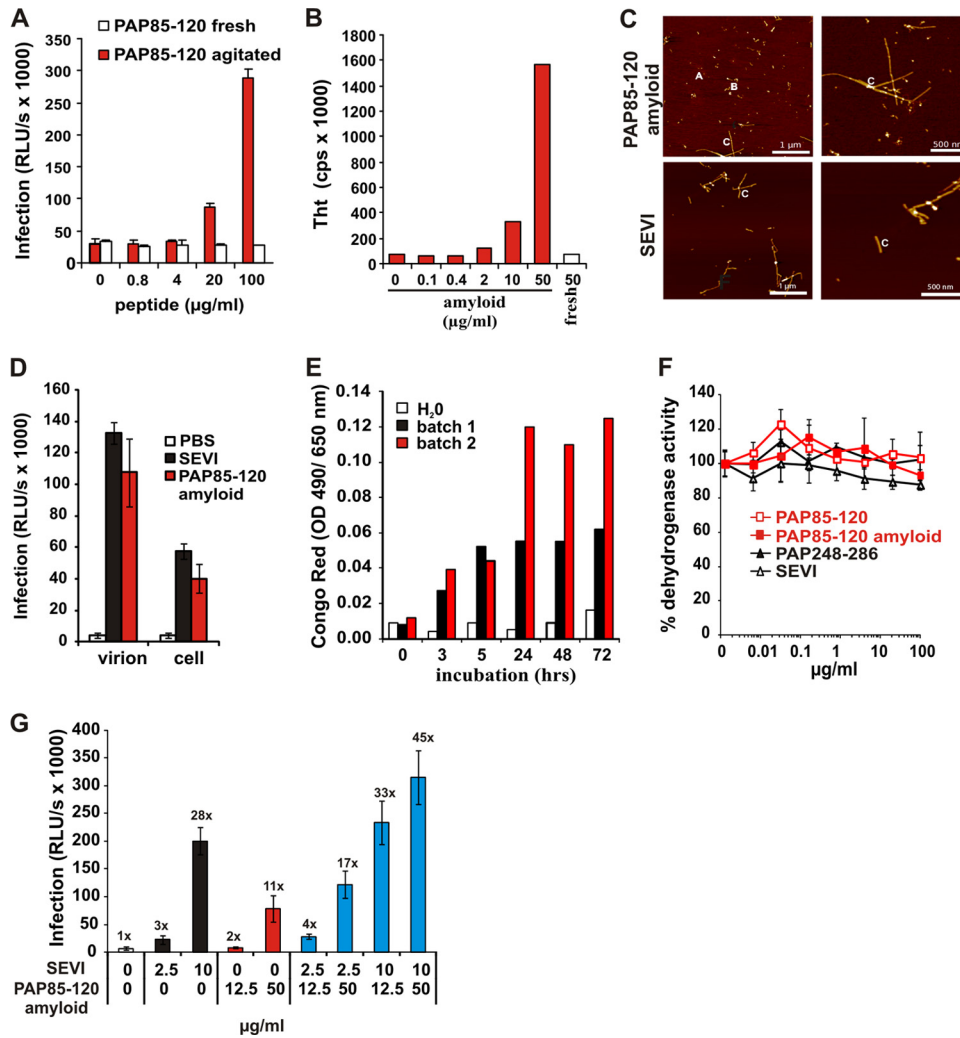
FIG 2 PAP85-120 forms amyloid and enhances HIV infection. (A) Only agitated PAP85-120 boosts HIV-1 infection of TZM-bl cells. All infection experiments in Fig. 2 to 4 were performed in triplicate, and values shown are average values \pm standard deviations. (B) Agitated PAP85-120 forms amyloid as assessed by fluorescence in the presence of Thioflavin T (ThT) (10). (C) AFM images of PAP85-120 and SEVI amyloid (0.05 \mu\text{g/ml} ) deposited on mica; images were obtained using a Nanoscope IIIa AFM (Digital Instruments) using silicon cantilevers (Omicron; spring constant, 2 N/m). A, oligomeric particles; B, protofibrils; C, mature fibrils (5, 6). (D) PAP85-120 amyloid promotes HIV-1 infection of TZM-bl cells following virion or target cell pretreatment. The final cell culture concentration of PAP85-120 amyloid was 10 \mu\text{g/ml} . (E) Fibril formation kinetics of two batches of PAP85-120 (5 \mu\text{g/ml} , 200 \mu\text{l} ; agitation at 1,200 rpm). At the indicated time points, aliquots were taken and amyloid formation was quantified in a Congo red-based amyloid staining assay (10). (F) PAP-derived amyloid does not diminish cell viability. PBMCs were incubated for 3 days with the indicated PAP preparations, and cell viability was measured in an MTT (3-[4,5-dimethyl-2-thiazolyl]-2,5-diphenyl-2H-tetrazolium bromide) assay (10). (G) Additive HIV enhancing effects of fibrillar PAP fragments. TZM-bl cells were infected with HIV-1 incubated with the indicated PAP fibrils alone or in combination.
