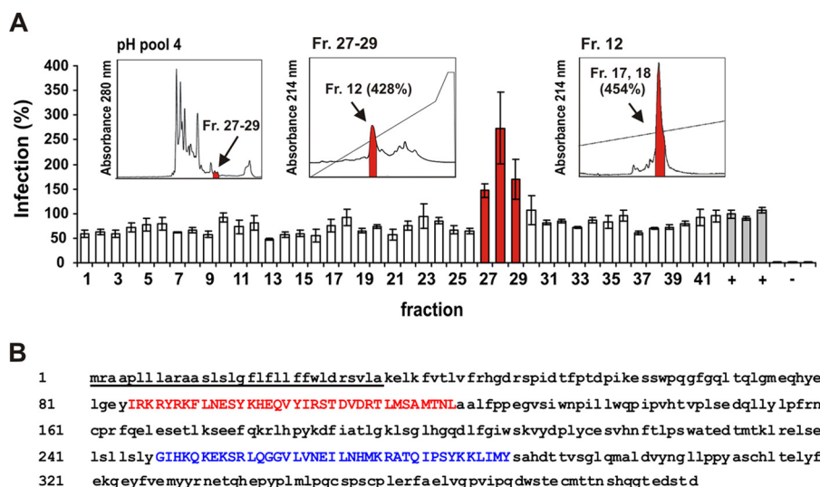
FIG 1 Purification of a second fibril-forming PAP fragment that enhances HIV-1 infection from semen. (A) Fractions 27 to 29 of pH pool 4 (red) promote HIV-1 infection of TZM-bl cells. The insets show the high-performance liquid chromatography results of pH pool 4 (left) and of the active fractions 12 (middle) and 17/18 (right) obtained after the different purification steps. Fractions 17 and 18 used for peptide sequencing are shown in red. +, no peptide added; −, uninfected cells. (B) Amino acid sequence of PAP, with the signal peptide underlined, residues 85 to 120 in red, and residues 248 to 286 in blue.
