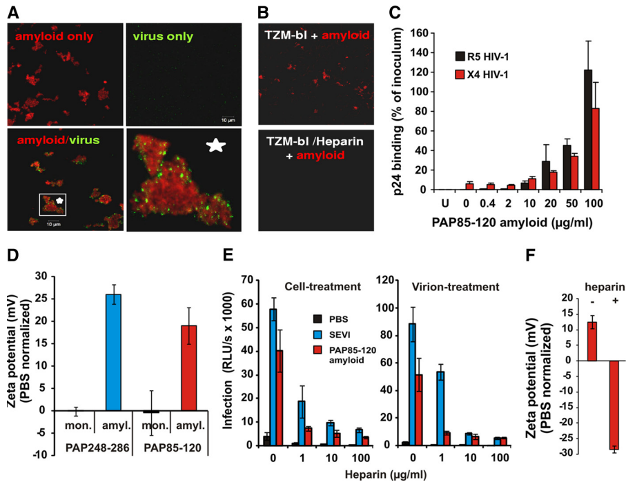
FIG 4 The cationic properties of PAP85-120 fibrils are essential for their ability to enhance HIV infection. (A) PAP85-120 amyloid captures virus. Confocal images of PAP85-120 amyloid stained with a fluorescent dye, YFP-tagged HIV-1, and a mixture of amyloid and virus. The panel with a star indicates a magnified image of the amyloid/virus complexes. (B) PAP85-120 amyloid binds TZM-bl cells in a manner that can be blocked by polyanions. Stained amyloid (50 µg/ml) was added to cells in the presence or absence of heparin (100 µg/ml), and cells were washed 30 min later, and imaged by fluorescence microscopy. (C) Fibrils increase virion attachment. X4- and R5-tropic HIV-1 virions were treated with PAP85-120 fibrils and added to TZM-bl cells. One hour later, cells were washed, and cell-associated p24 was quantified by ELISA. Shown are the percentages of the total quantity of p24 present in the viral inoculum. (D) Zeta potential measurements of monomeric and fibrillar PAP fragments. (E) Polyanions abrogate infectivity enhancement. Heparin was added to cells that were subsequently infected with SEVI or PAP85-120 amyloid (50 µg/ml) treated virus (cell-treatment). Alternatively, cells were infected with virus pretreated with amyloid in the presence of the indicated amounts of heparin (virion-treatment). (F) PAP85-120 amyloid binds heparin. Fibrils (100 µg/ml) were mixed with PBS or heparin (100 µg/ml) and centrifuged for 10 min at 14,000 rpm. The pellets were resuspended in PBS, and zeta potentials were measured.
