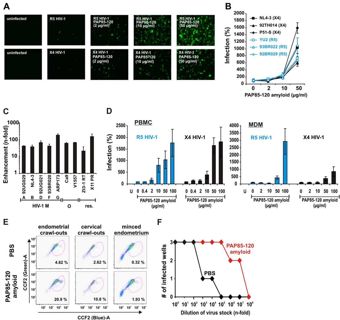
FIG 3 Fibrillar PAP85-120 enhances R5- and X4-tropic HIV-1 infection of cell lines and primary target cells (10, 12). (A) UV-microscopy images taken 3 days postinfection of CEM-M7 with PAP85-120 amyloid-treated X4- and R5-tropic virus (12). (B and C) TZM-bl cells were infected with various X4- and R5-tropic HIV-1 NL4-3 V3 recombinants (12) treated with various concentrations of PAP85-120 fibrils (B) or primary HIV-1 isolates and drug-resistant virus (10) treated with 50 µg/ml of PAP85-120 fibrils (C). (D) PAP85-120 amyloid enhances infection of interleukin-2/phytohemagglutinin-stimulated PBMCs (left) and monocyte-derived macrophages (MDM) (right) by luciferase-encoding HIV-1 (10). Concentrations shown are those of PAP85-120 amyloid during virion preincubation. (E) The fibrils (31.35 µg/ml) boost fusion of HIV-1 to CD4 + T cells purified from endometrial biopsies. These cells were isolated by allowing T cells to “crawl out” of endometrial biopsies (13) or by positive selection from minced tissue (“minced endometrium”). Percent values give fusion rates in the absence and presence of amyloid fibrils. (F) Limiting dilution analysis of HIV-1. CEM-M7 cells were infected in triplicates with 10-fold dilutions of R5-tropic HIV-1 virus stock in the absence or presence of PAP85-120 fibrils (50 µg/ml). Shown are the numbers of infected cultures 7 days postinfection as determined by UV-microscopy.
