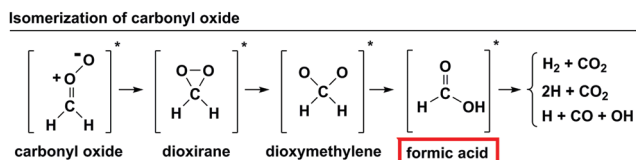
Scheme 3 Isomerization of the simplest Criegee intermediate, carbonyl oxide, to formic acid.
