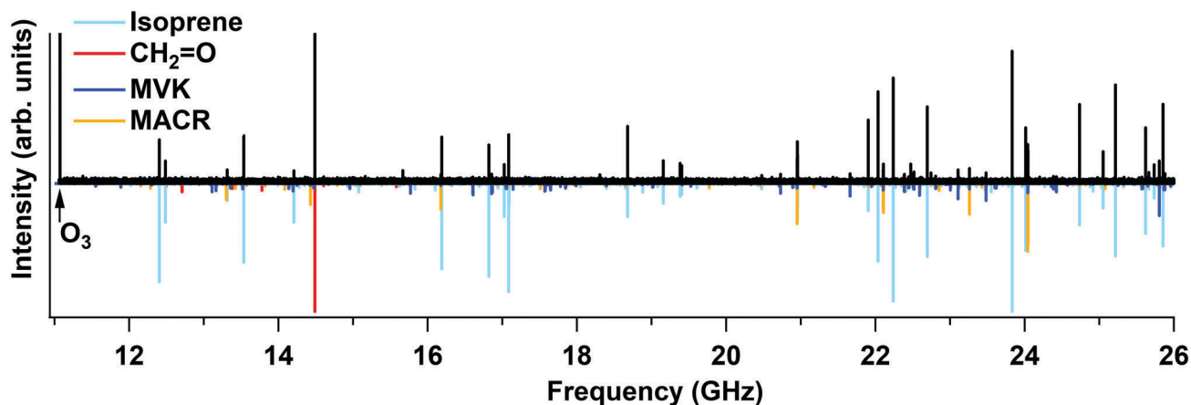
Fig. 2 The 12–26 GHz CP-FTMW spectrum of the ozonolysis of isoprene. The reactant ratio is 2 : 1 \text{O}_3 to isoprene, and the total reagent concentration is 2% in argon. Authentic samples of isoprene, \text{CH}_2=\text{O} , MVK and MACR are displayed along the negative y -axis for reference.
