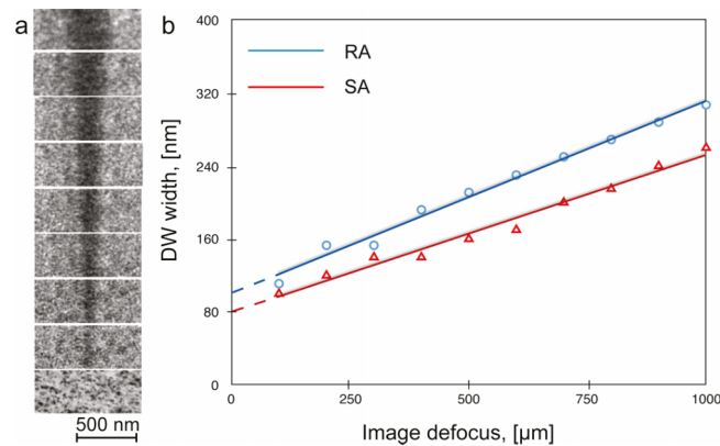
FIG. 4. (a) Fresnel defocus images of a 180^\circ DW in the SA FeSiNbCuB sample. The defocus difference between successive images is 100 \mu\text{m} . (b) FWHM values of divergent DWs measured from defocus series recorded from the RA and SA FeSiNbCu samples.
