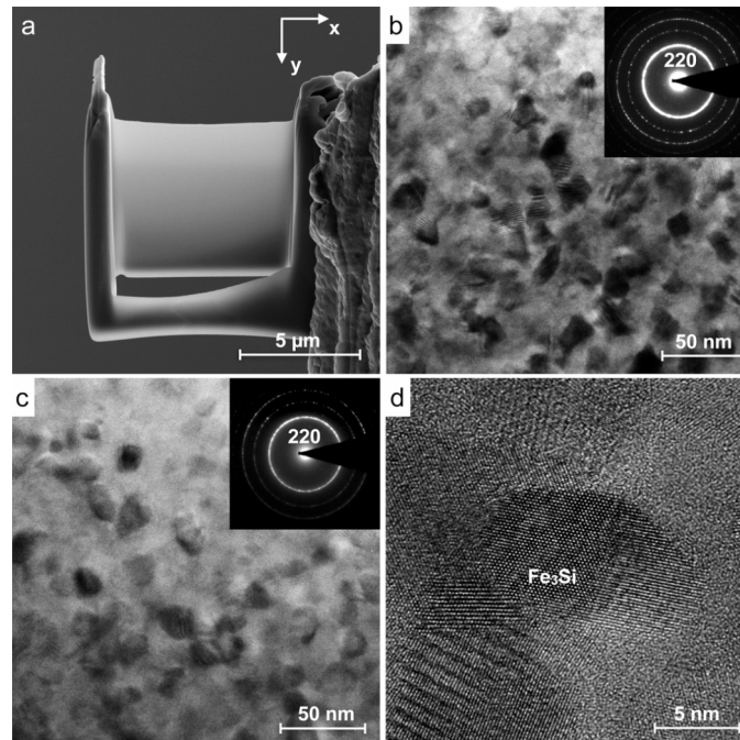
FIG. 1. (a) SEM image of a TEM specimen of SA FeSiBNbCu. The stress was applied along the x direction. (b, c) BF TEM images and SAED patterns of the RA and SA samples, which have random polycrystalline structures. (d) High-resolution TEM image of Fe 3 Si grains in an amorphous Nb- and B-rich matrix. The average grain size is ~10 nm.
