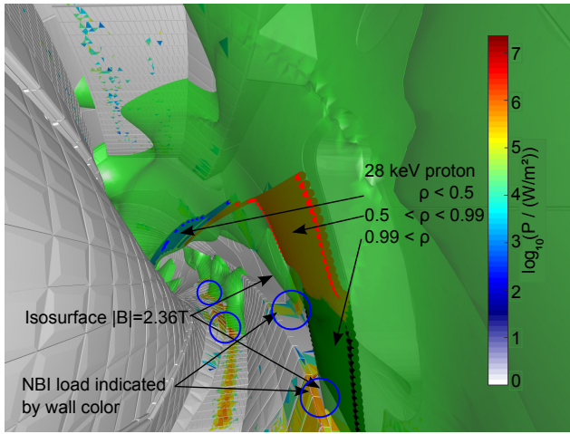
Figure 1. Perspective view into the plasma vessel illustrating the main wall load mechanism. The wall color indicates the wall load from the NBI ions in logarithmic scale. A |B| isosurface is drawn in translucent green to illustrate the local magnetic wells due to the modular coils. Fast ions trapped in such wells drift quickly to the wall due to the gradient-B drift ( \nabla B \times B ). This is illustrated by following a 28 keV proton collisionlessly while omitting the radial electric field. The proton trajectory is colored according to the minor radius ( \rho , square root of the normalized toroidal flux) of the path. The |B| isosurface value is chosen to match the reflection magnetic field ( E/\mu ) of the ion, 2.36 T. Hence, the ion is toroidally reflected at the isosurface and remains in the well and finally drifts to the wall. Similarly, most of the hot spots on the wall are located where the wall intersects the wells (blue circles). The simulation is for the reversed field W7-X standard configuration \langle\beta\rangle = 2\% . Here the ions drift downwards, while in a forward field case the hot spots would be located at the stellarator symmetric [10] top intersection areas.
